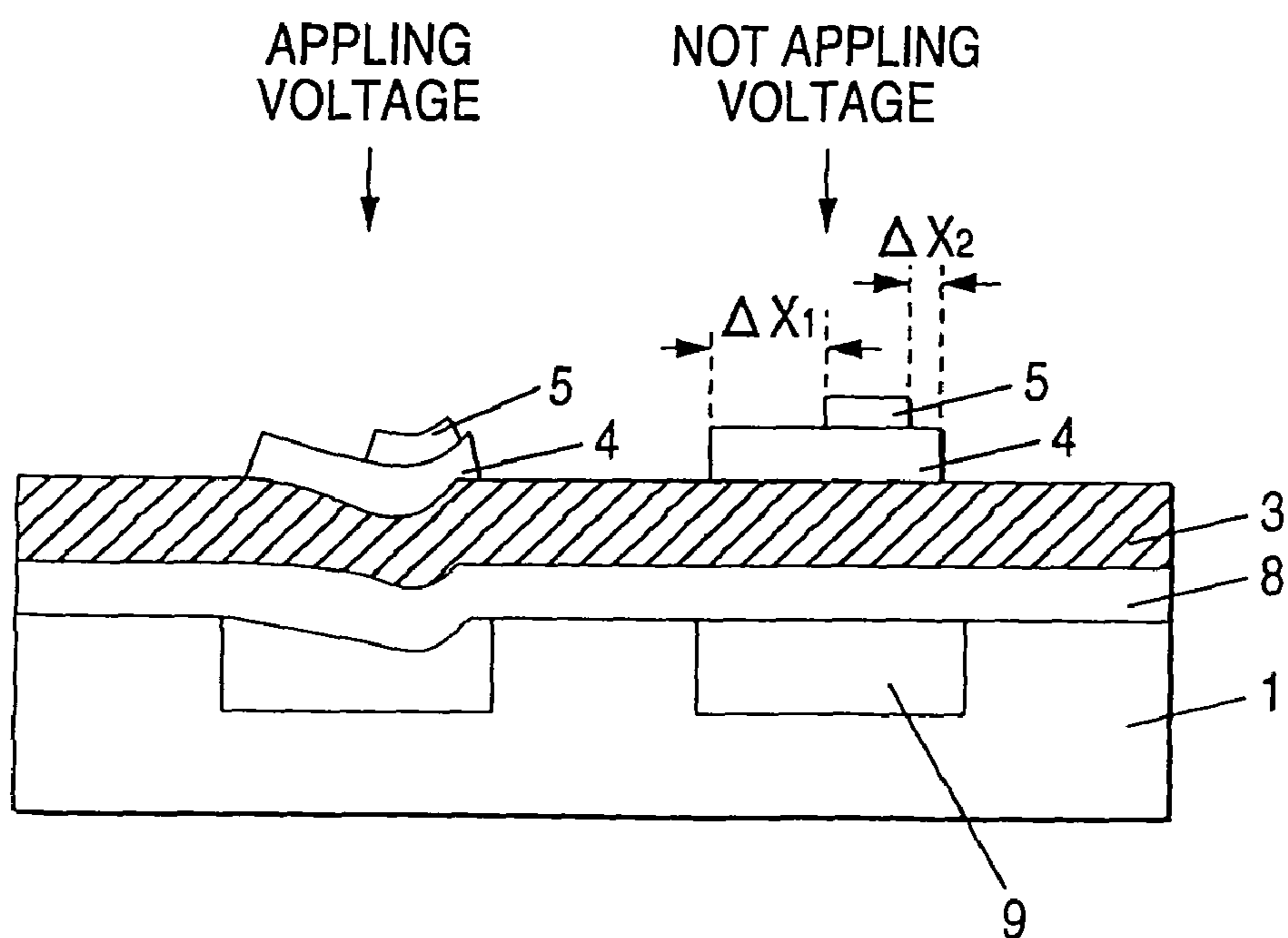
FIG. 43 PRIOR ART
