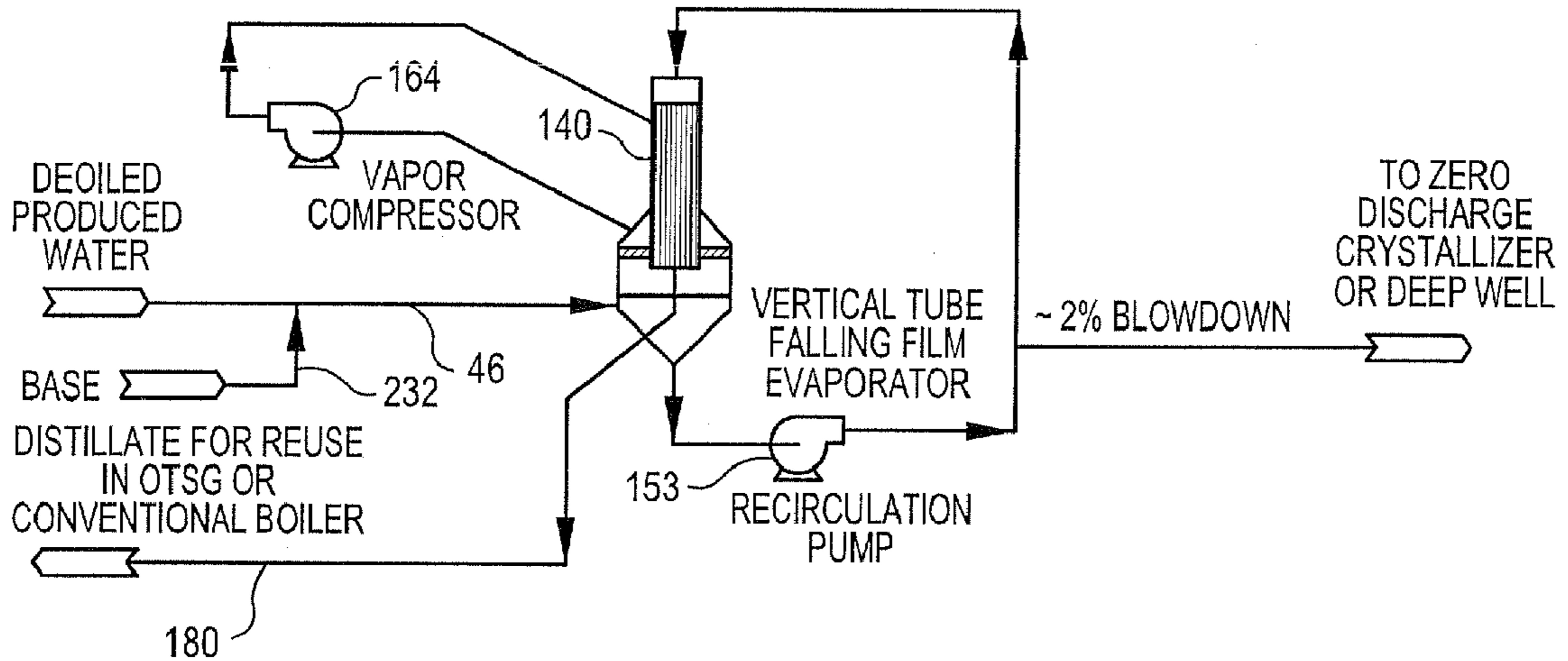
SIMPLIFIED VAPOR COMPRESSION FALLING FILM EVAPORATOR SYSTEM
