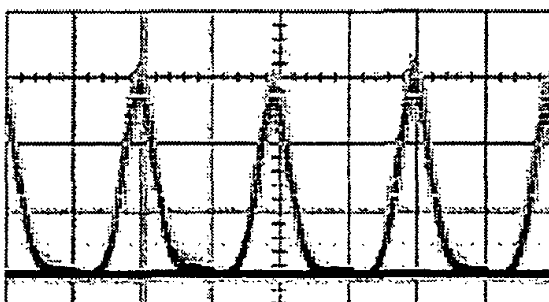
\lambda_s = 1560 nm
