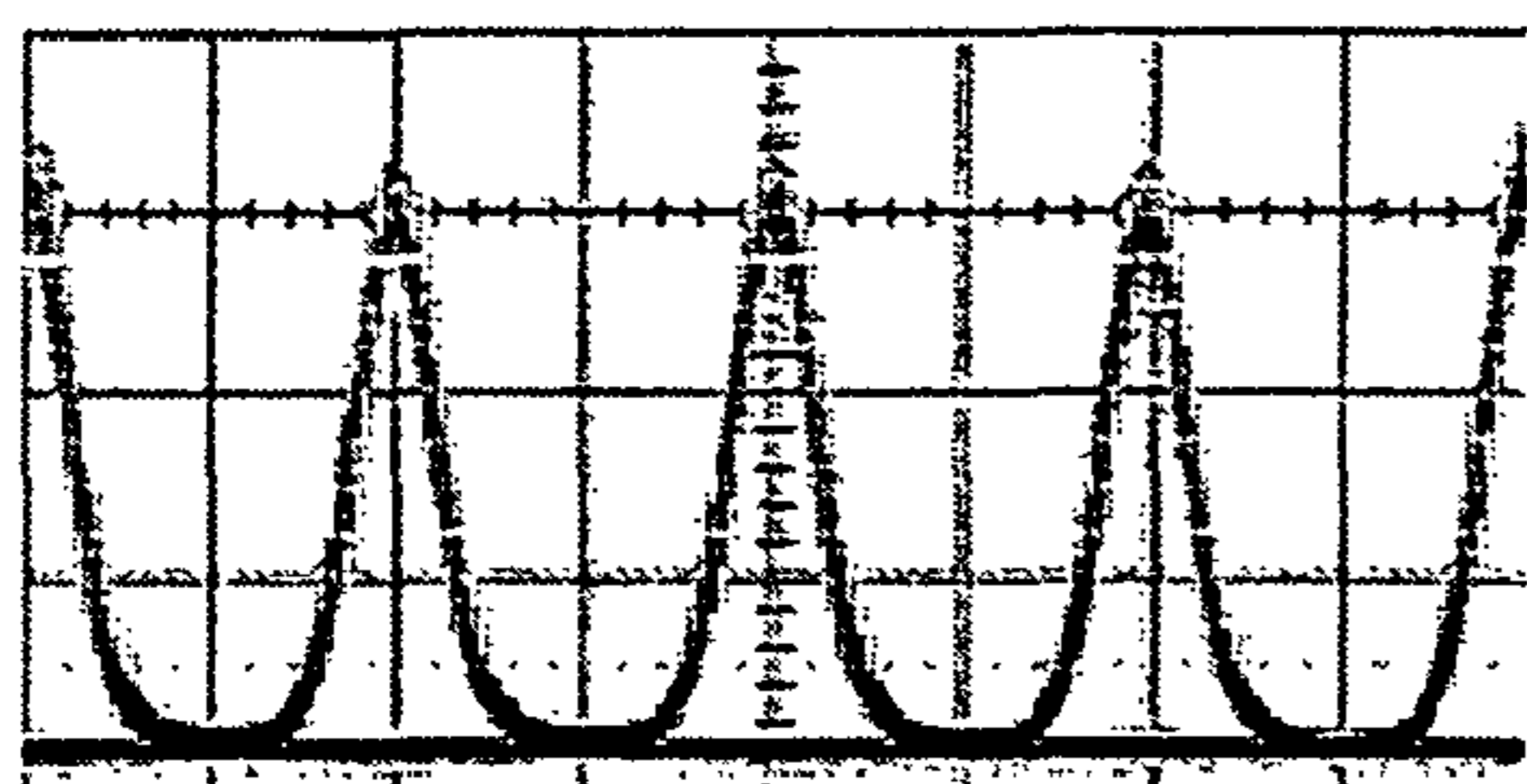
160 Gb/s ( \lambda_s = 1540 nm)
