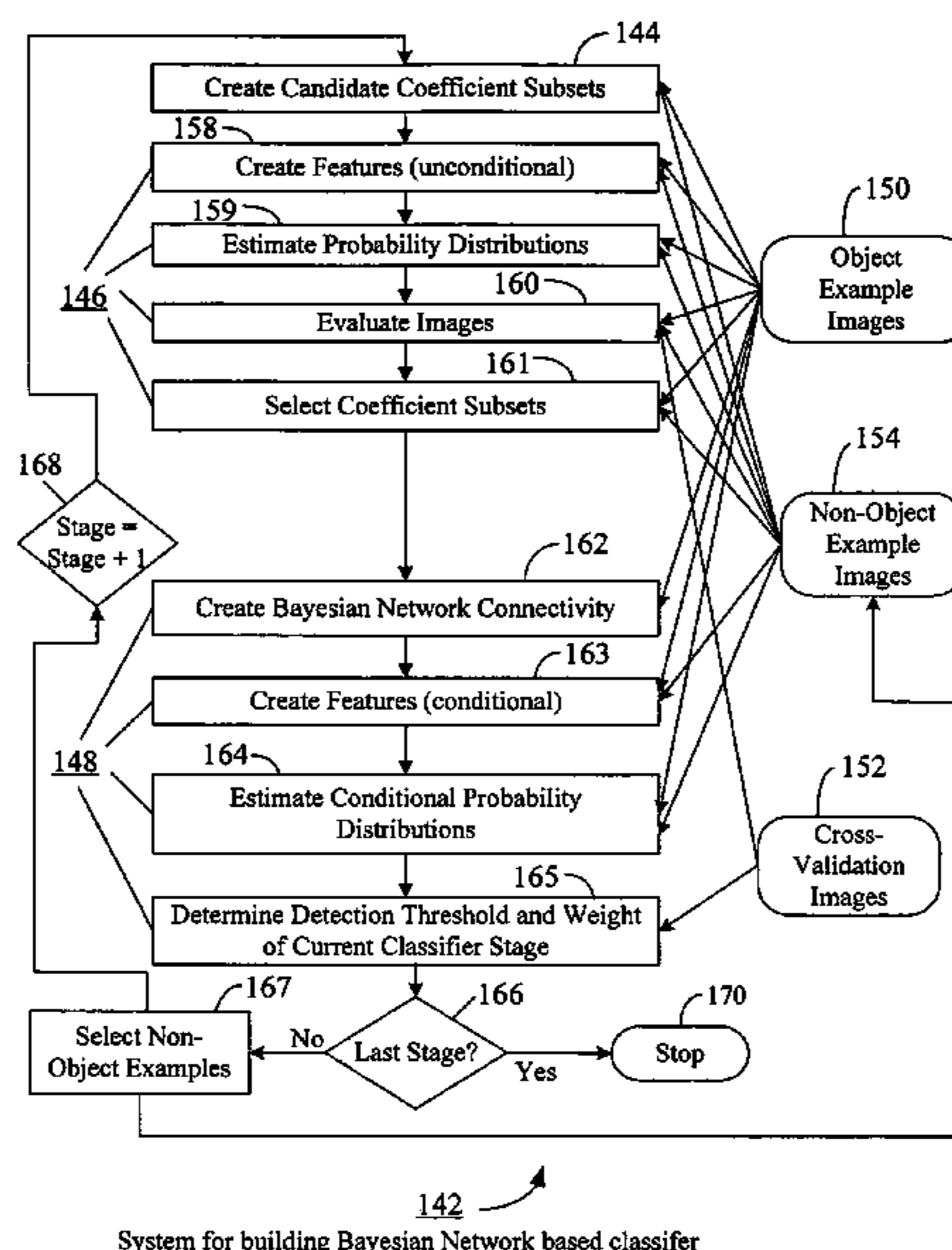
142 System for building Bayesian Network based classifier
