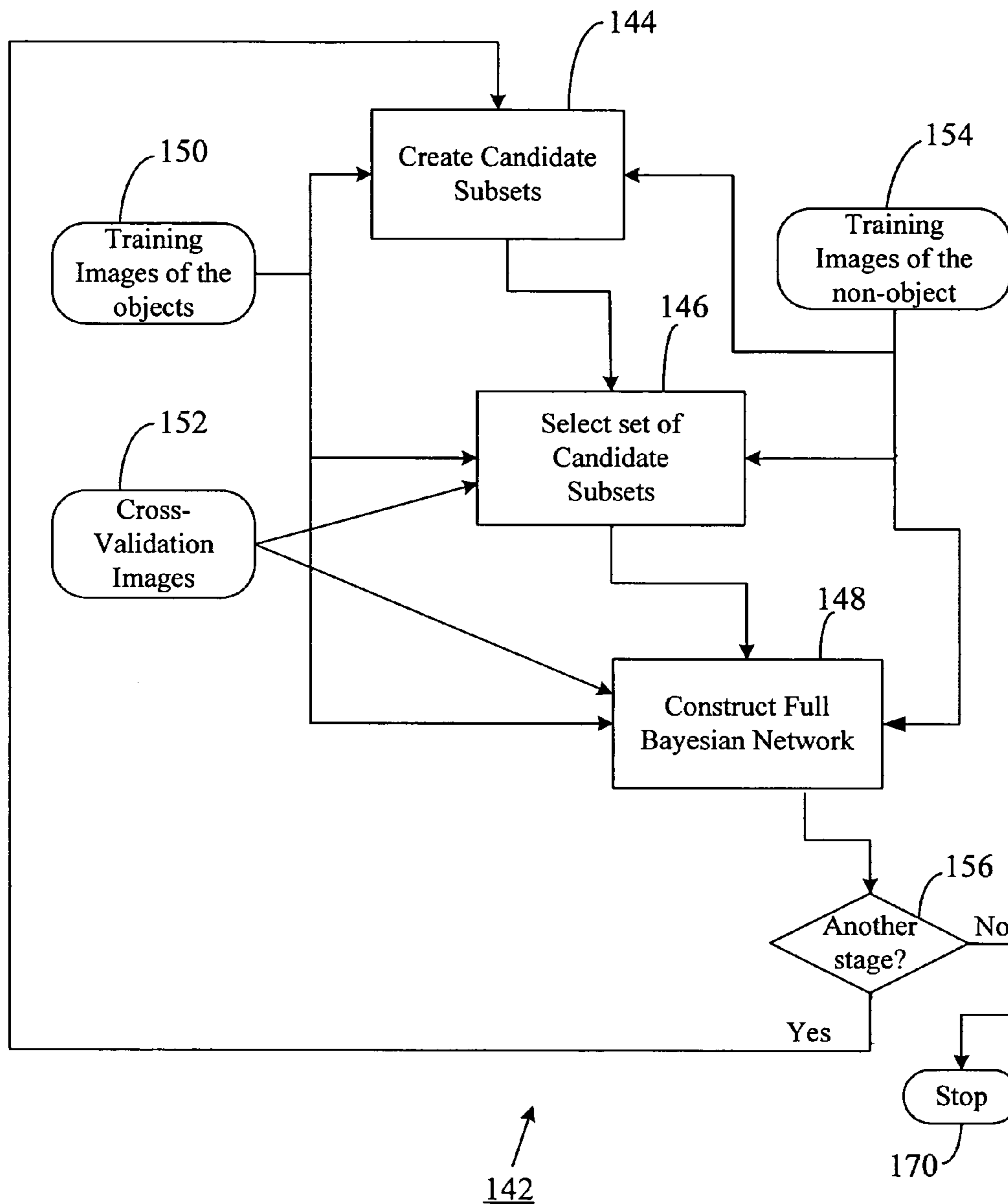
System for Creation of Bayesian Network Classifier
