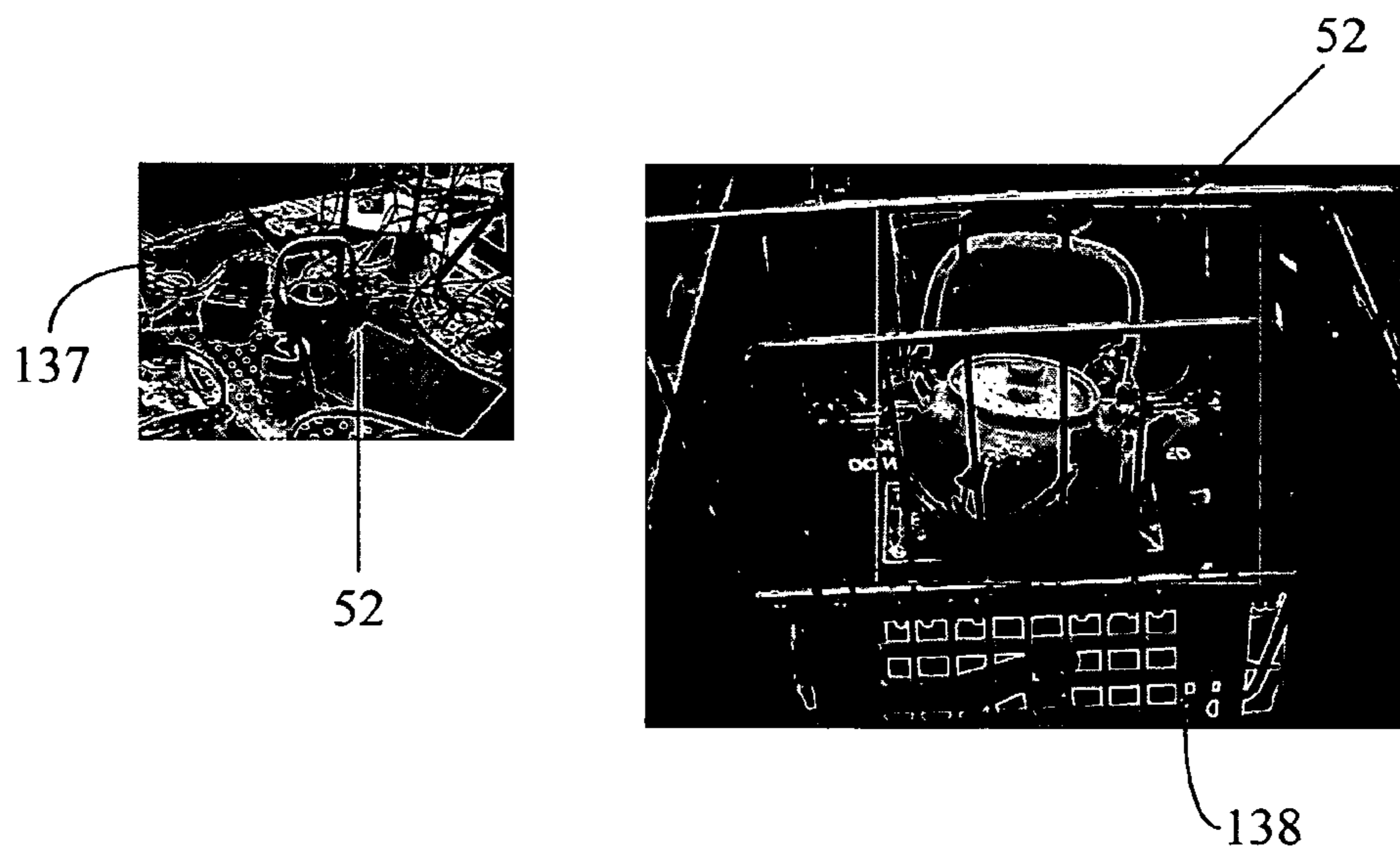
FIG. 32 Teapot Detection
