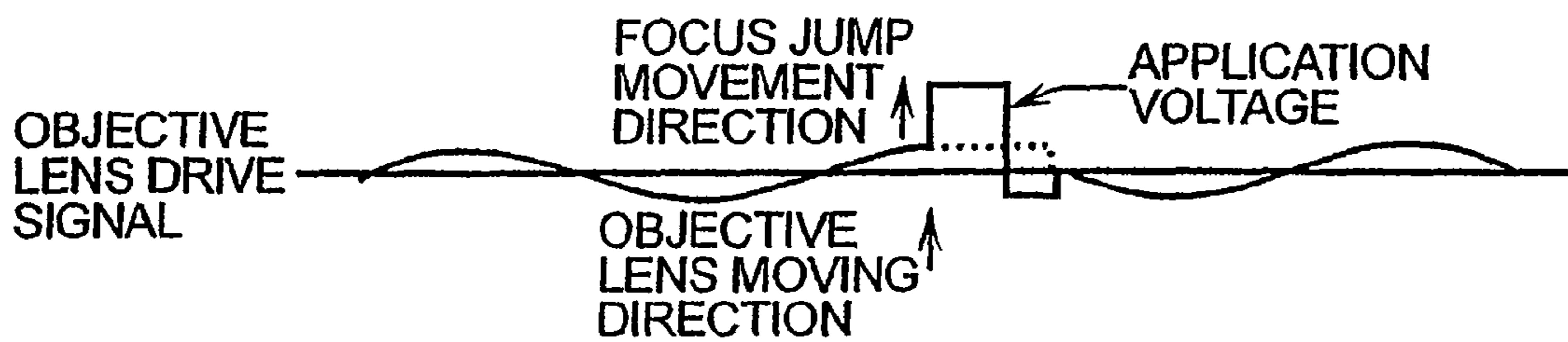
Fig. 4 (b) CASE WHERE A VOLTAGE IS APPLIED TO A PEAK OF A SURFACE VIBRATION COMPONENT (Prior Art)
