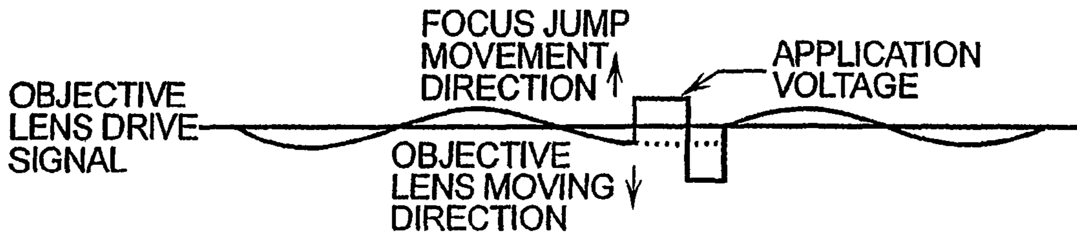
Fig. 4 (a) CASE WHERE A VOLTAGE IS APPLIED TO A VALLEY OF A SURFACE VIBRATION COMPONENT (Prior Art)
