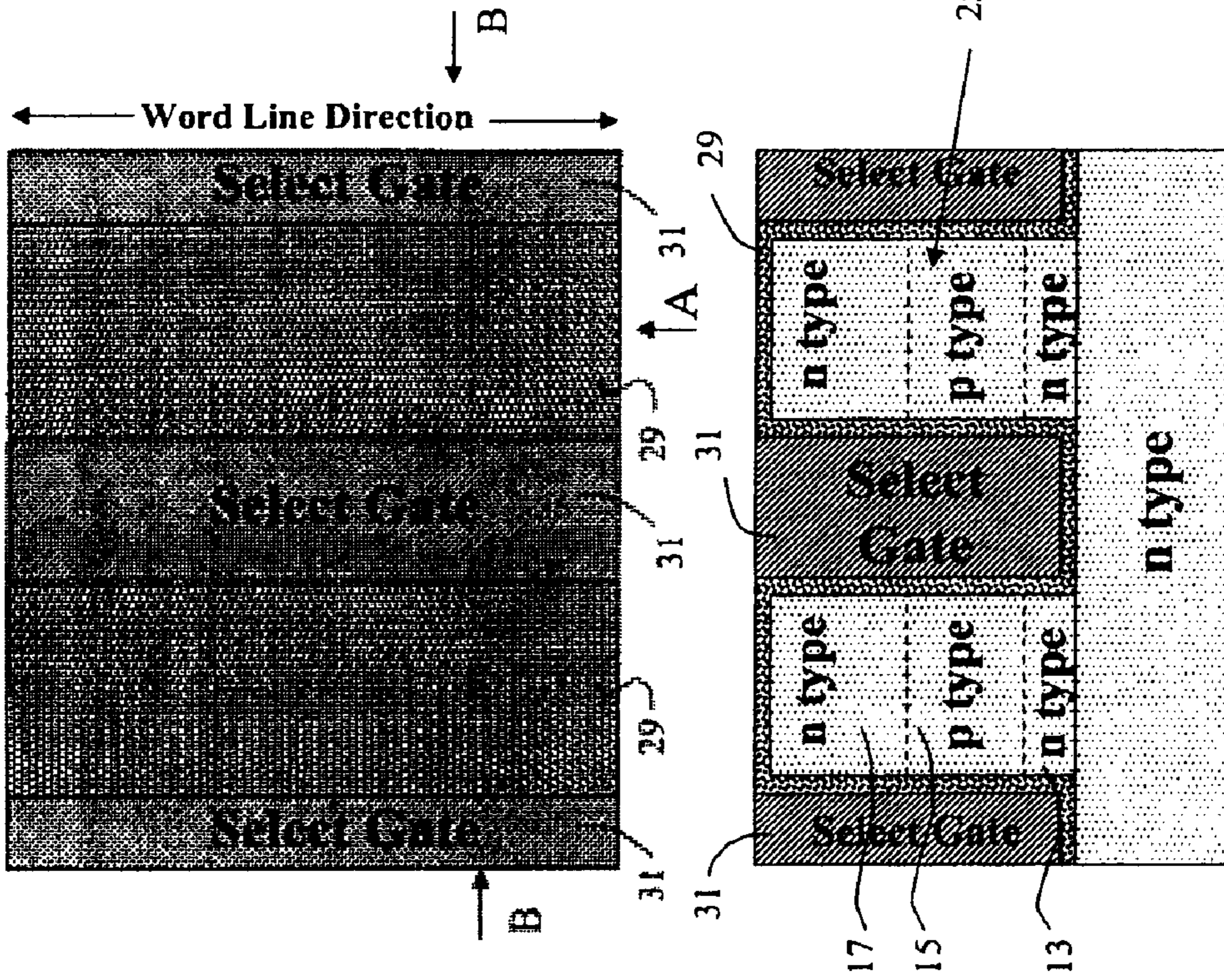
FIGURE 7A Bit Line Direction Word Line Direction
