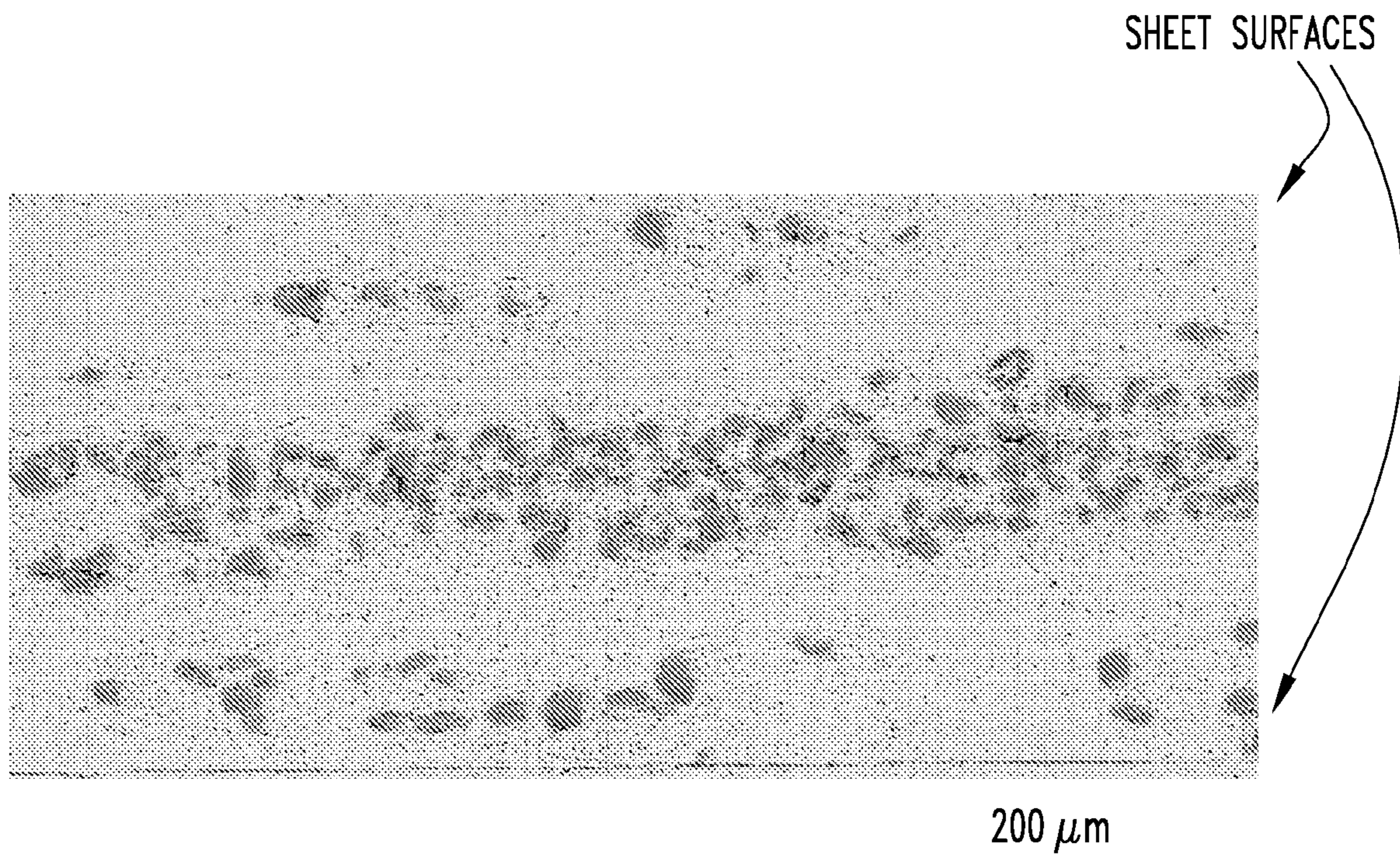
FUNCTIONALLY GRADED MMC STRIP – METALLIC OUTER LAYERS FOR GOOD FORMABILITY, MMC CENTER FOR IMPROVED RIGIDITY (Al-15 VOLUME % Al_2O_3 COMPOSITE IN ROLLED CONDITION AT 0.2 mm THICKNESS)
