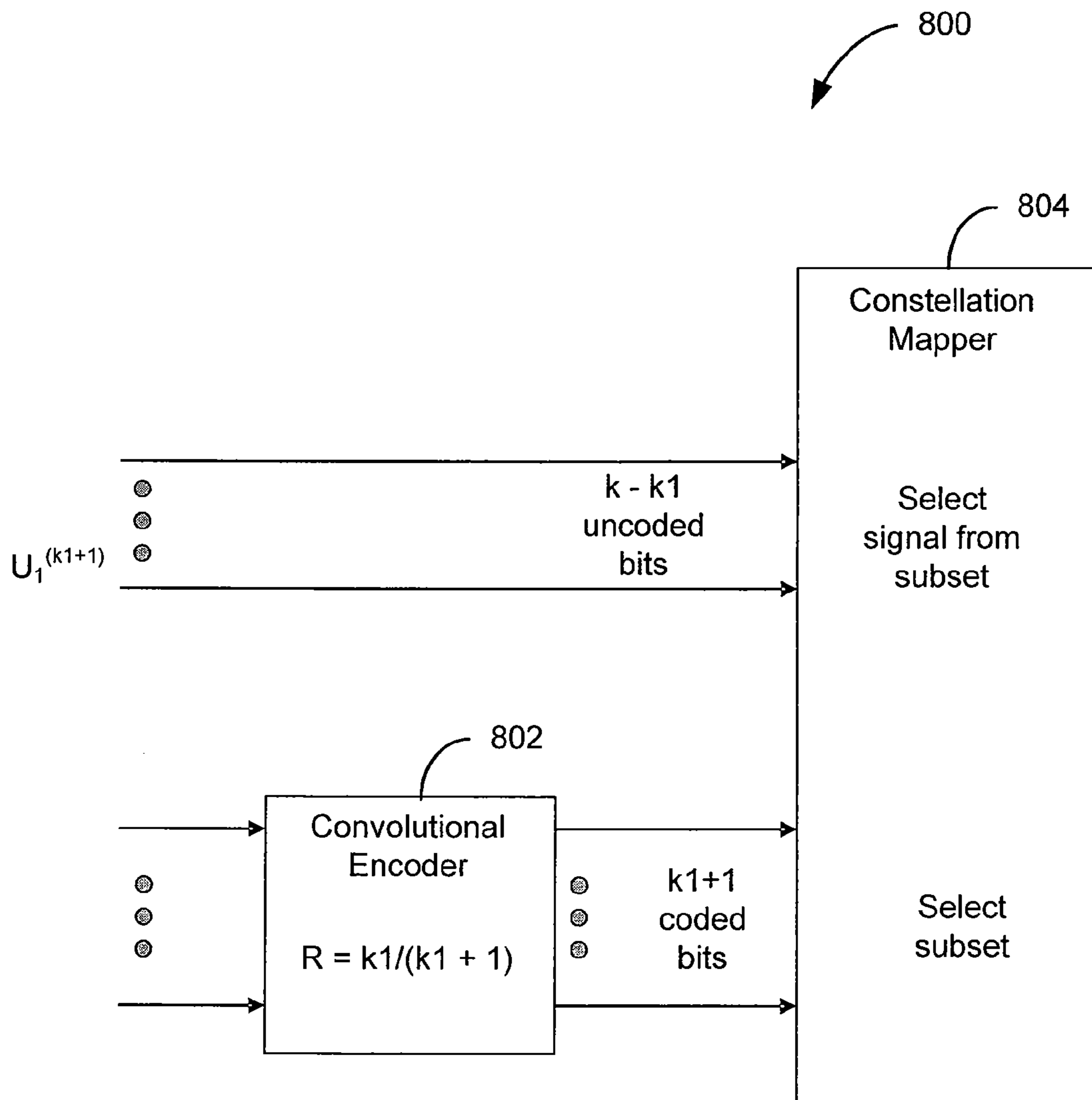
FIG. 8 (PRIOR ART)
