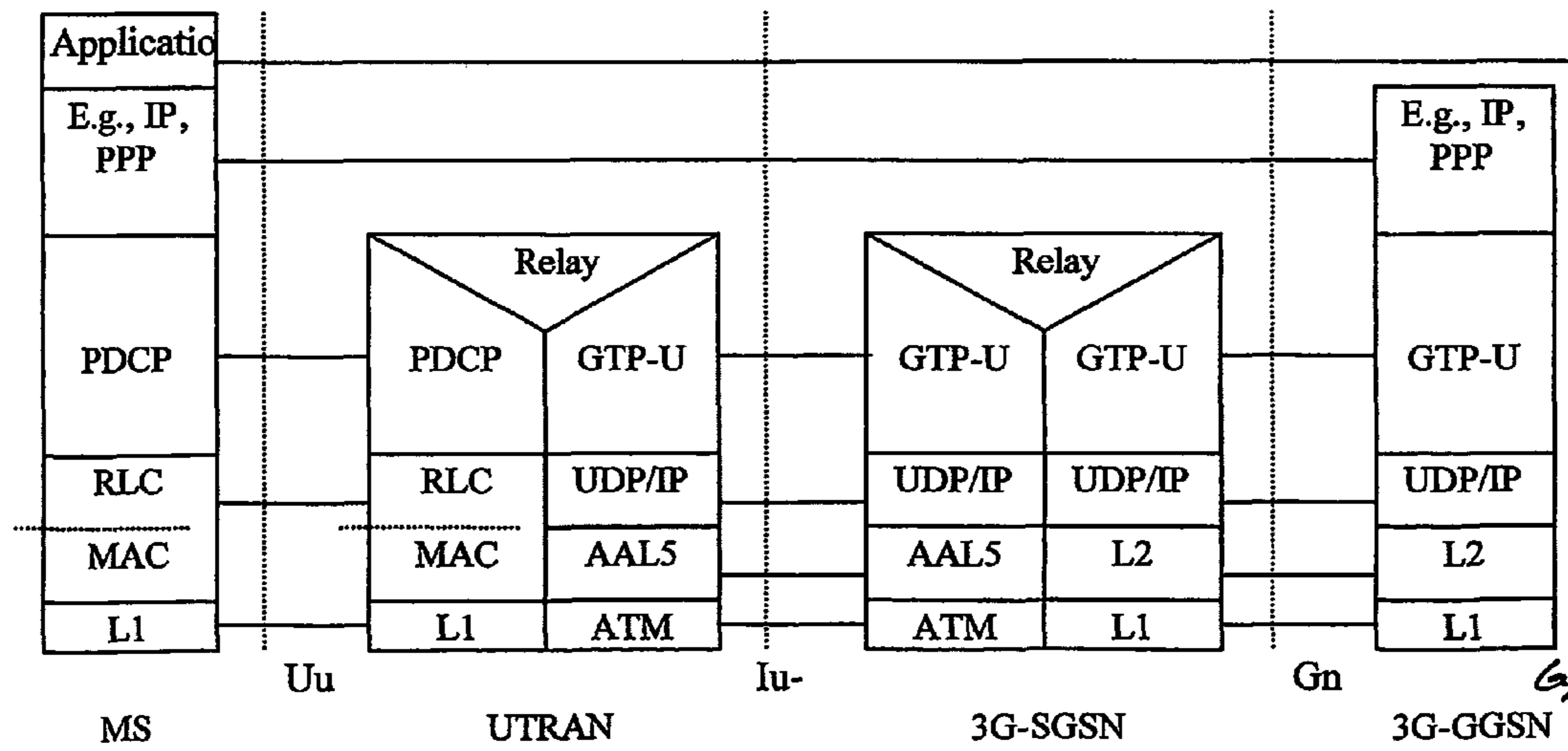
Fig. 3 – prior art
