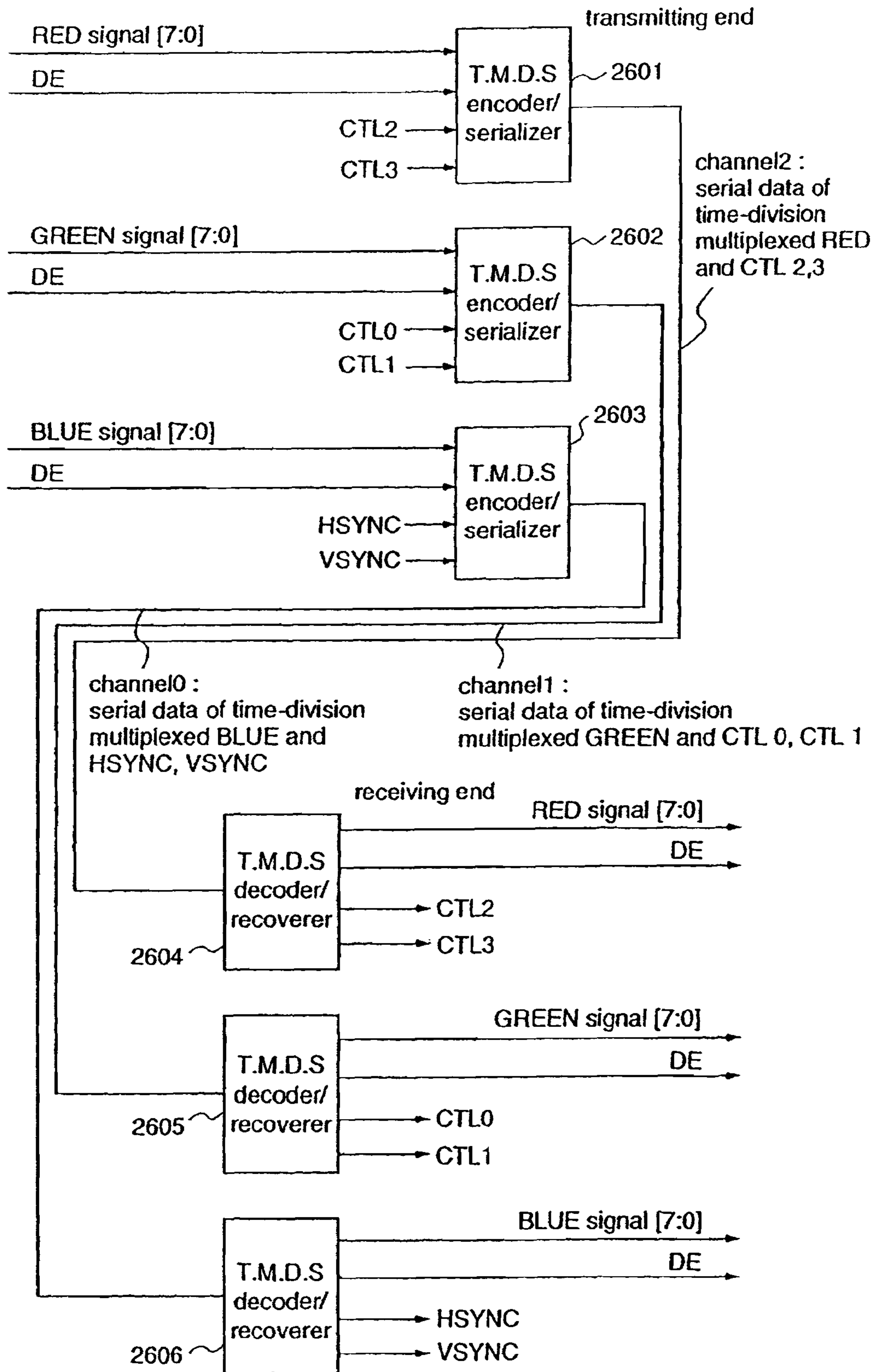
Fig.26 PRIOR ART
