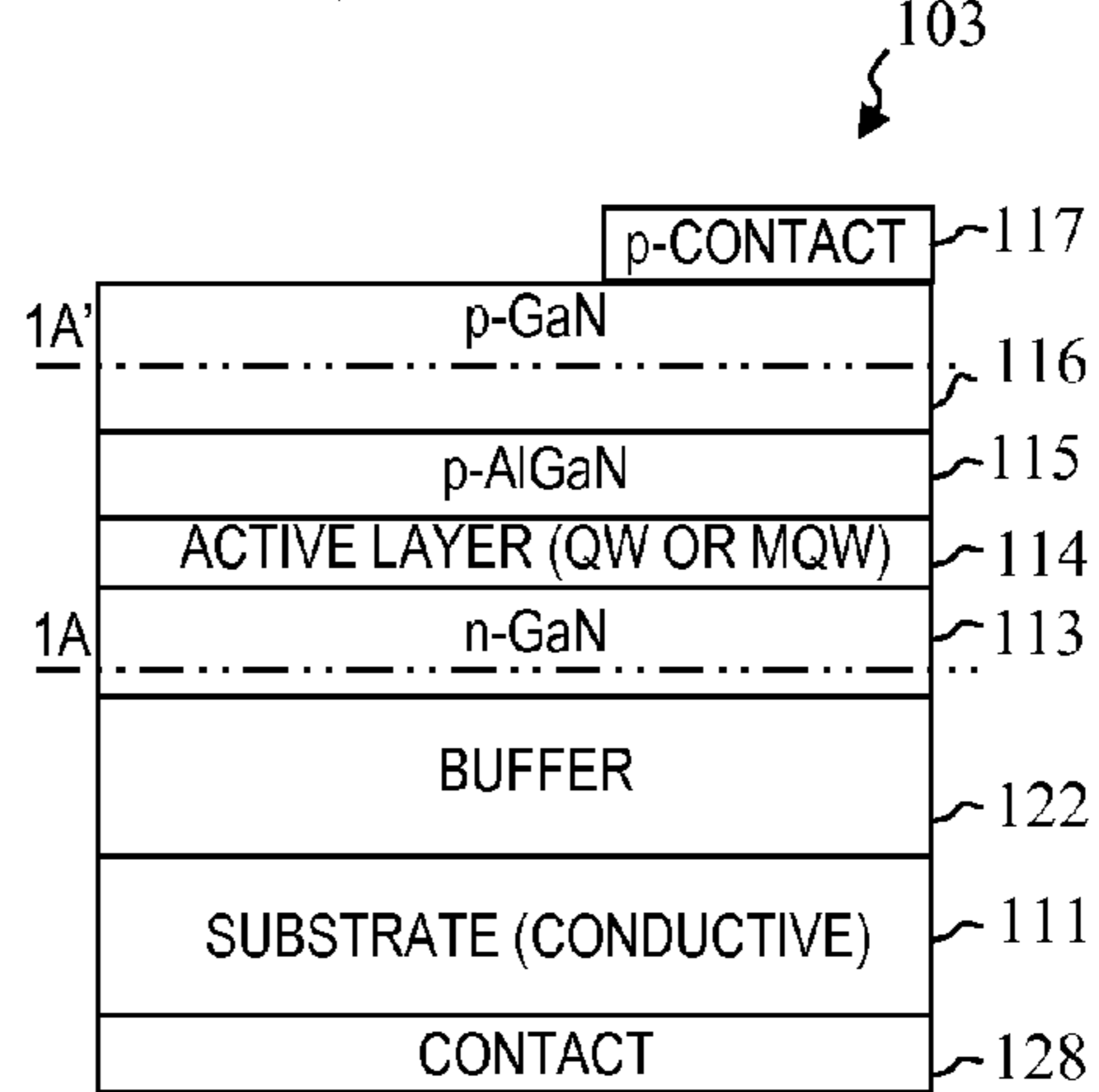
FIG. 1C (PRIOR ART)
