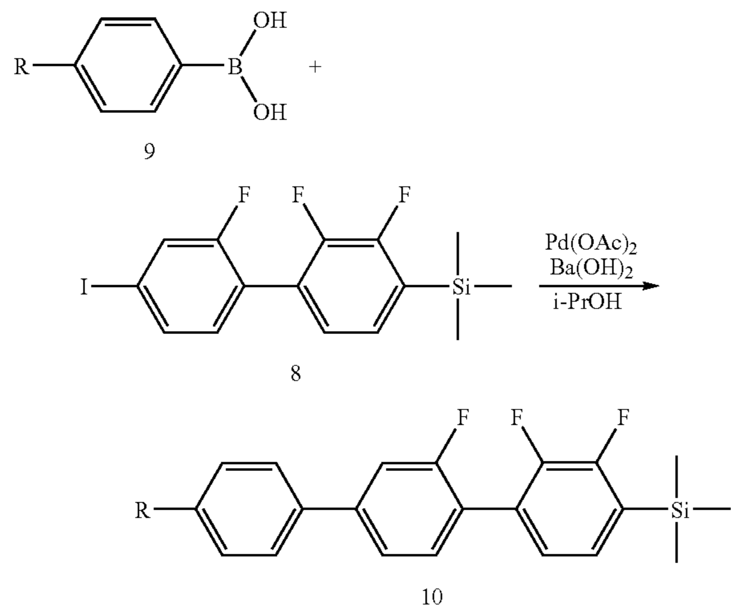
Scheme 2 Synthesis of the terphenyl (10)
