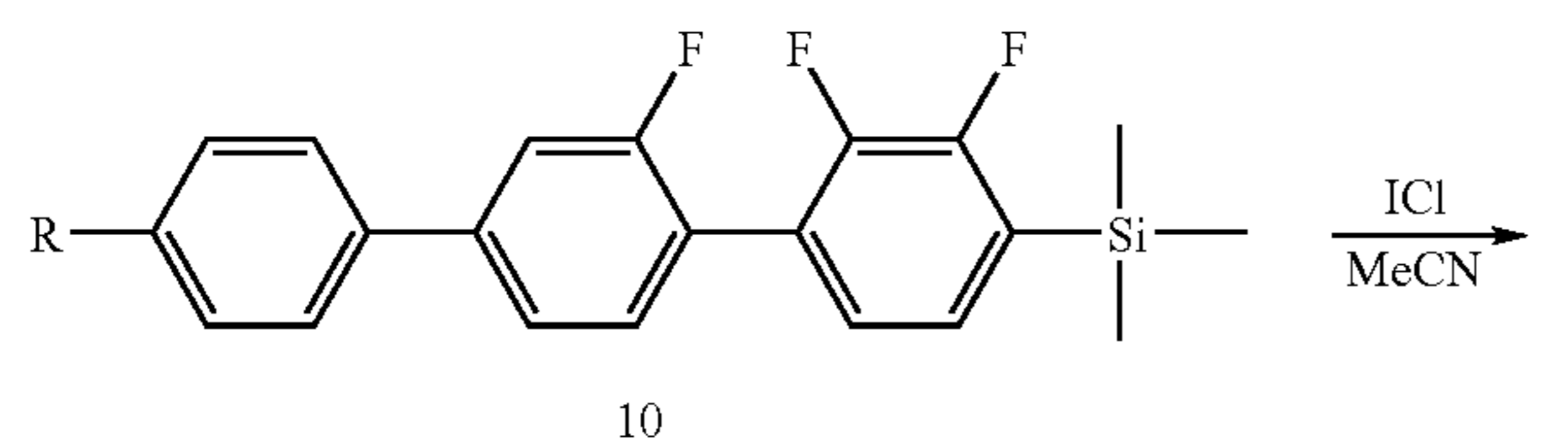
Scheme 3 Synthesis of the terphenyl (11) by iodo-desilylation
