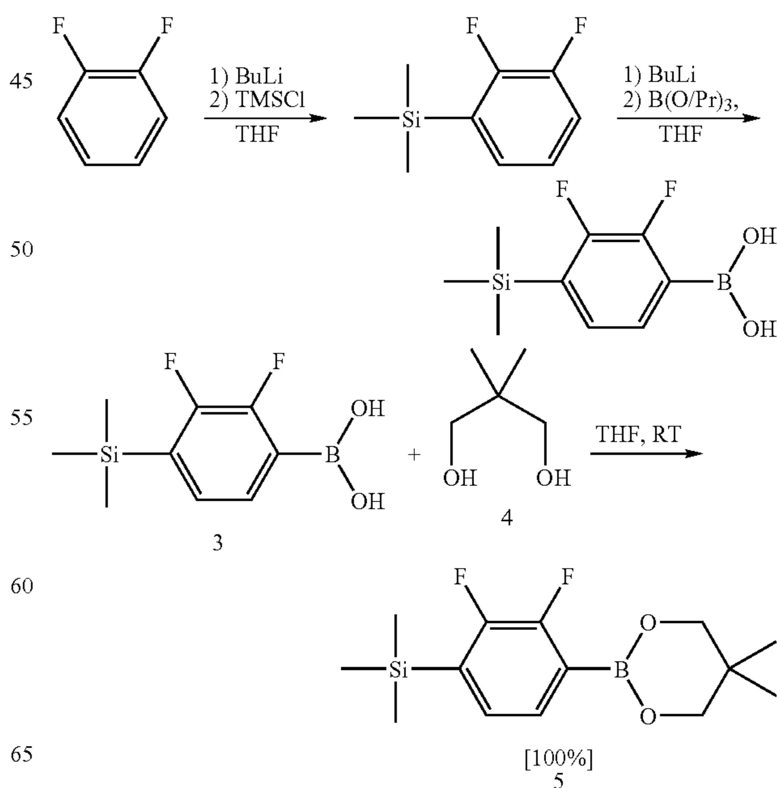
Scheme 1. Synthesis of the biphenyl (8)
