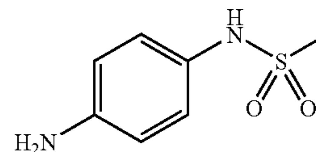
(b)': N-(4-Amino-phenyl)-methanesulfonamide
