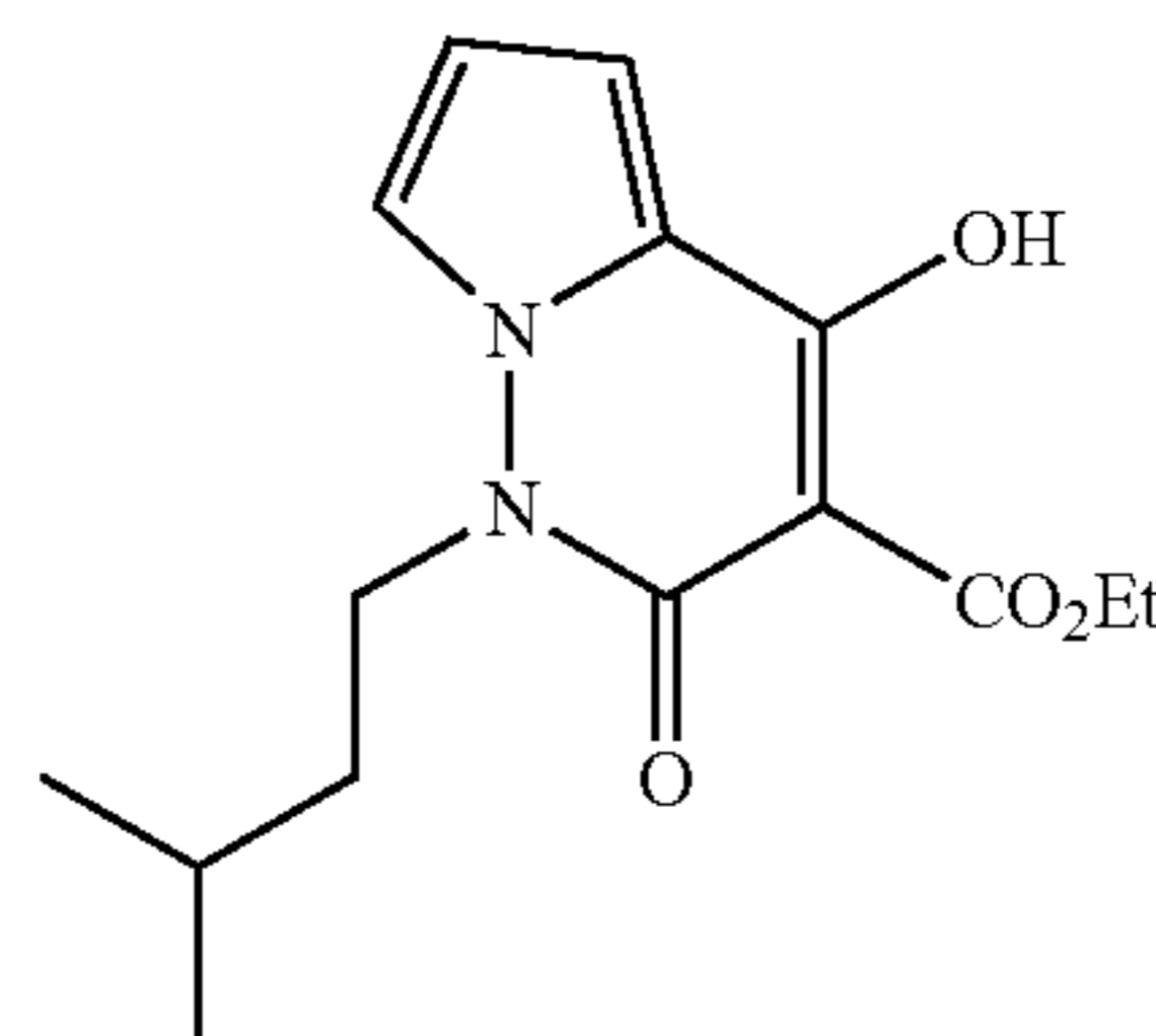
(f) 4-Hydroxy-1-(3-methyl-butyl)-2-oxo-1,2-dihydro-pyrrolo[1,2-b]pyridazine-3-carboxylic acid ethyl ester
