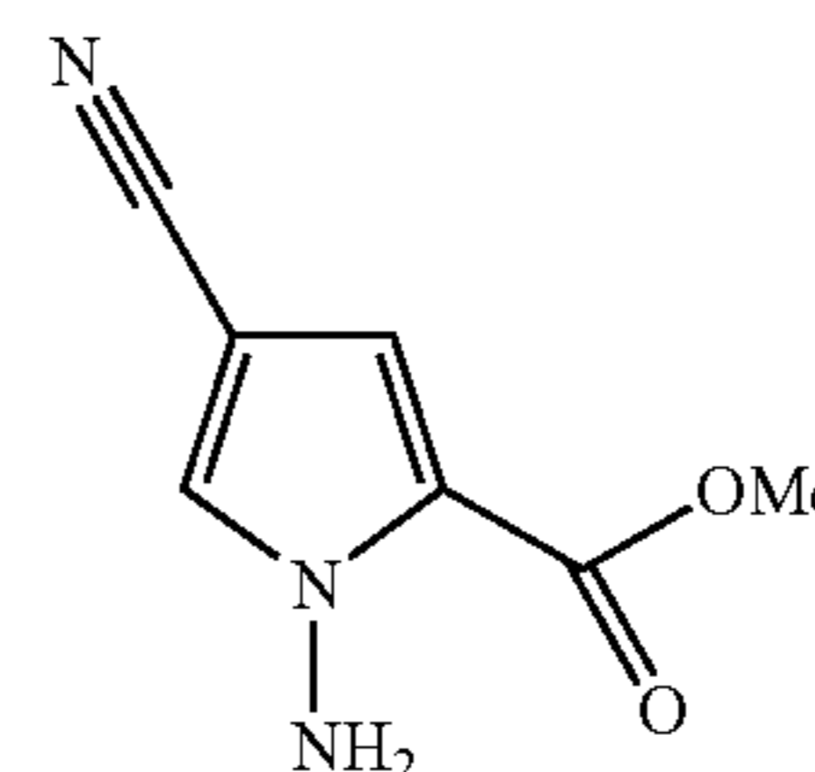
b) 1-Amino-4-cyano-1H-pyrrole-2-carboxylic acid methyl ester
