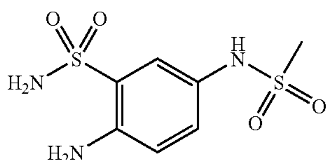
d) 2-Amino-5-methanesulfonylamino-benzenesulfonamide
