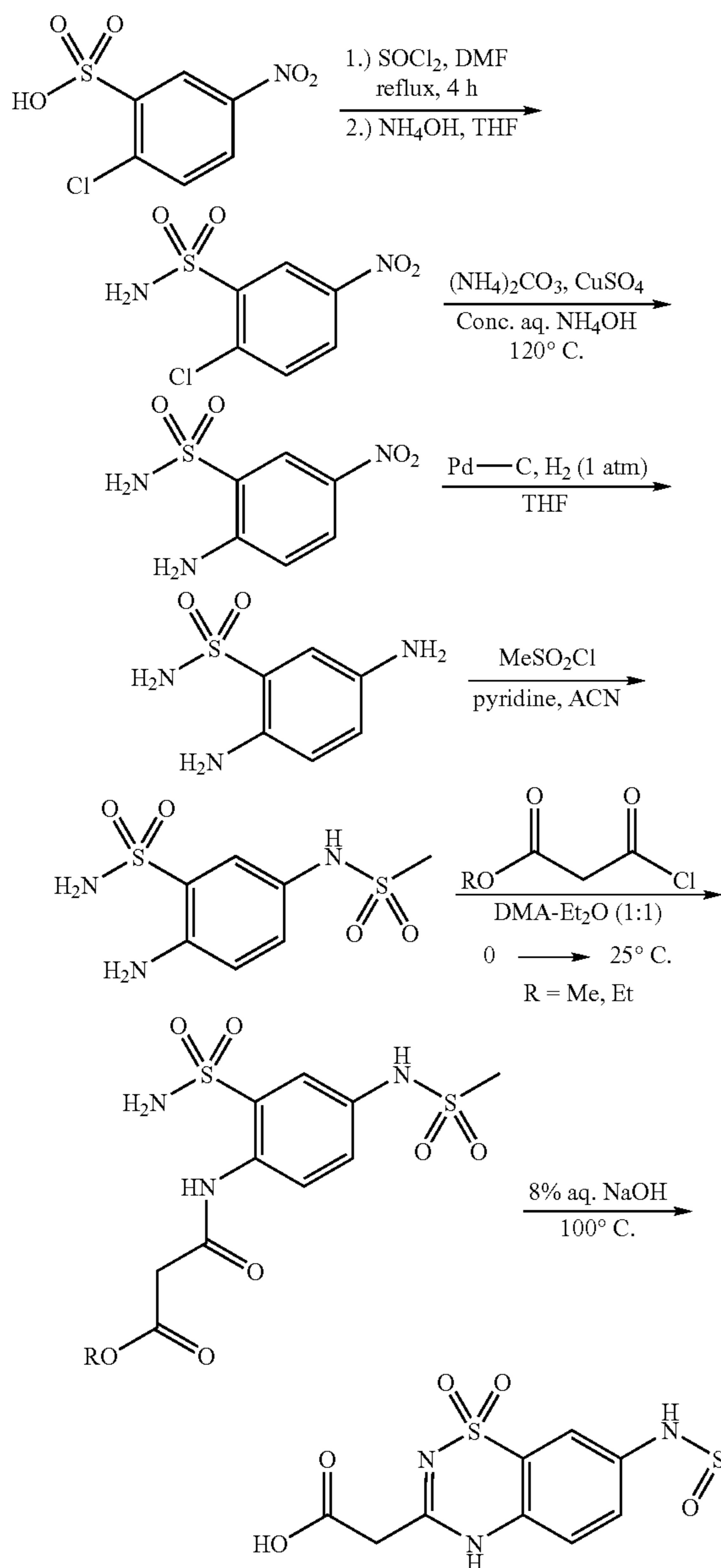
Scheme 11
