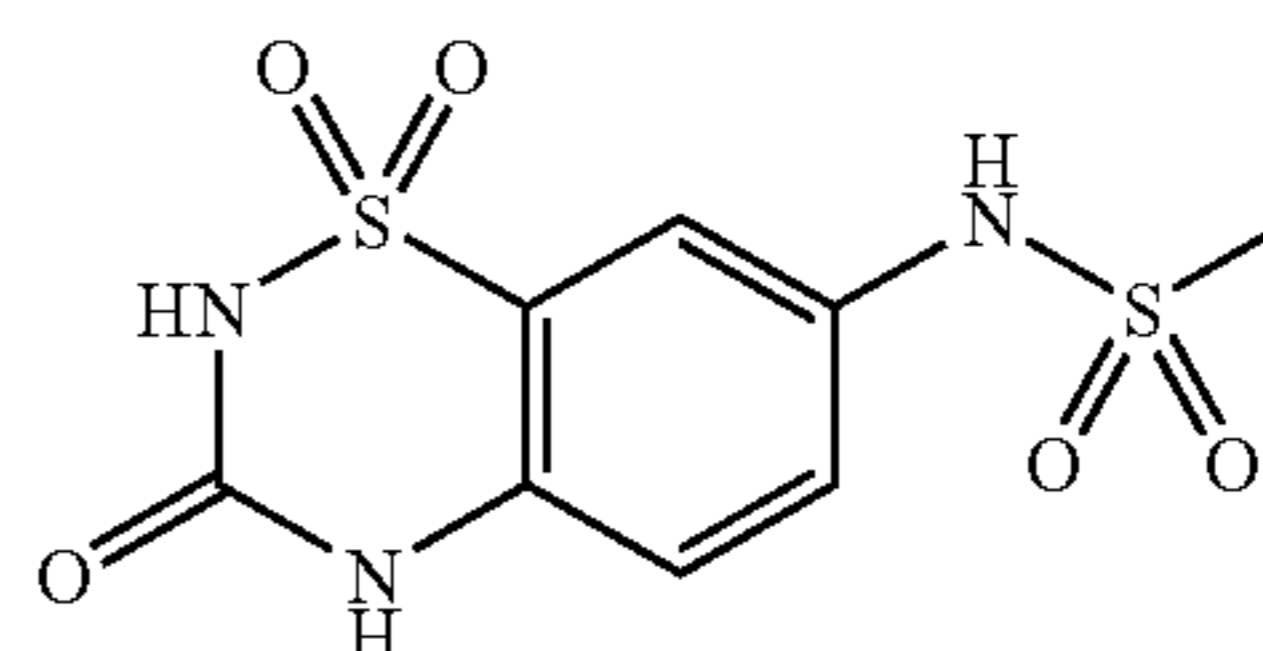
(c)': N-(1,1,3-Trioxo-1,2,3,4-tetrahydro-1 \lambda^6 -benzo[1,2,4]thiadiazin-7-yl)-methanesulfonamide
