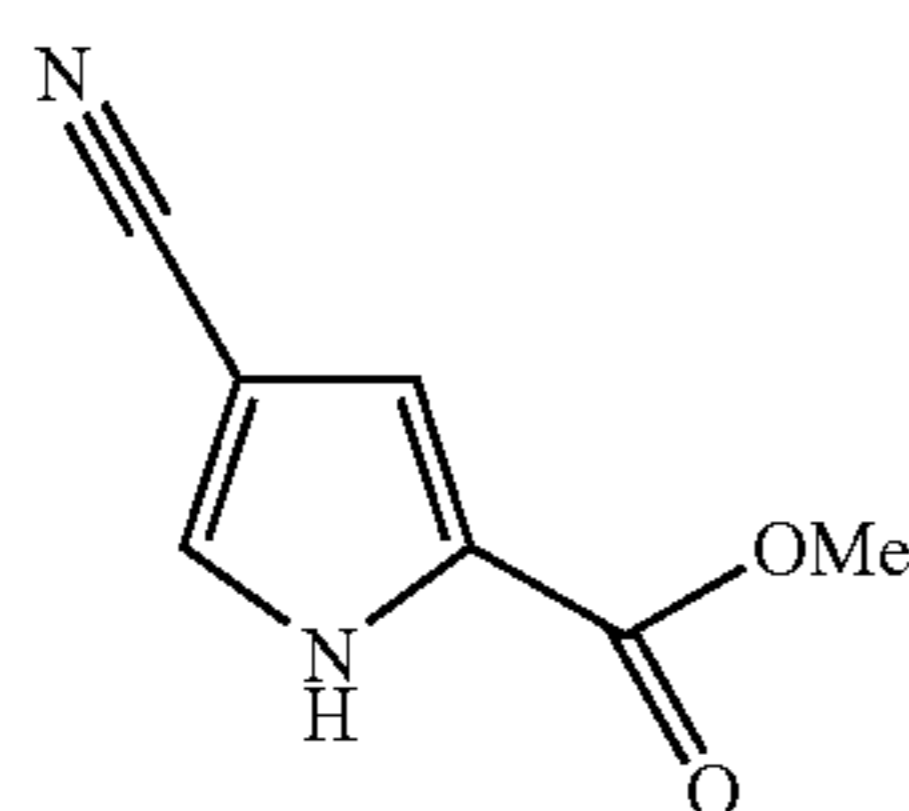
a) 4-Cyano-1H-pyrrole-2-carboxylic acid methyl ester
