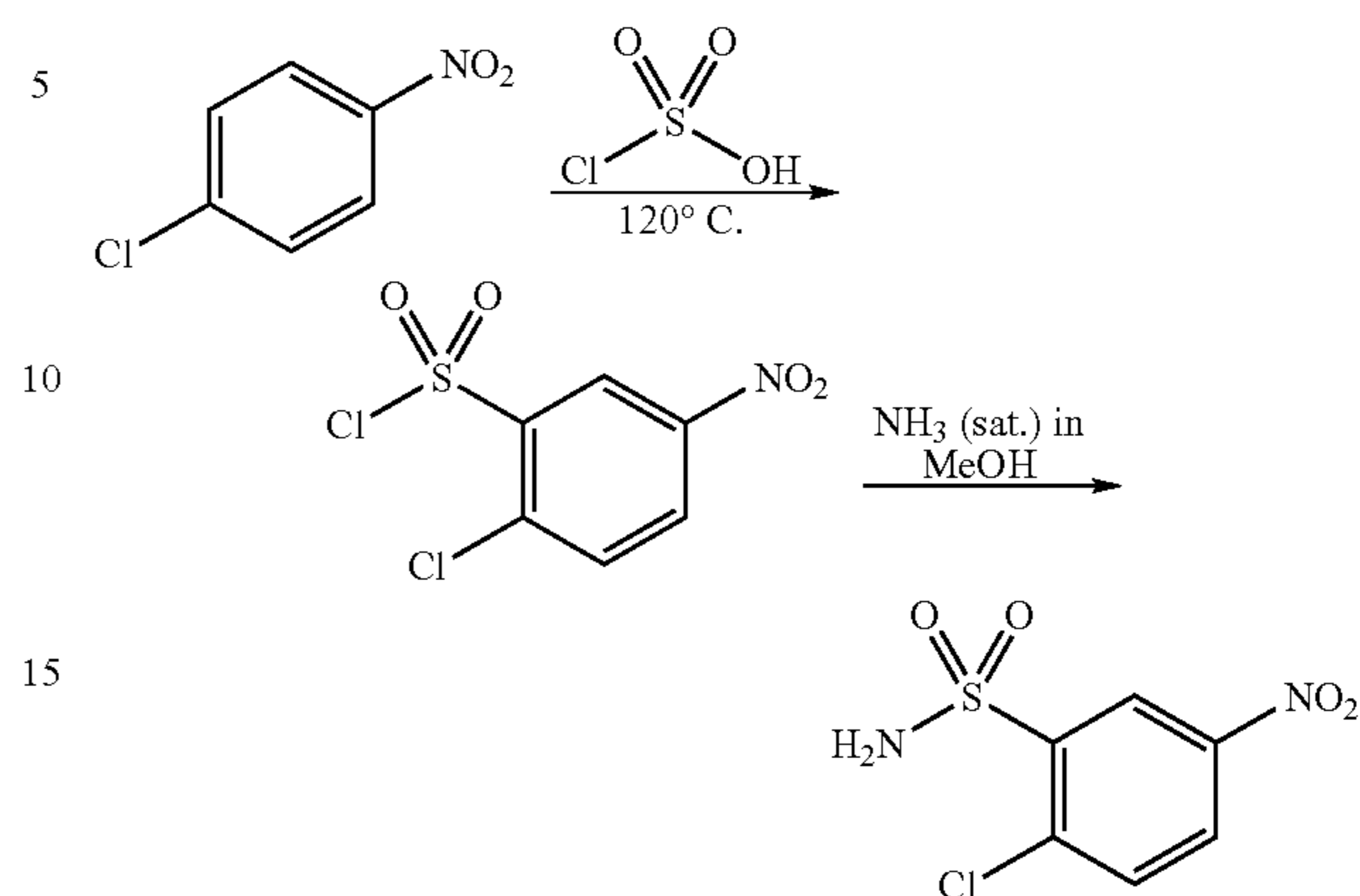
Scheme 12
