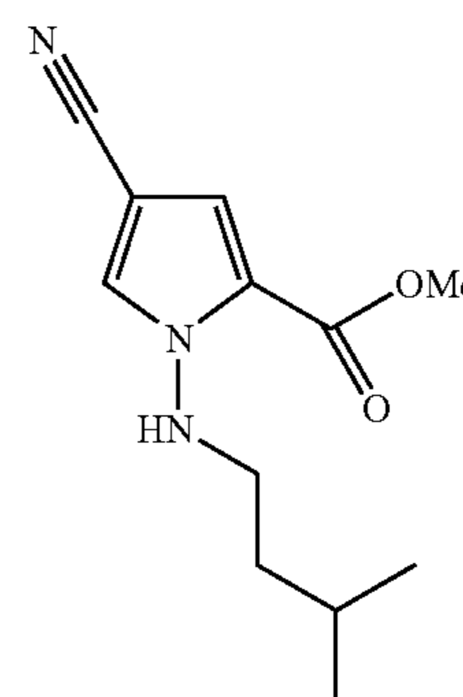
c) 4-Cyano-1-(3-methyl-butylamino)-1H-pyrrole-2-carboxylic acid methyl ester
