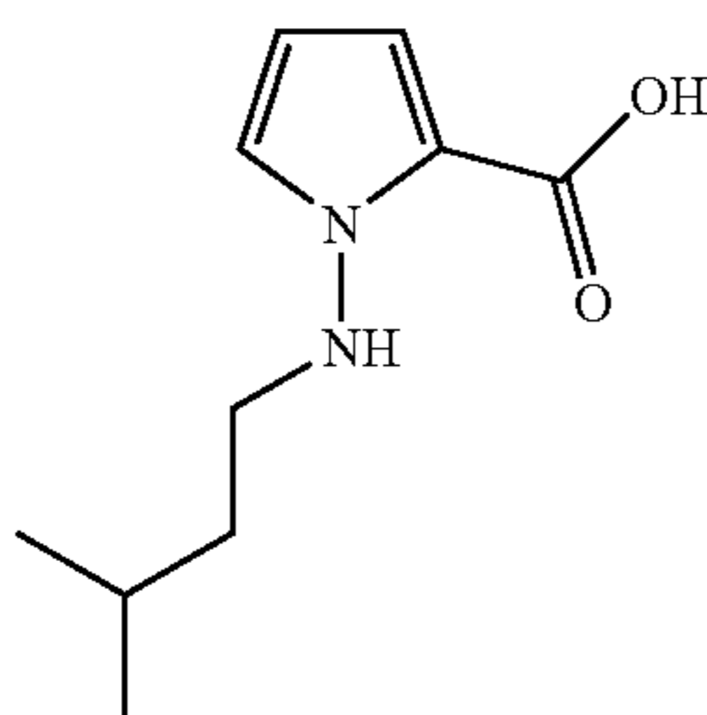
d) 1-(3-Methyl-butylamino)-1H-pyrrole-2-carboxylic acid
