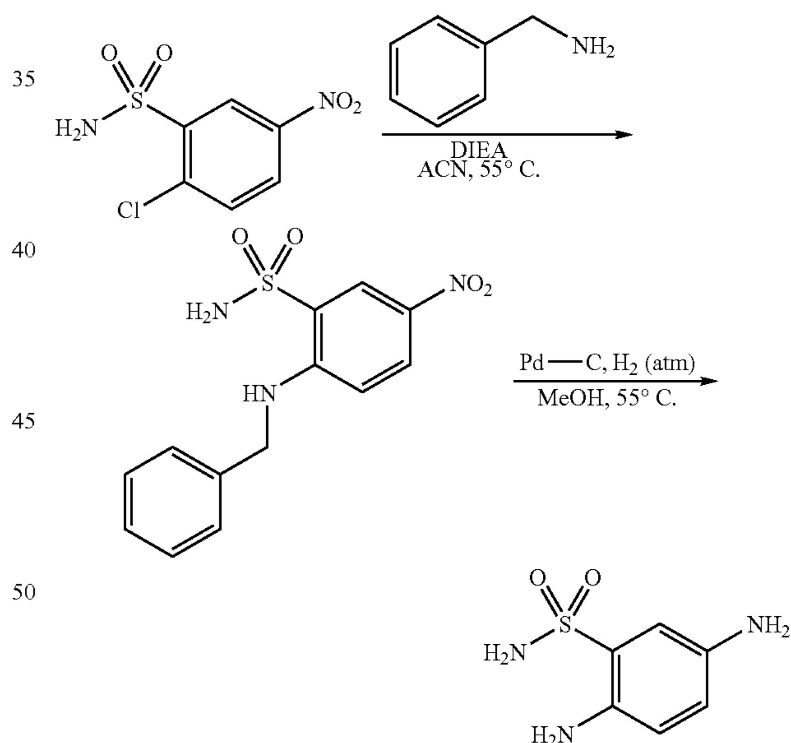
Scheme 13
