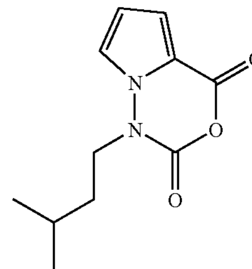
(e) 4-(3-Methyl-butyl)-6-oxa-3a,4-diaza-indene-5,7-dione
