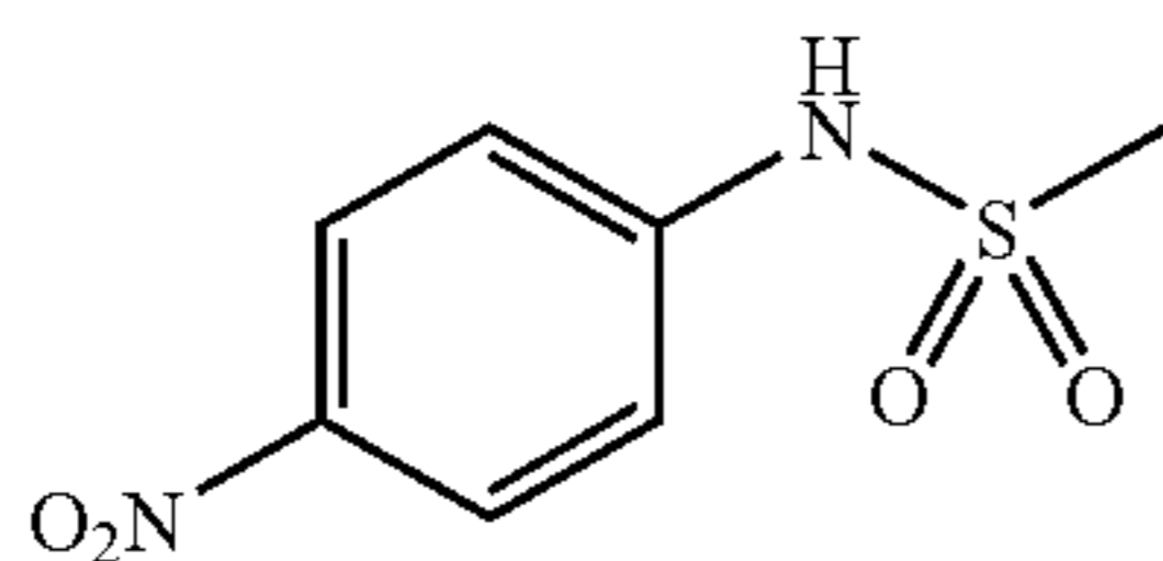
(a)': N-(4-Nitro-phenyl)-methanesulfonamide
