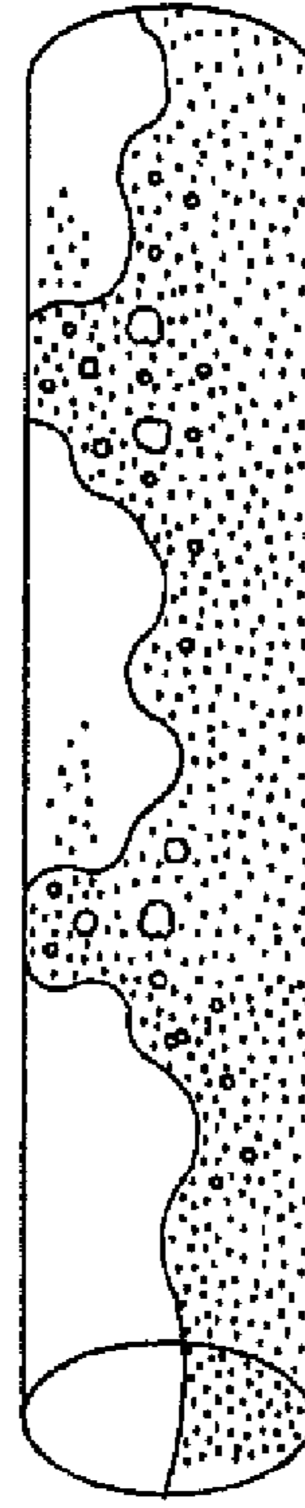
SLUG FLOW
