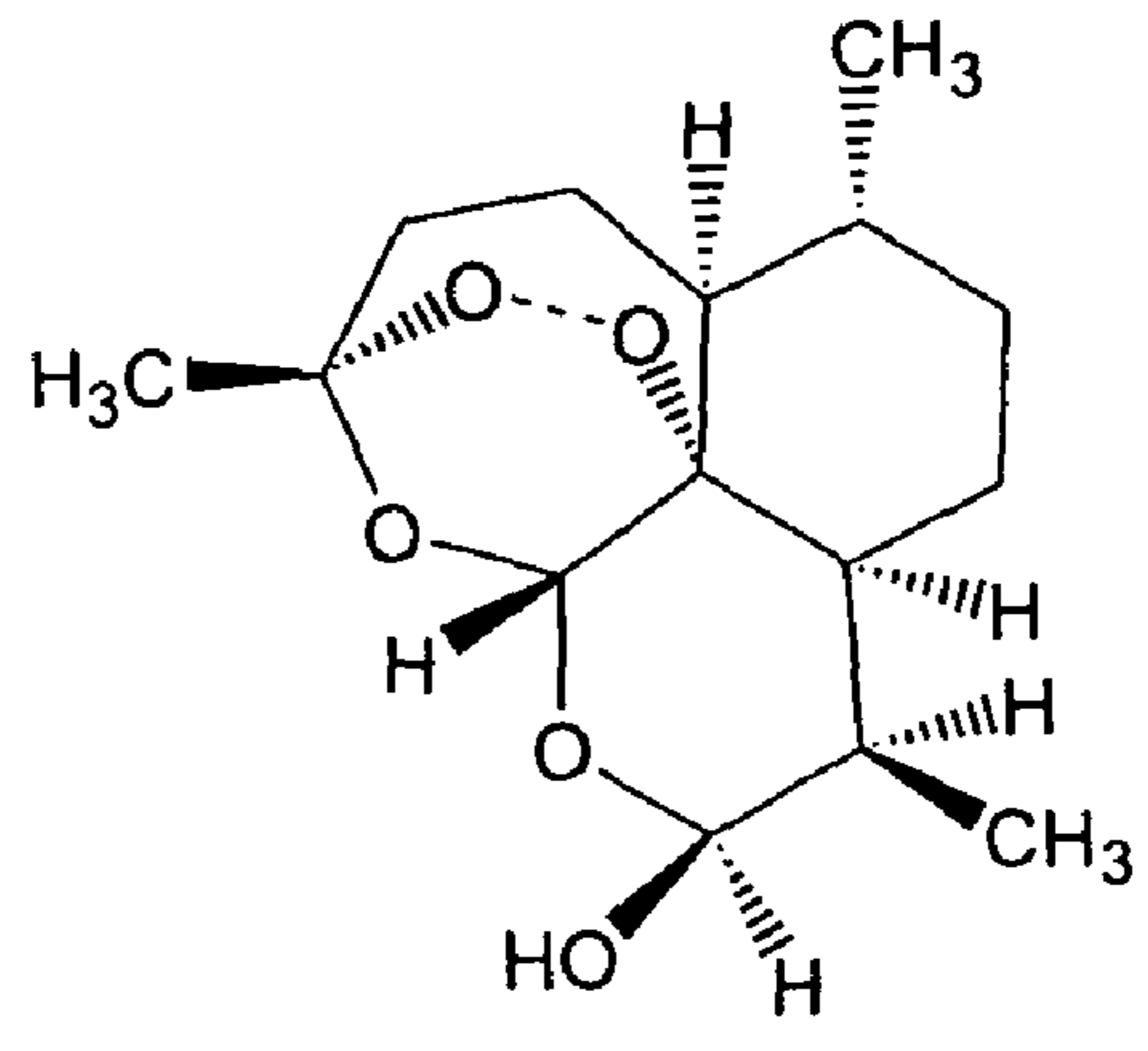
Dihydroartemisinin
