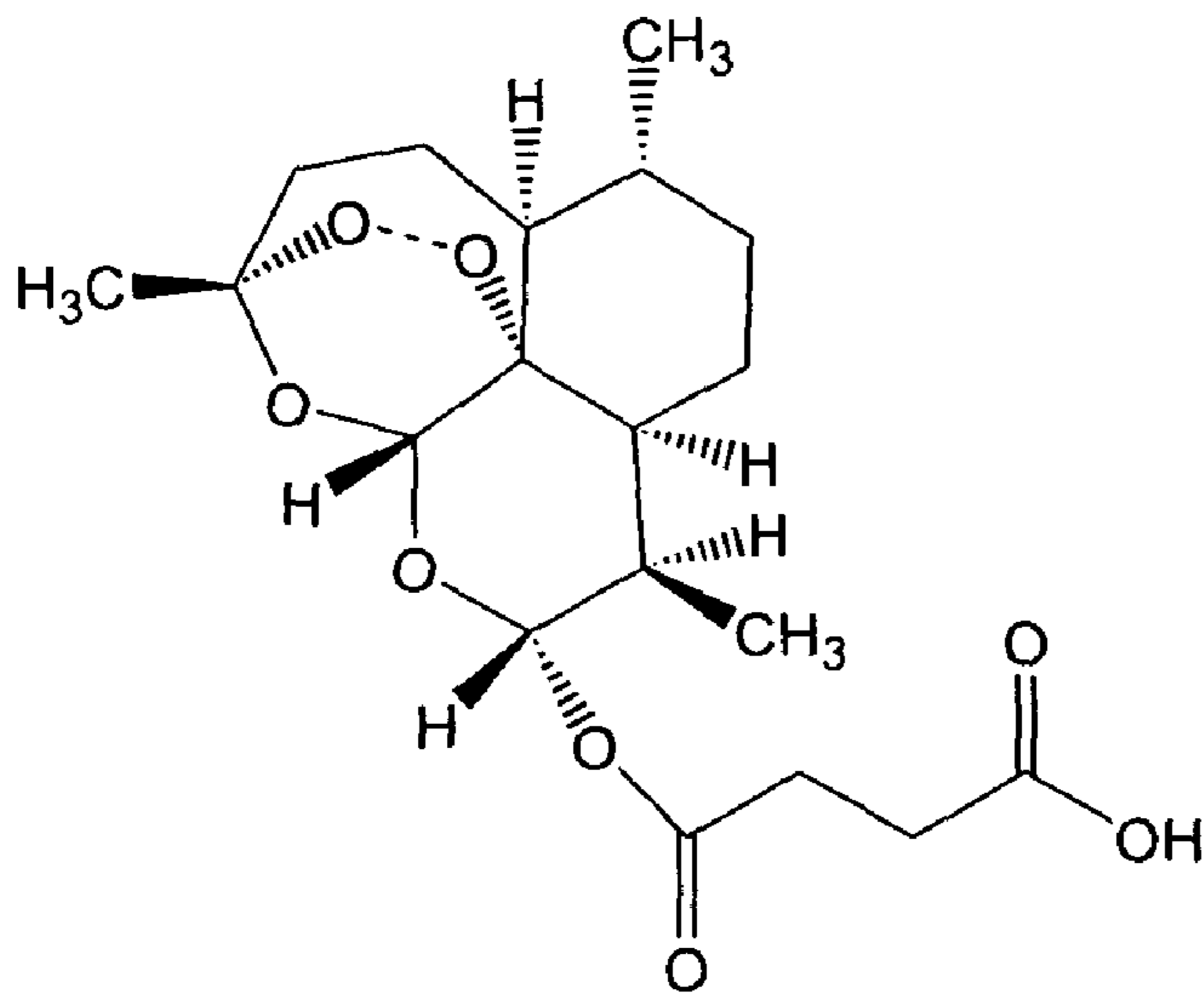
Artesunate
