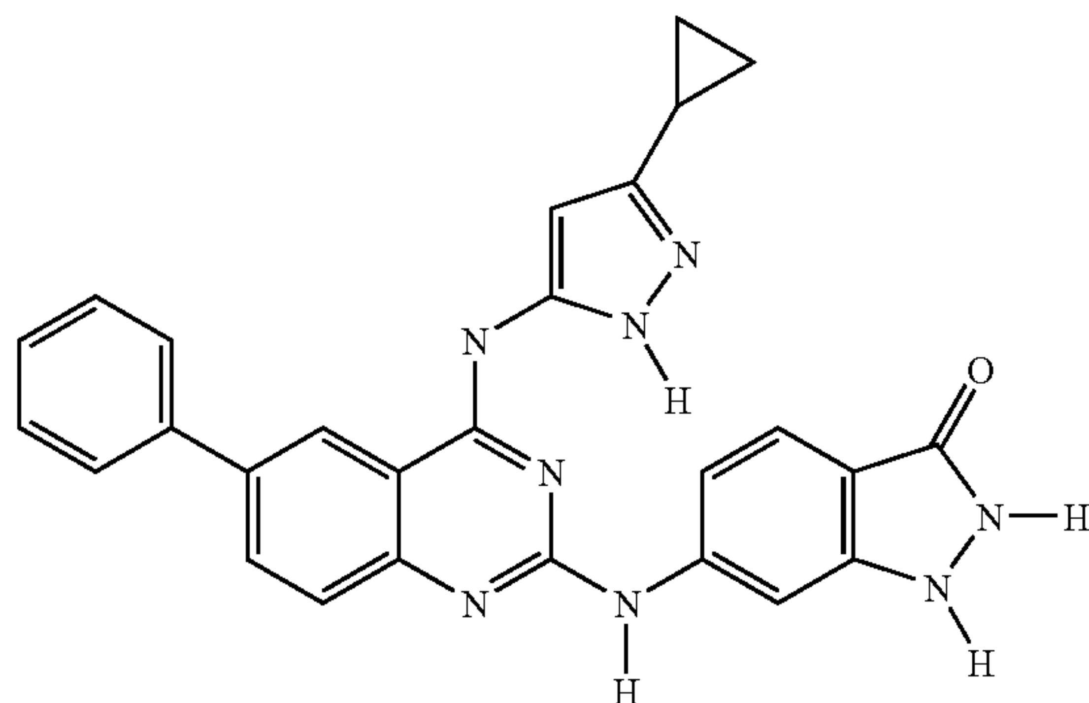
Step F: 6-[4-(5-Cyclopropyl-2H-pyrazol-3-ylamino)-6-phenyl-quinazolin-2-ylamino]-1,2-dihydro-indazol-3-one
