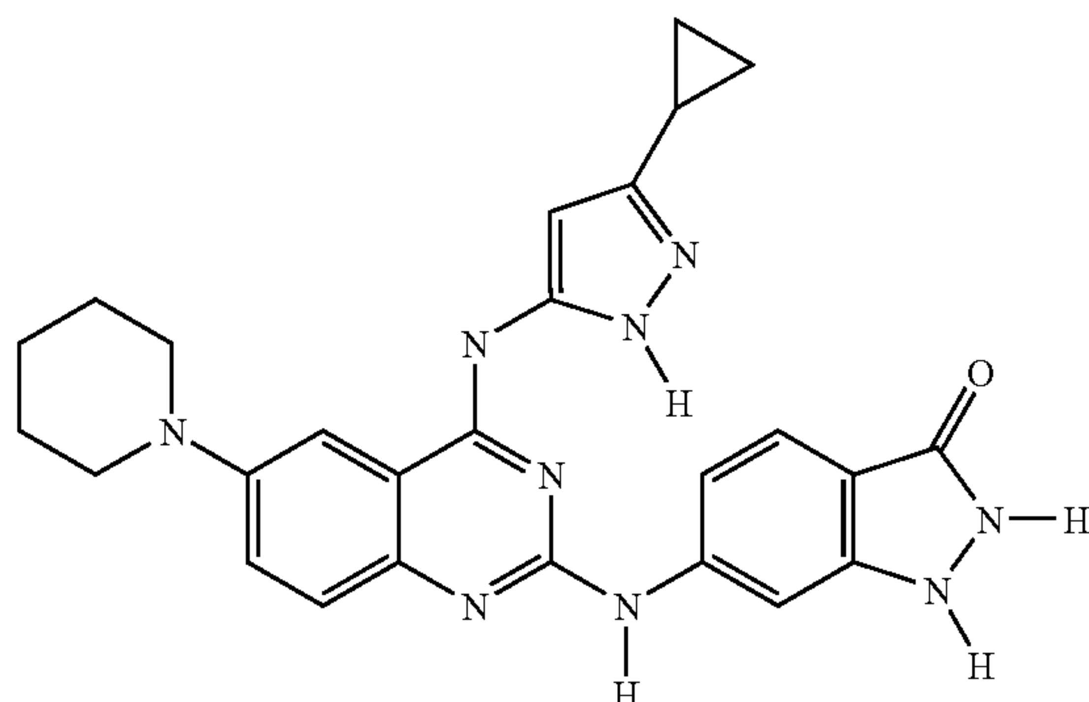
Step G: 6-[4-(5-Cyclopropyl-2H-pyrazol-3-ylamino)-6-piperidin-1-yl-quinazolin-2-ylamino]-1,2-dihydro-indazol-3-one
