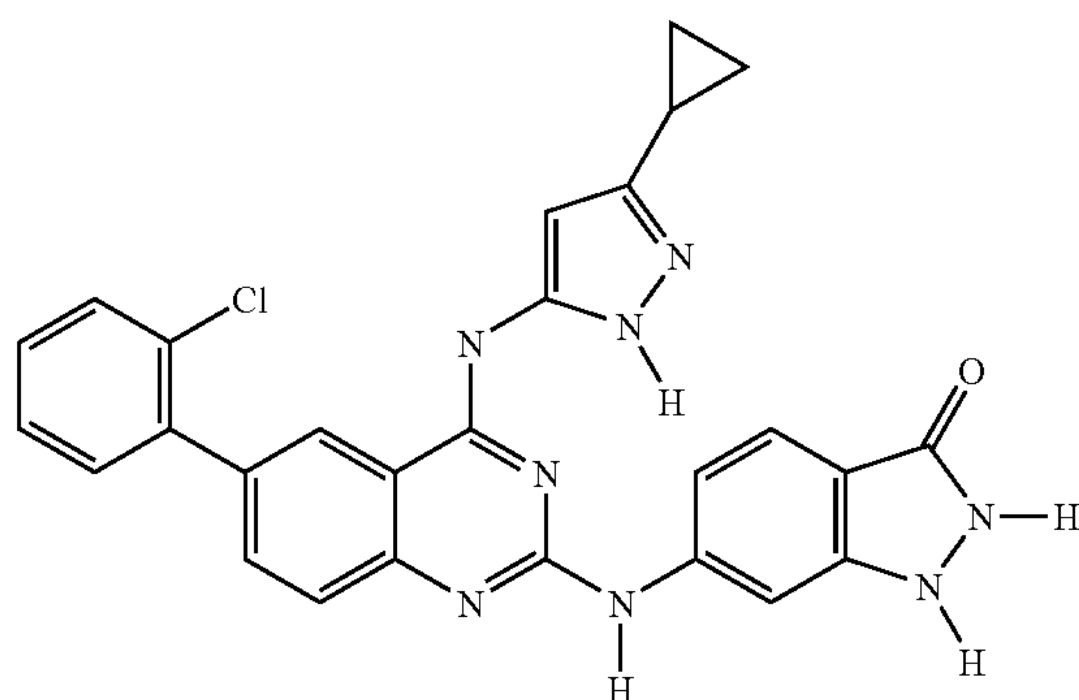
6-[6-(2-Chloro-phenyl)-4-(5-cyclopropyl-2H-pyrazol-3-ylamino)-quinazolin-2-ylamino]-1,2-dihydro-indazol-3-one
