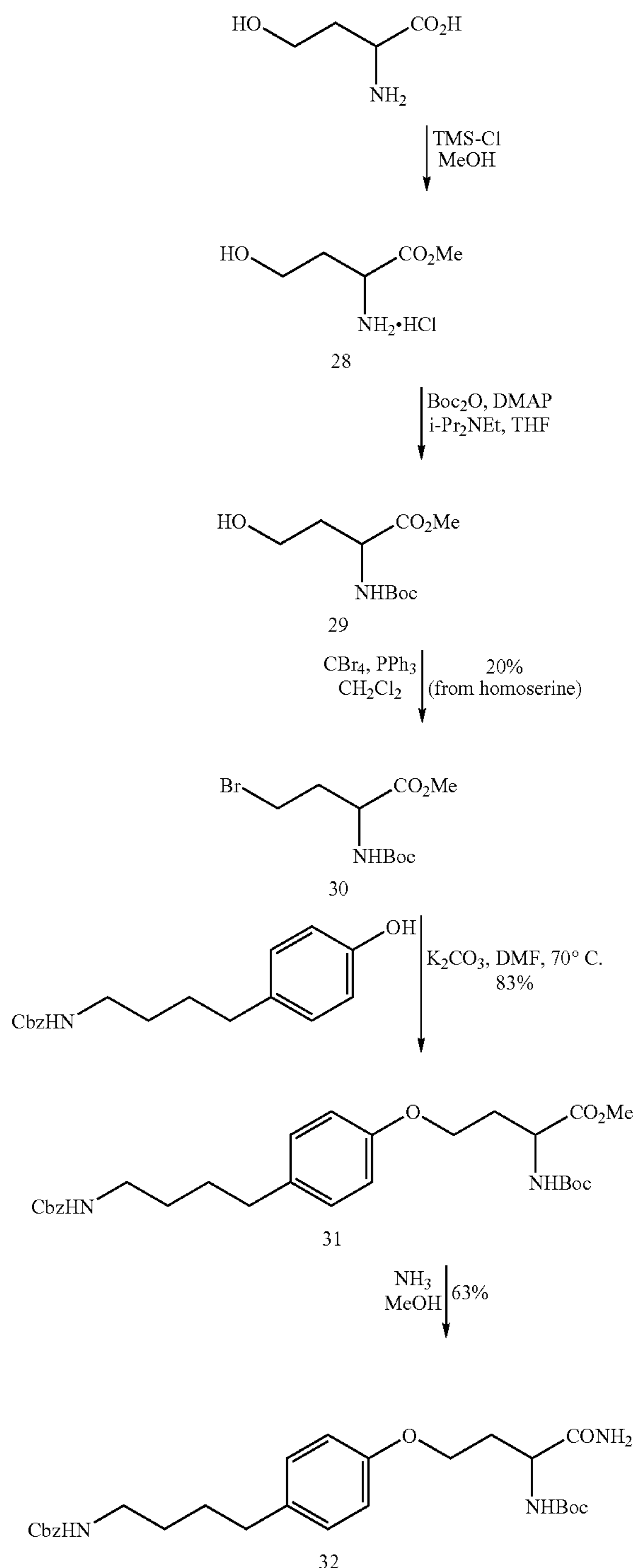
Scheme 7. Synthesis of Amino Amides and Esters
