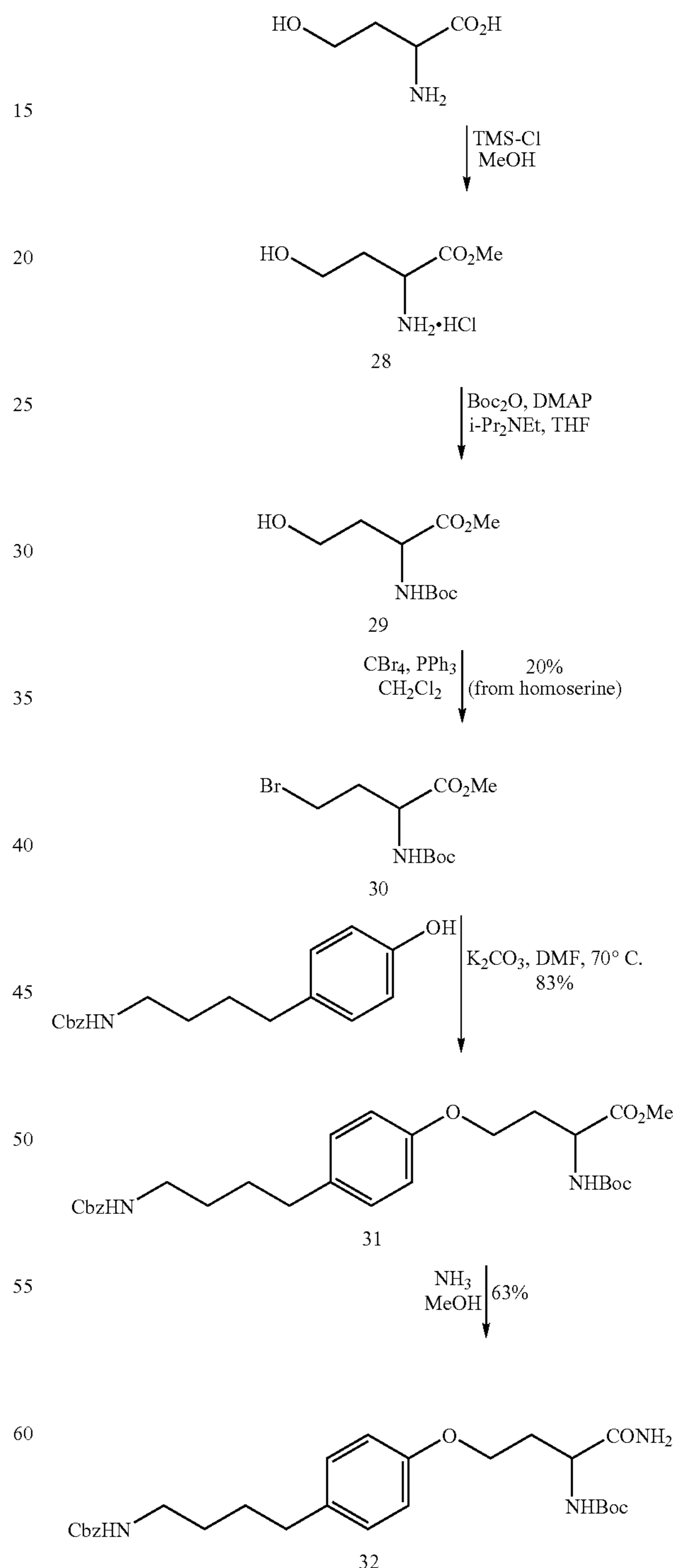
Scheme 7. Synthesis of Amino Amides and Esters
