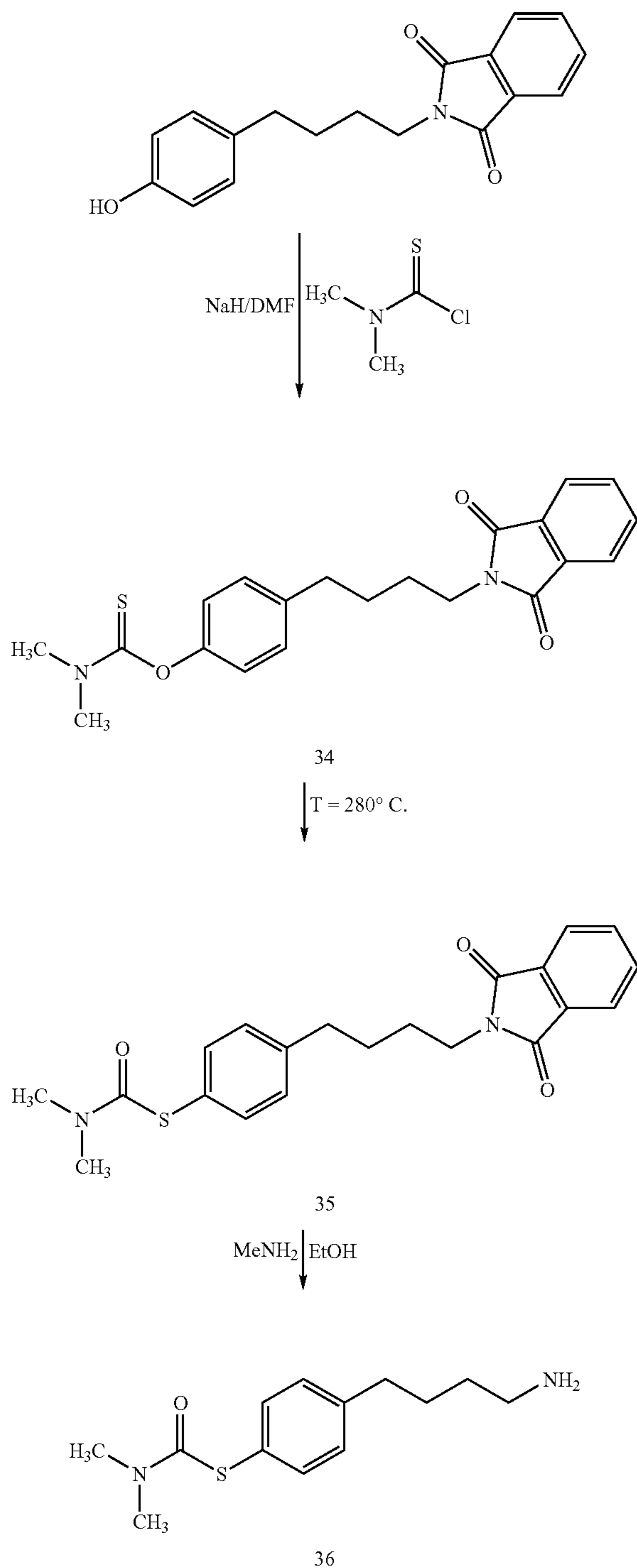
Scheme 9. Synthesis of Thia Amide Precursors
