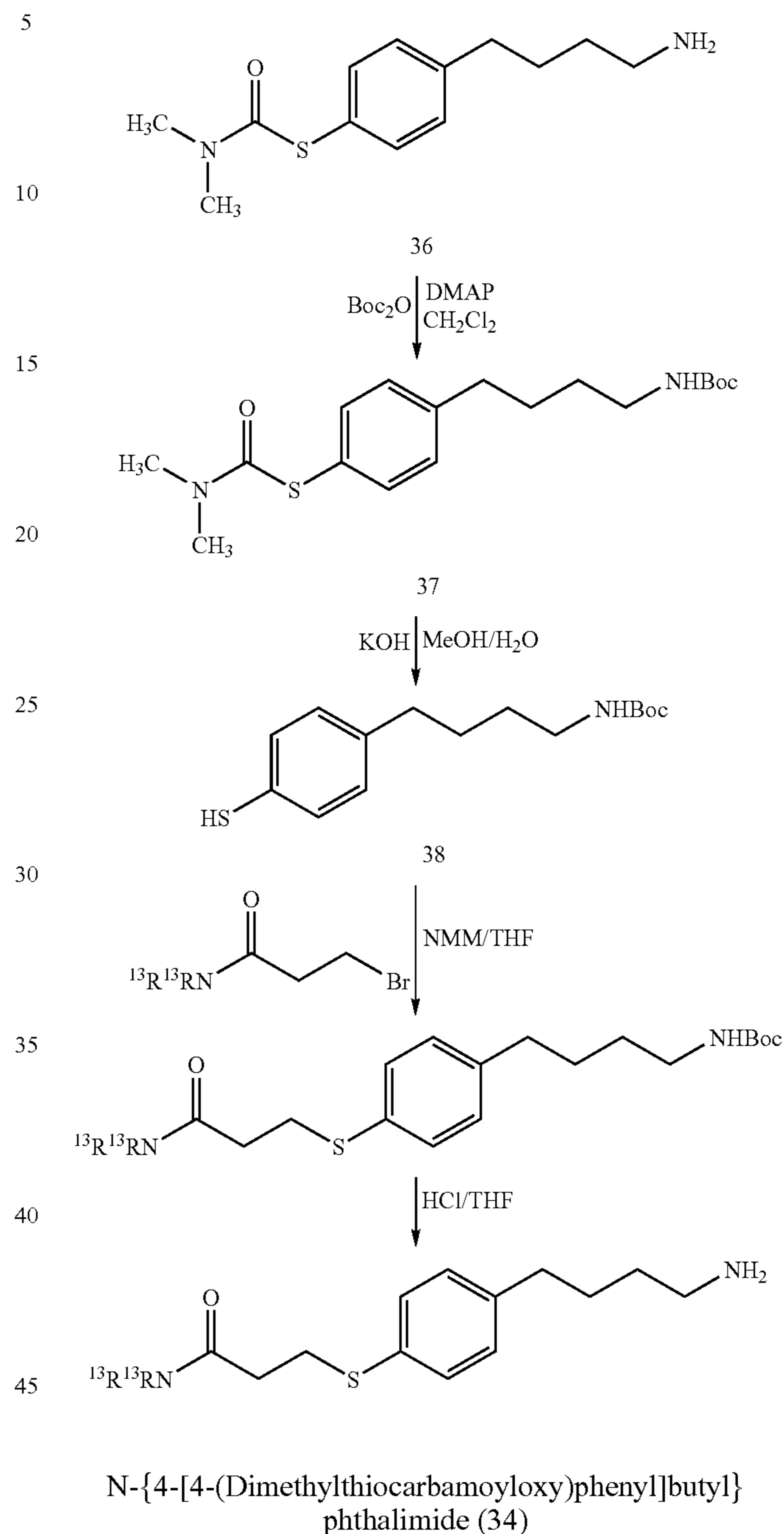
Scheme 14. Synthesis of Thia Amides
