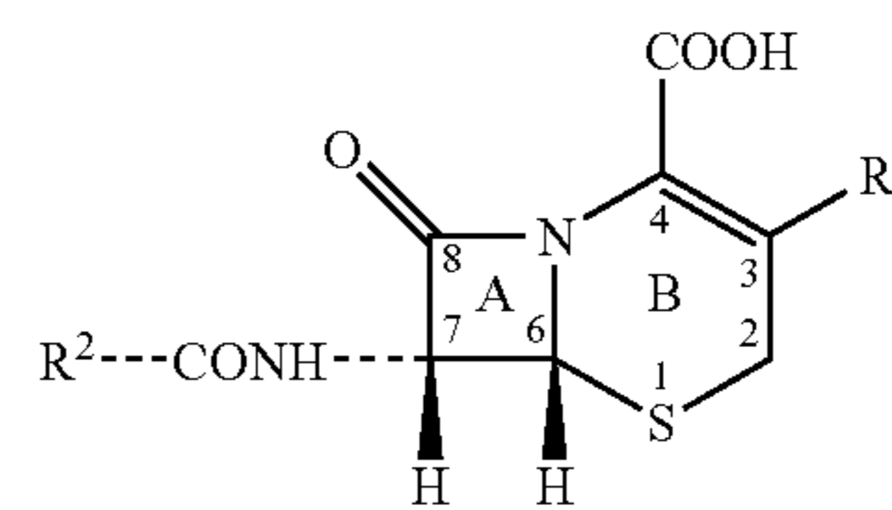
cephalosporin nucleus A \beta -lactam ring B dihydrothiazine ring
