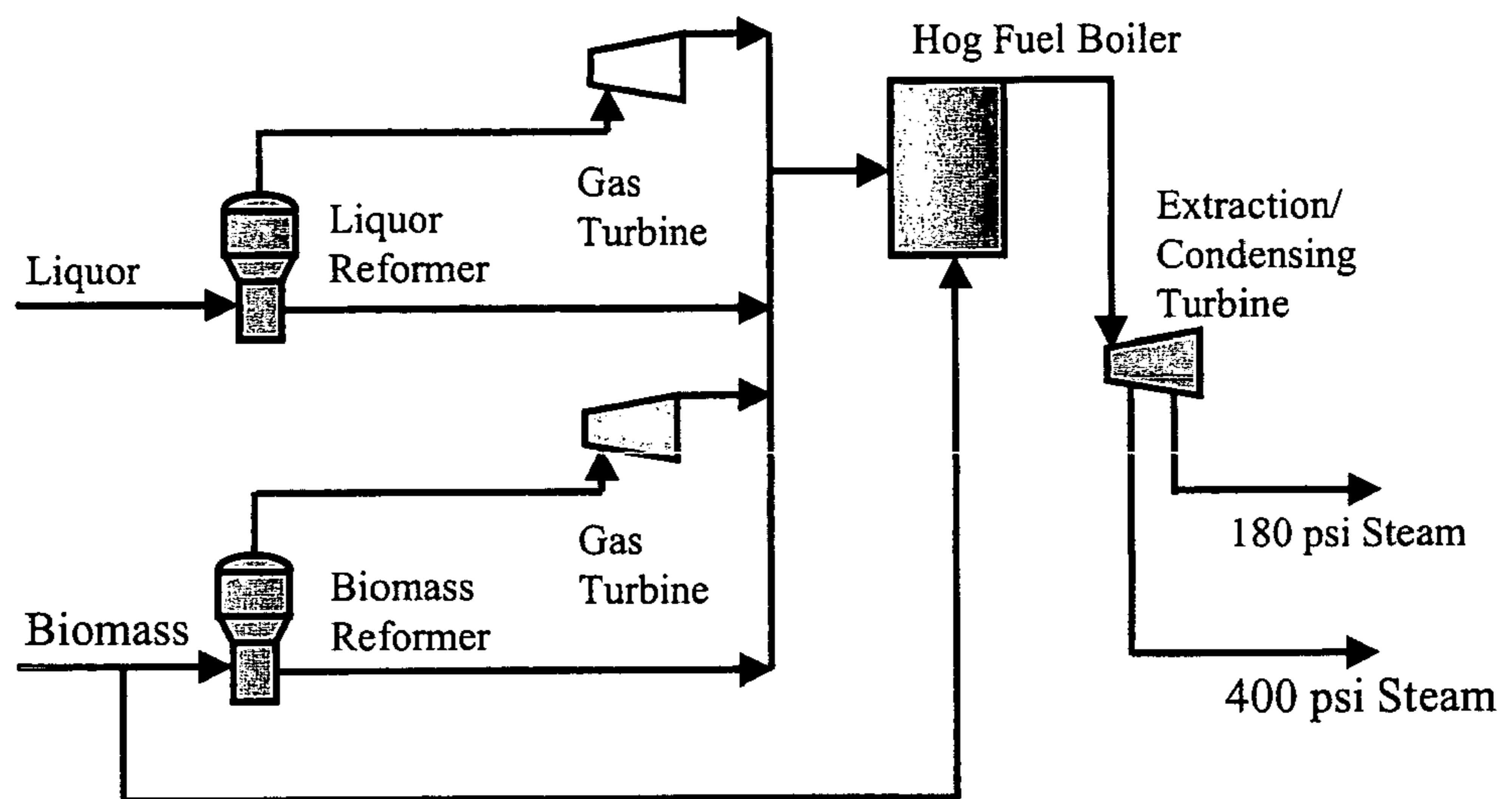
Figure 10 Steam Reforming Co-generation
