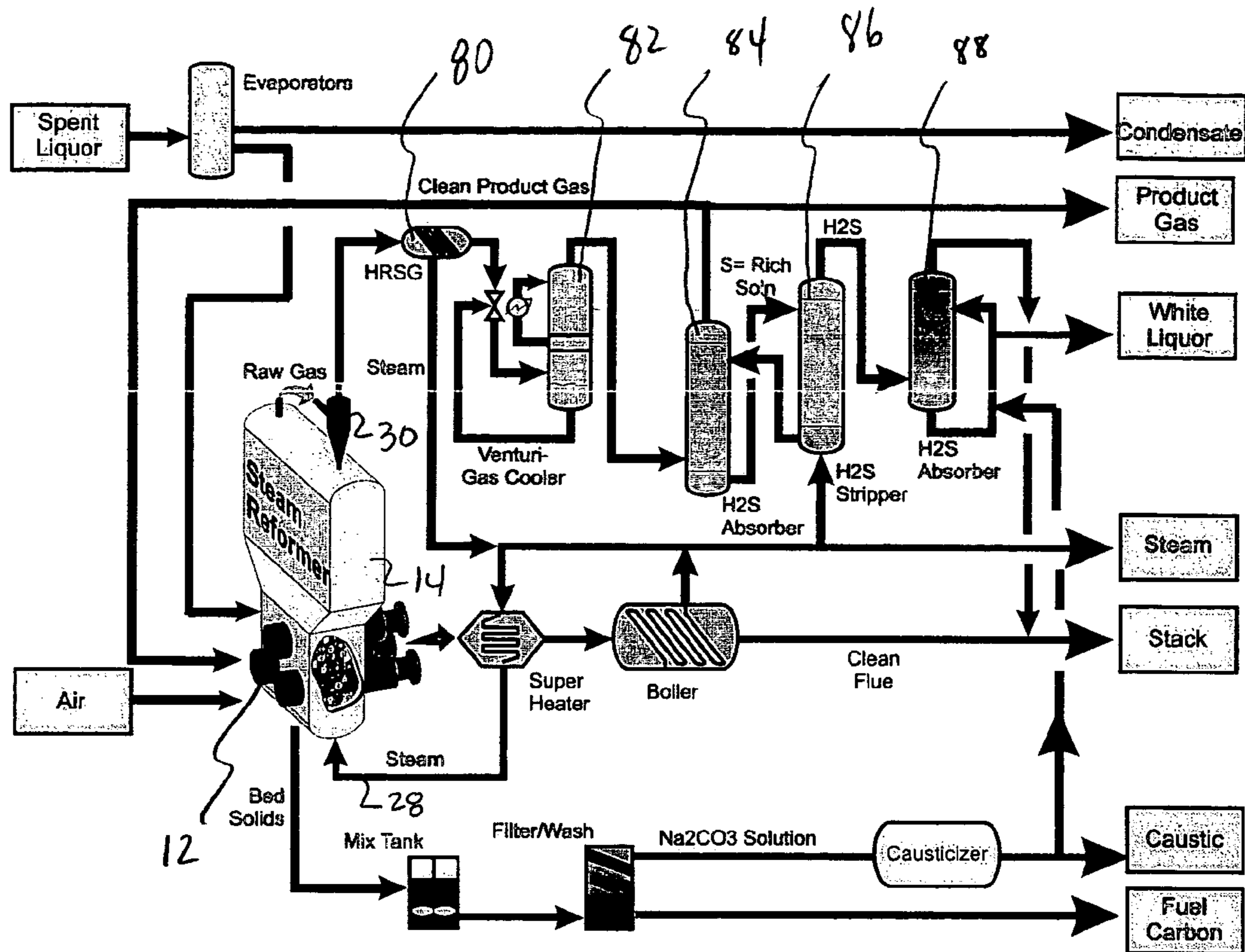
Figure 11 Steam Reformer Island
