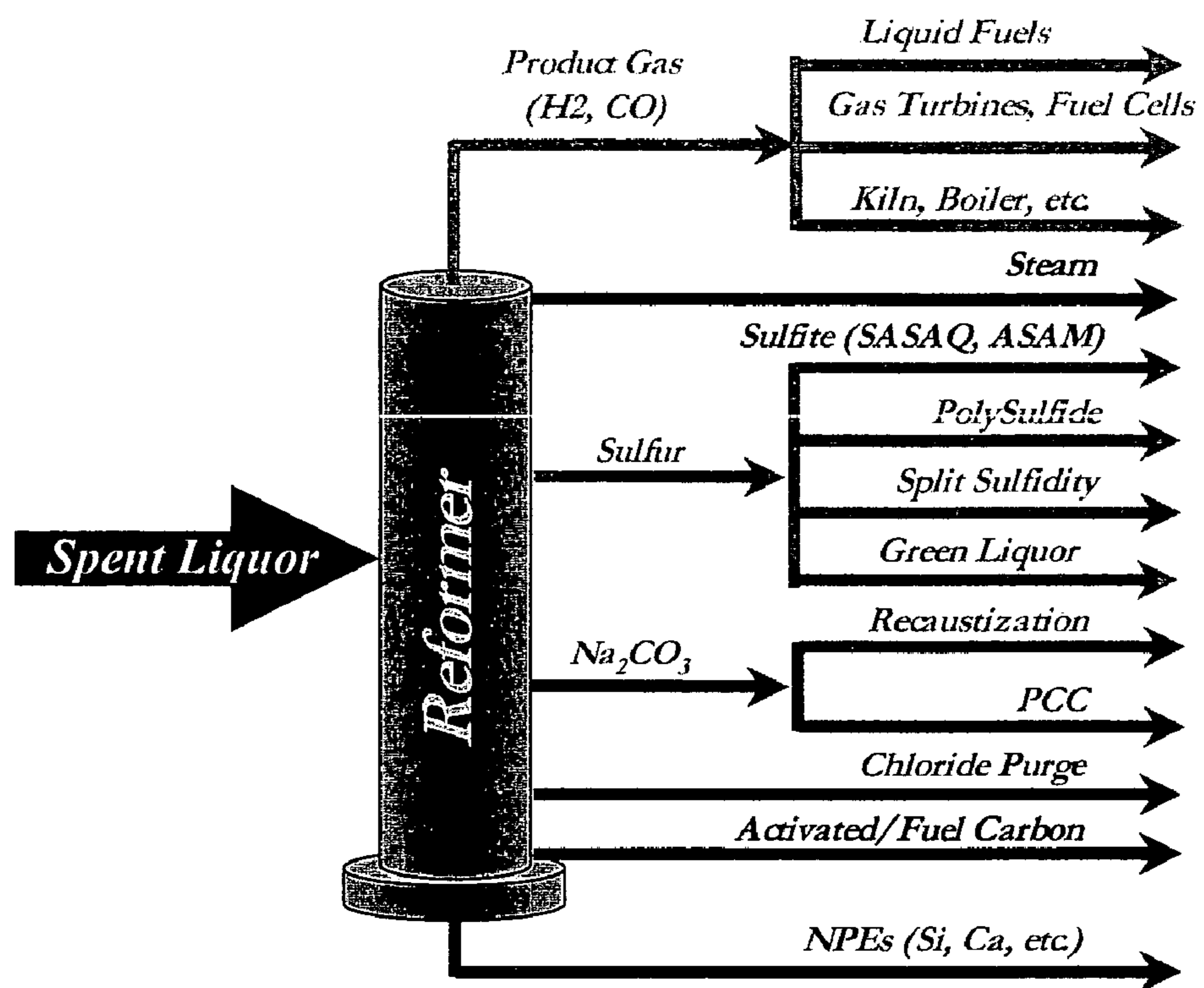
Figure 3. Spent Liquor Recovery Options
