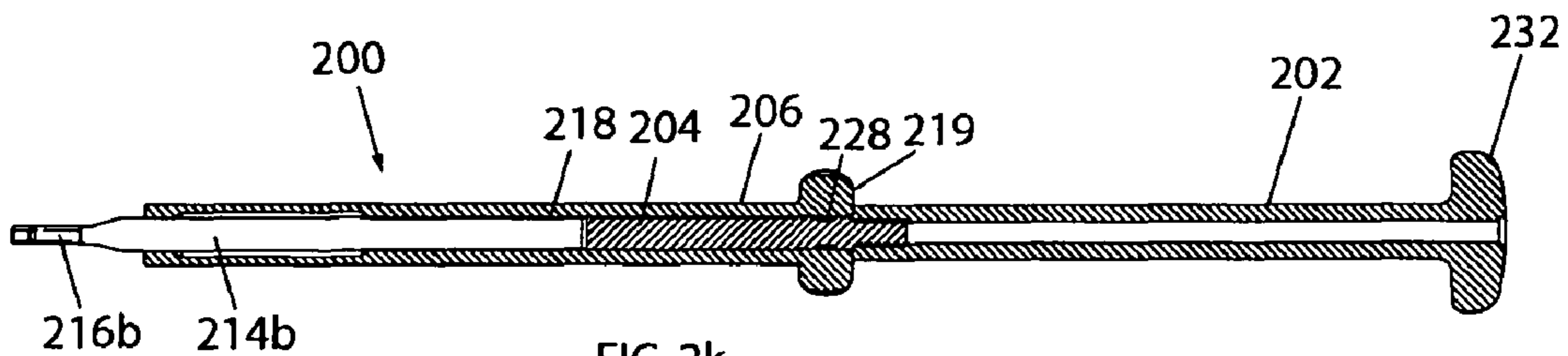
FIG. 2k (Section A-A of Fig. 2b)
