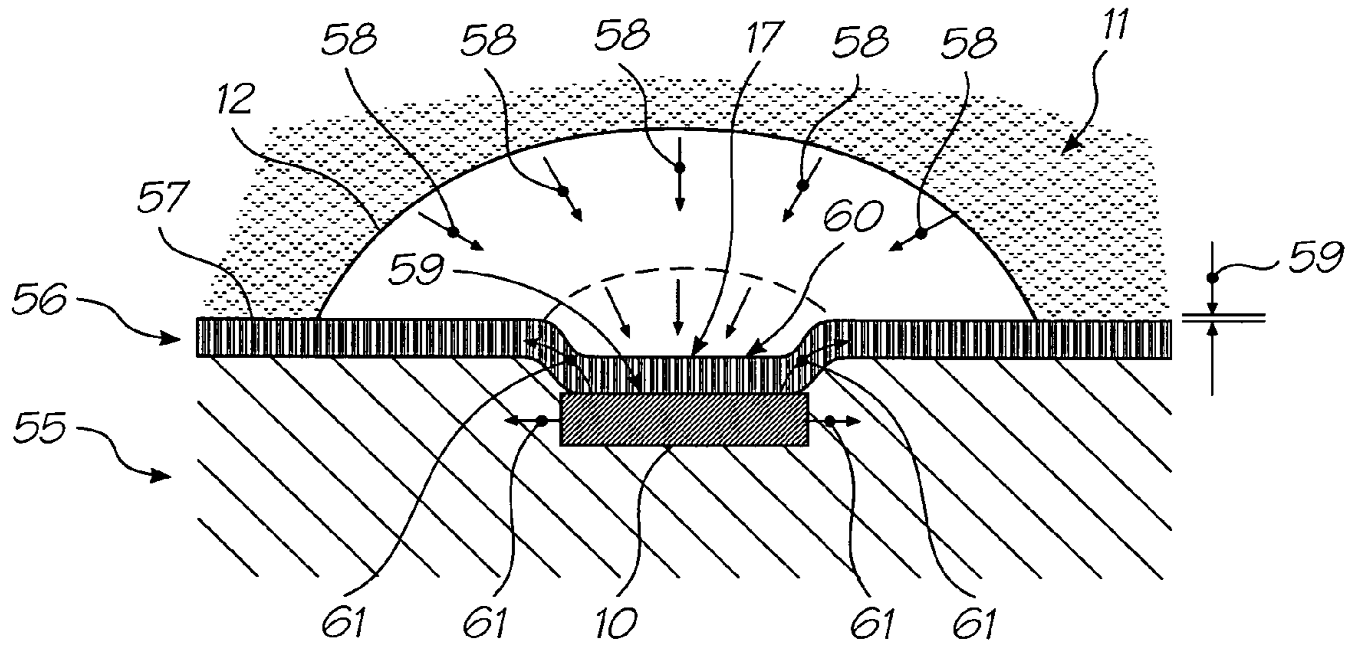
FIG. 47 (PRIOR ART)
