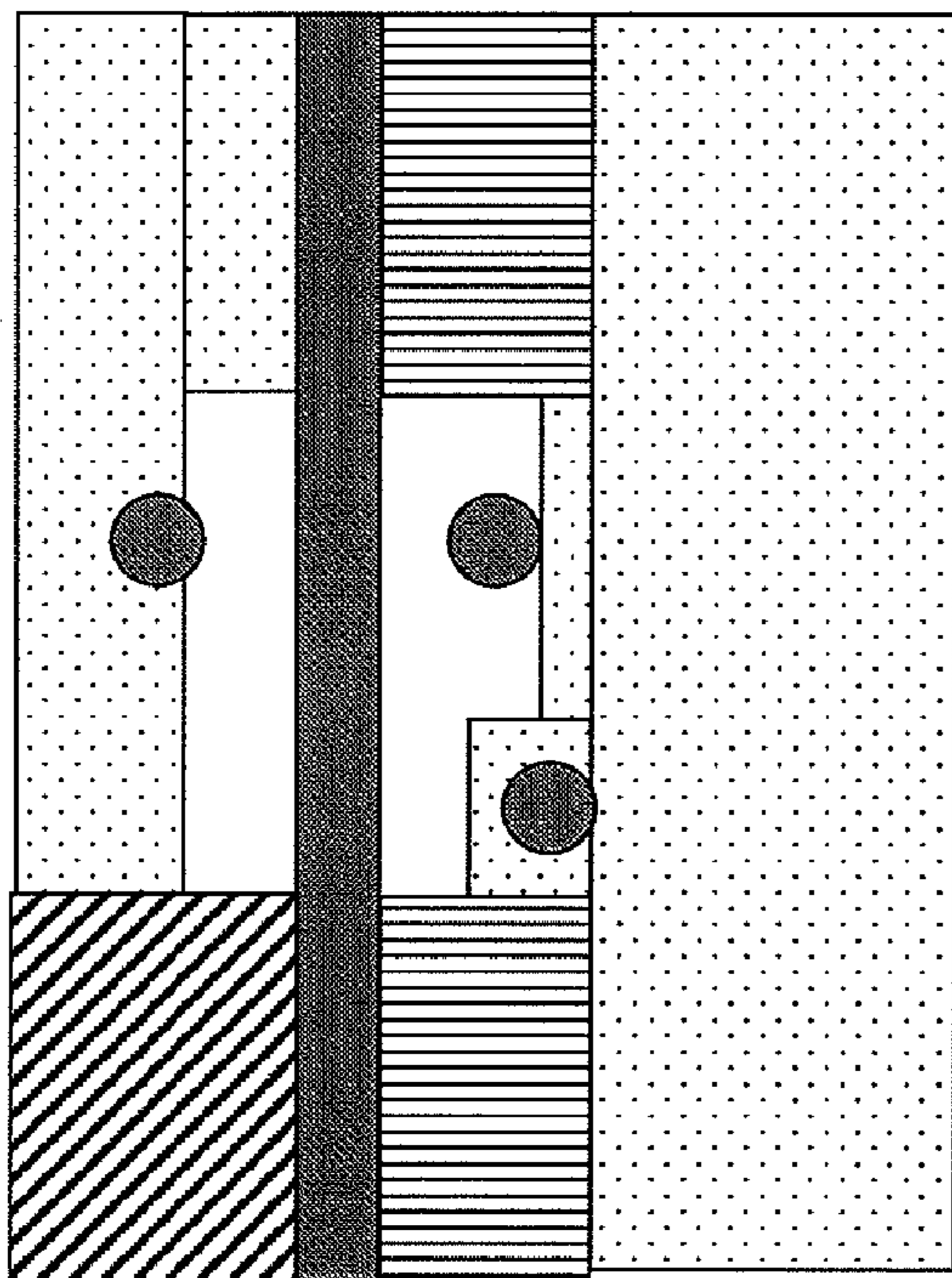
Figure 8A: NT Device Cross Section - SINGLE NANOTUBES
