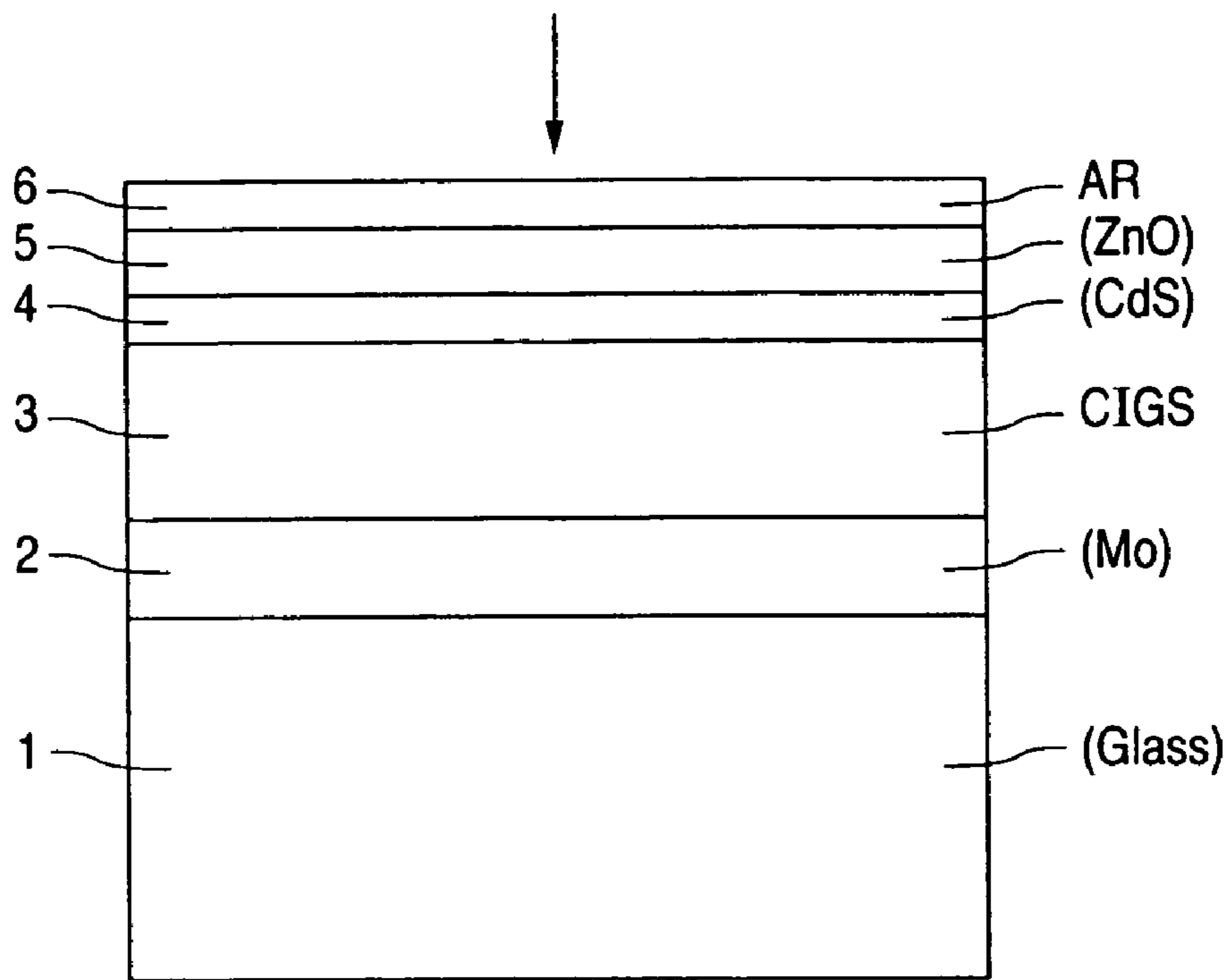
FIG. 1 (PRIOR ART)
