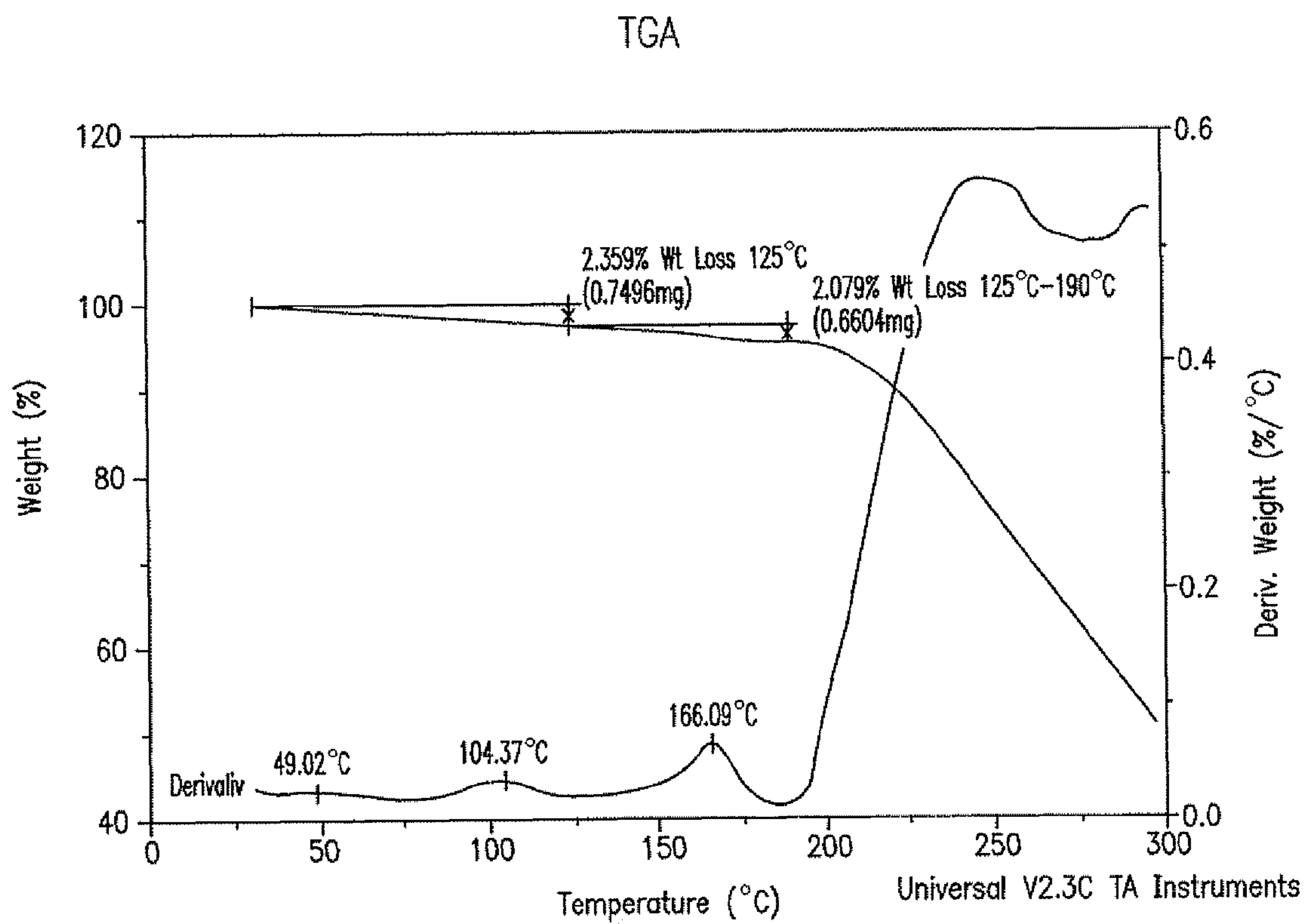
TGA Pattern C
