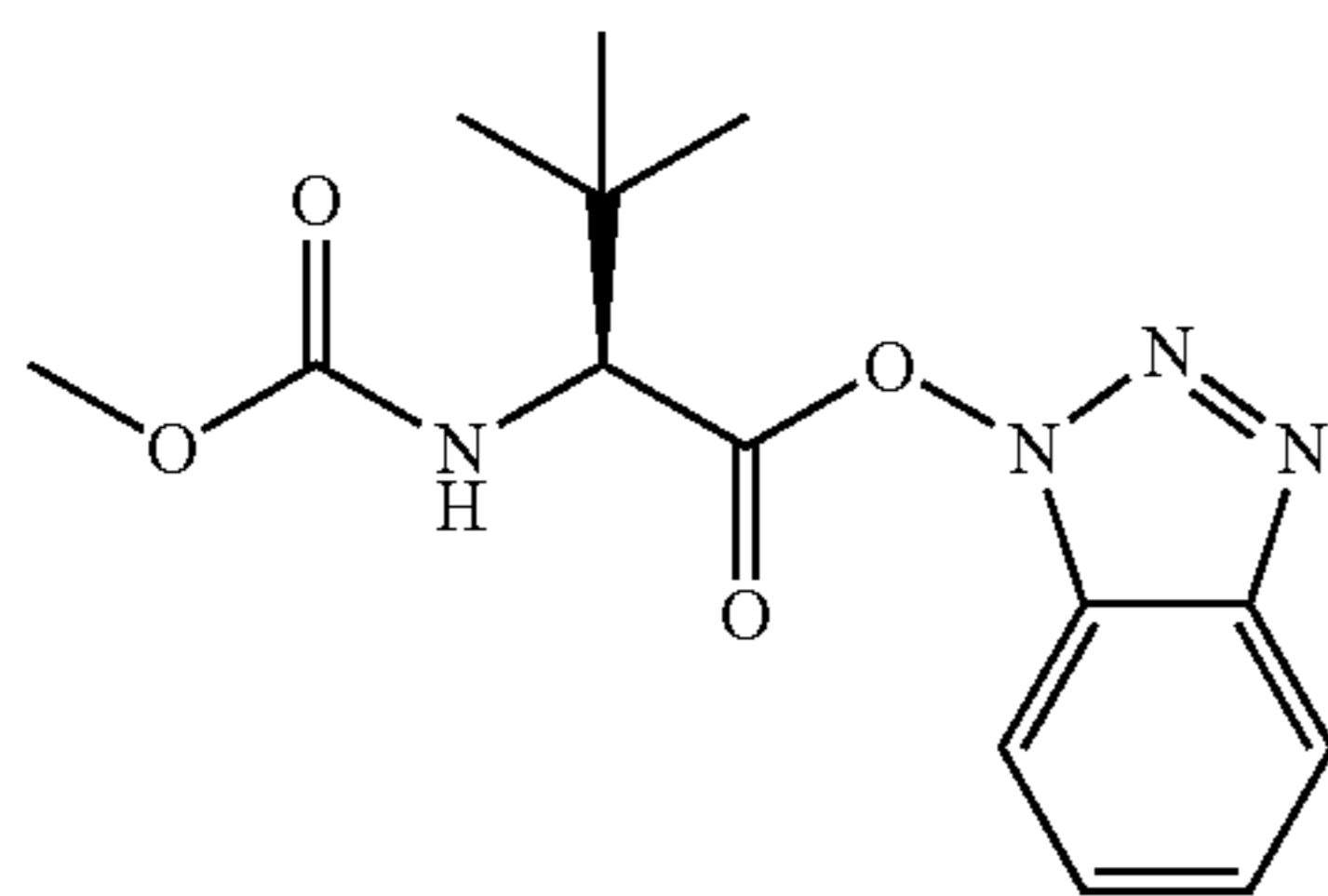
B. Active Ester of N-methoxycarbonyl-L-tert-leucine
