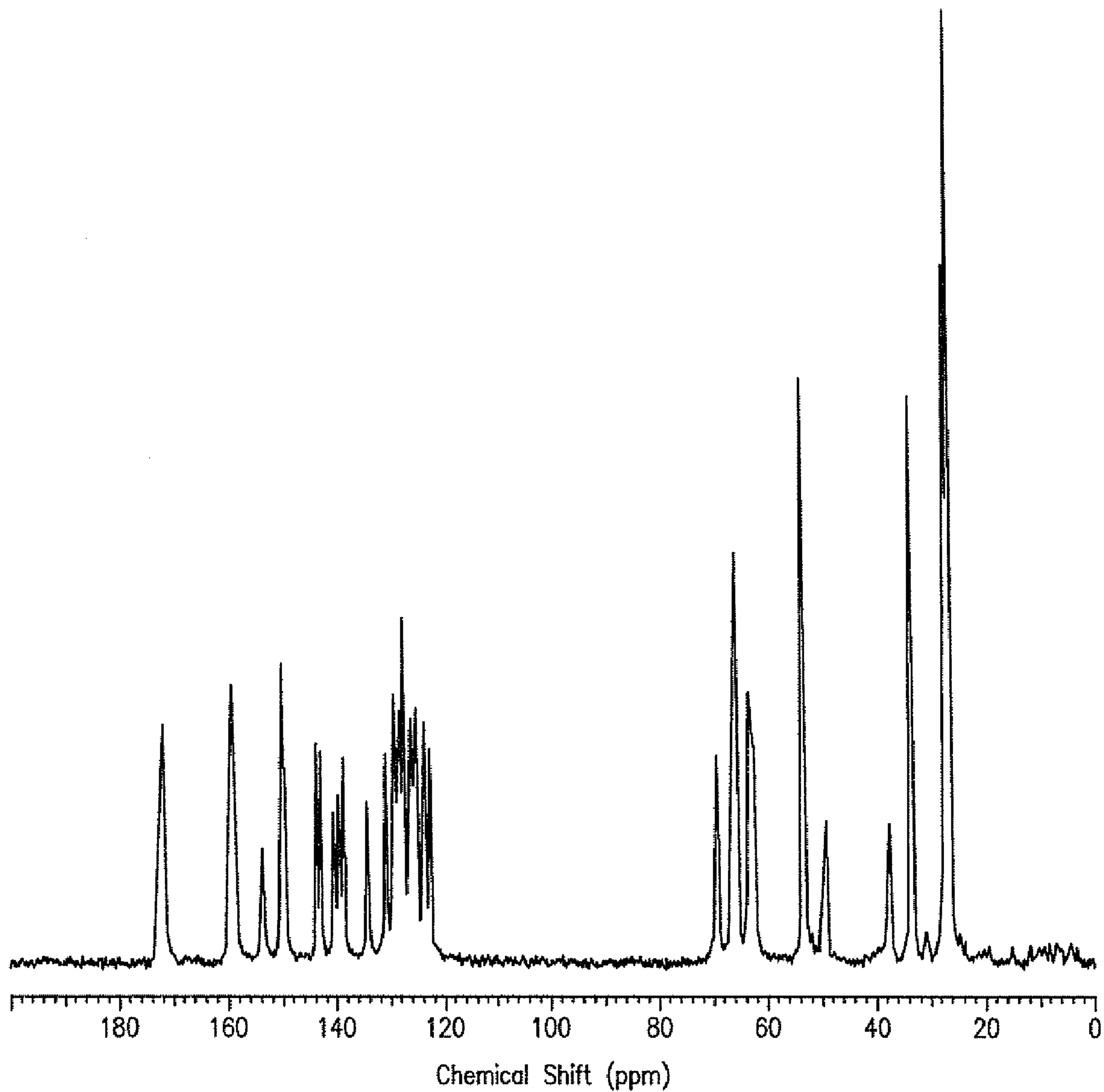
Carbon-13 SSNMR of Form A
