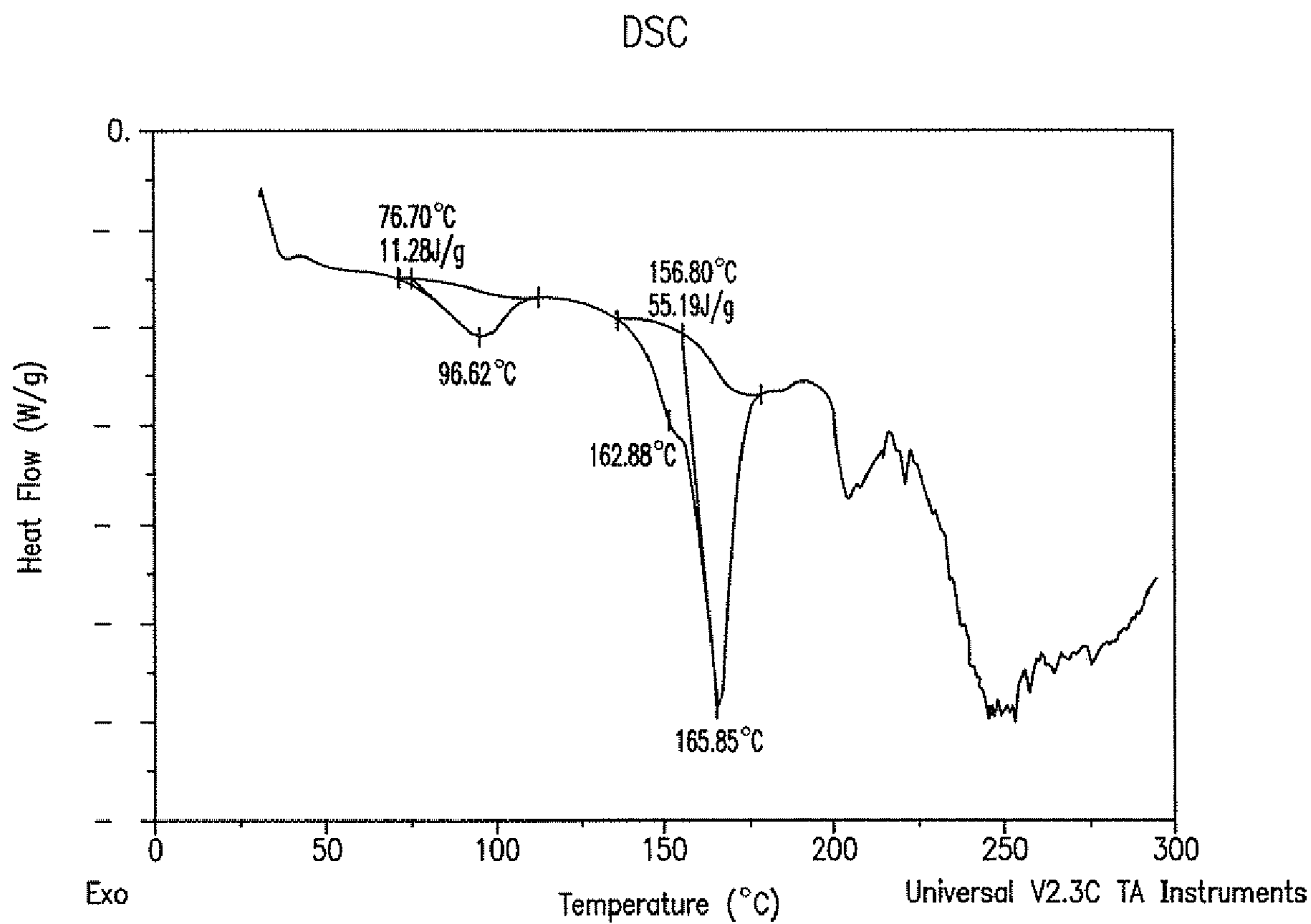
DSC Pattern C
