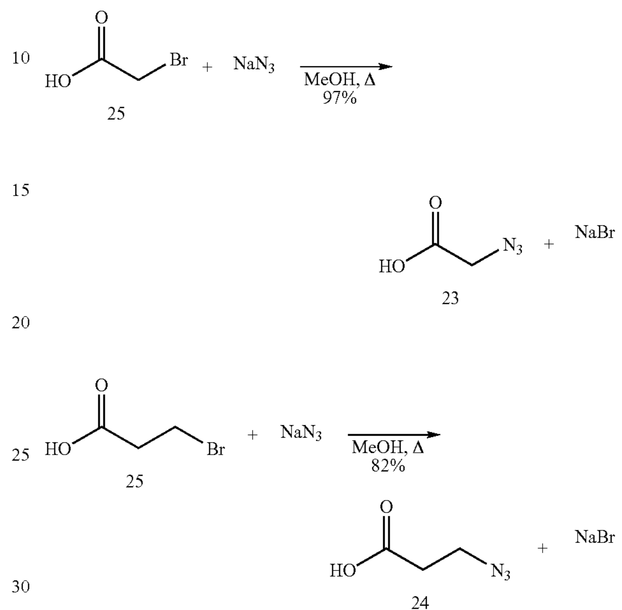
Scheme 6
