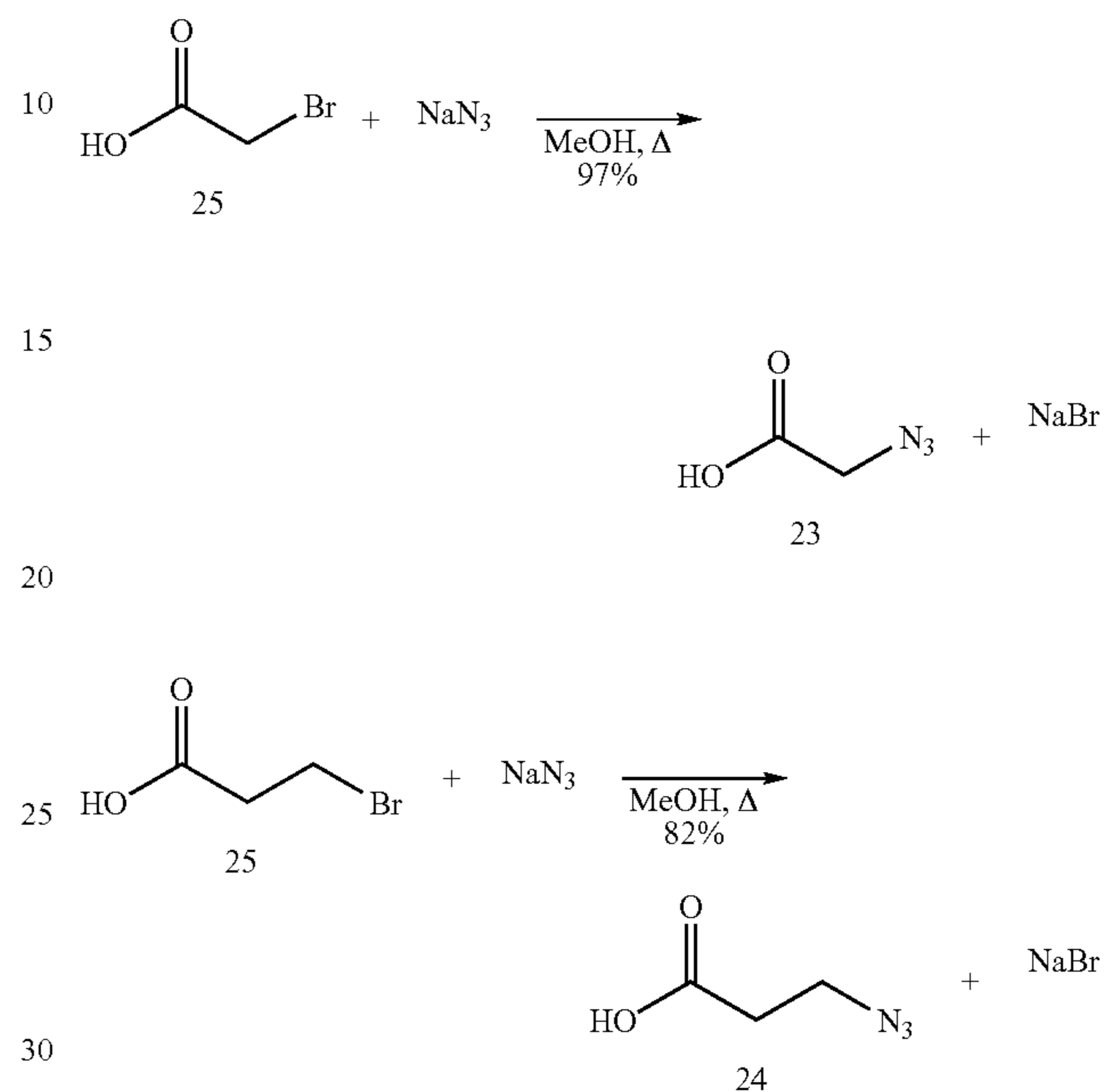
Scheme 6
