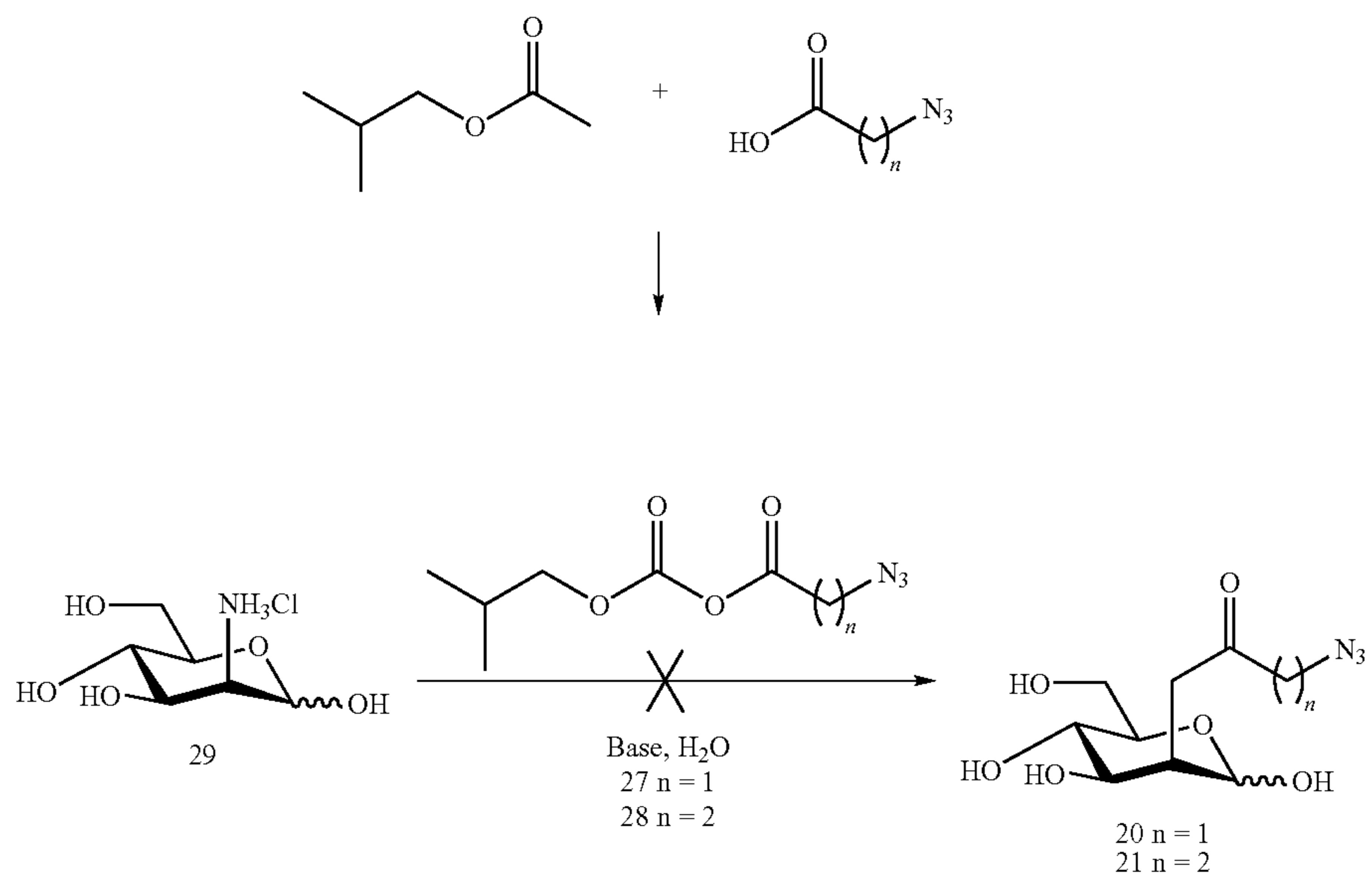
Scheme 7
