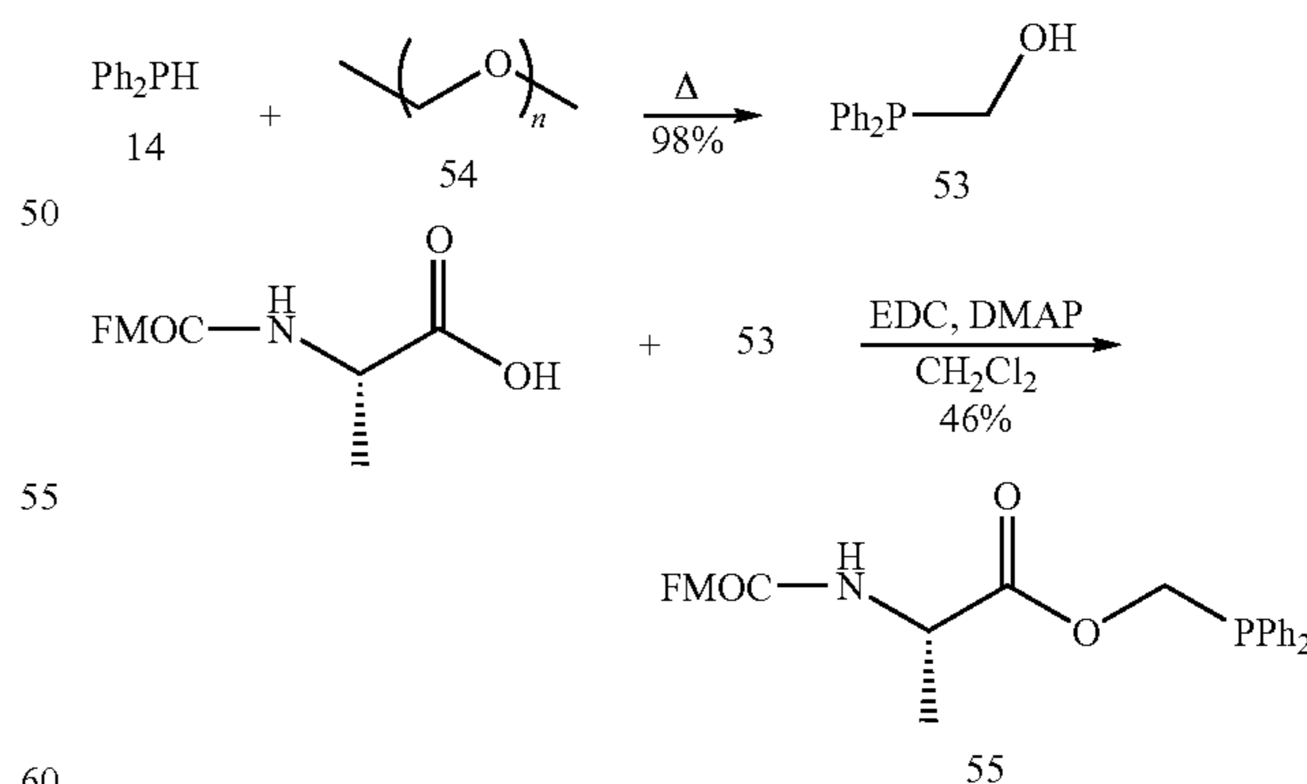
Scheme 16
