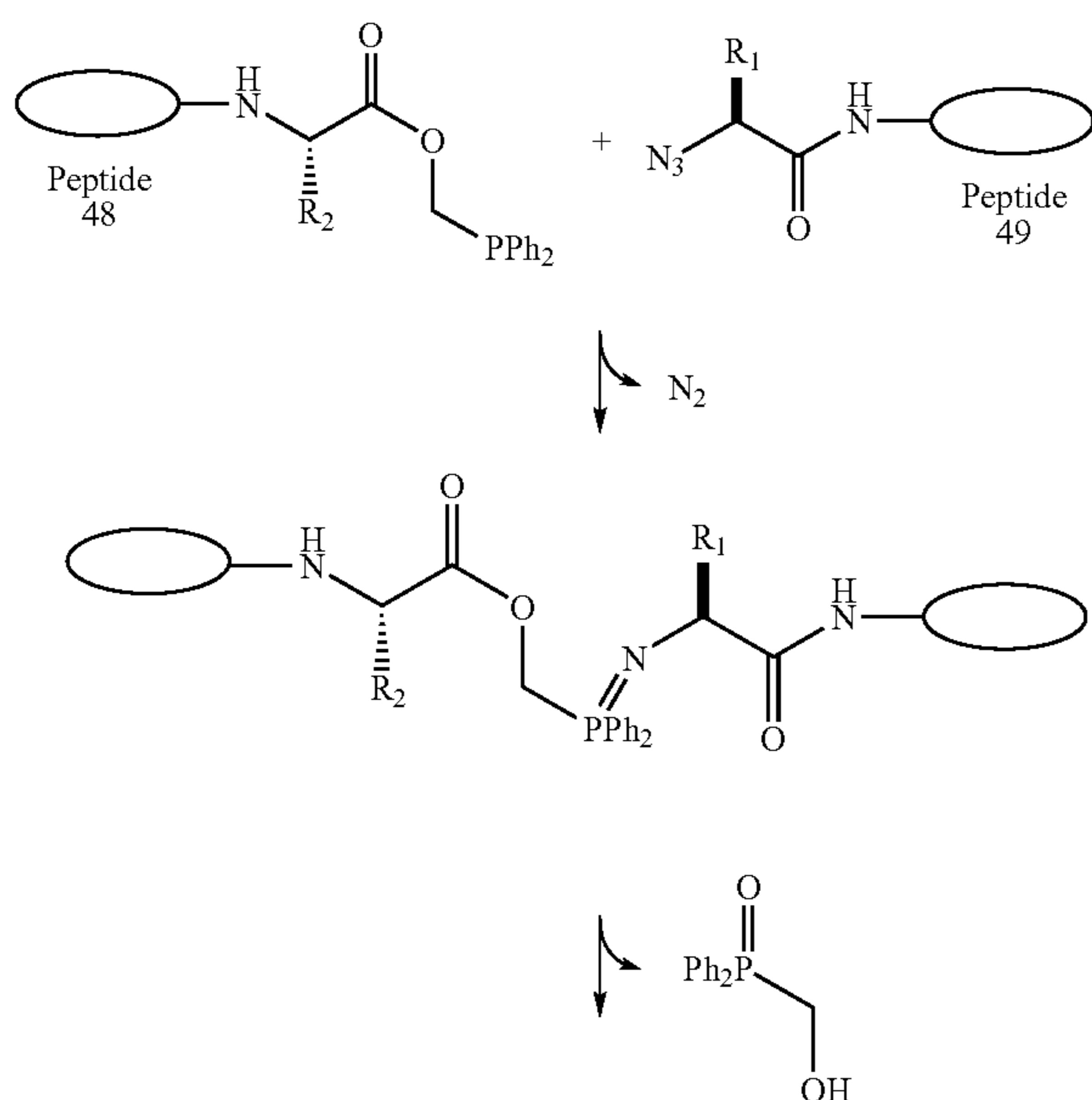
Scheme 14
