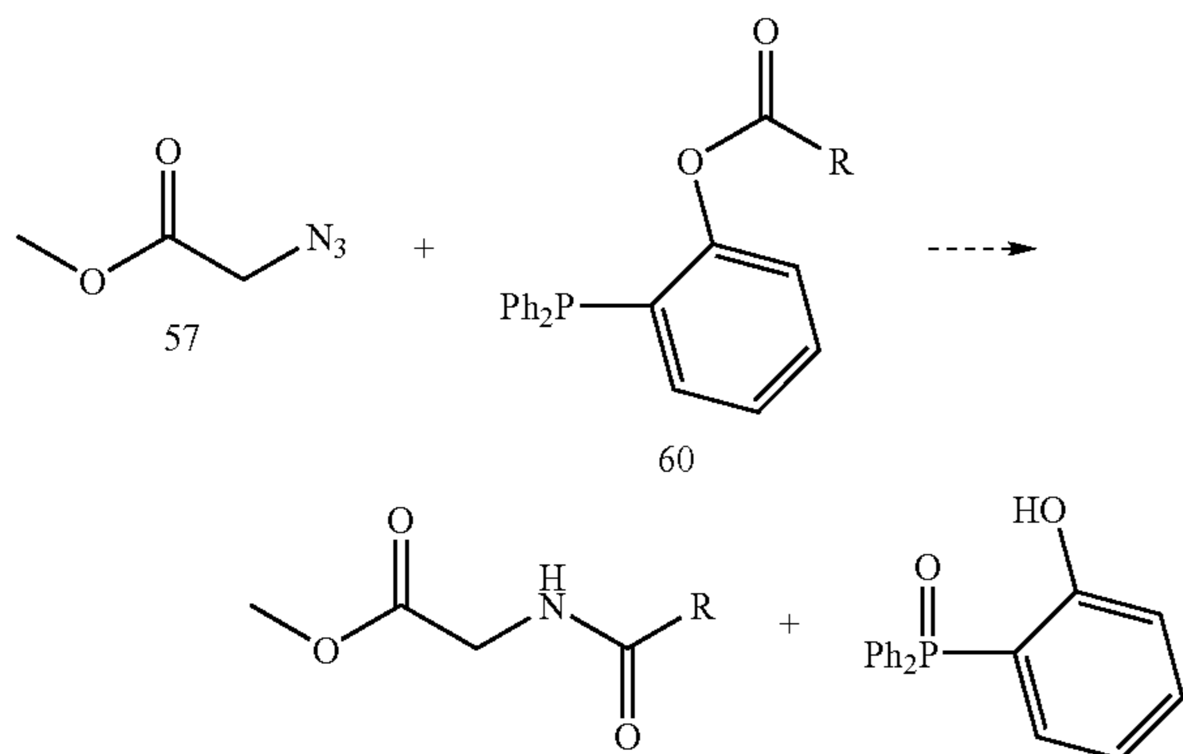
Scheme 18
