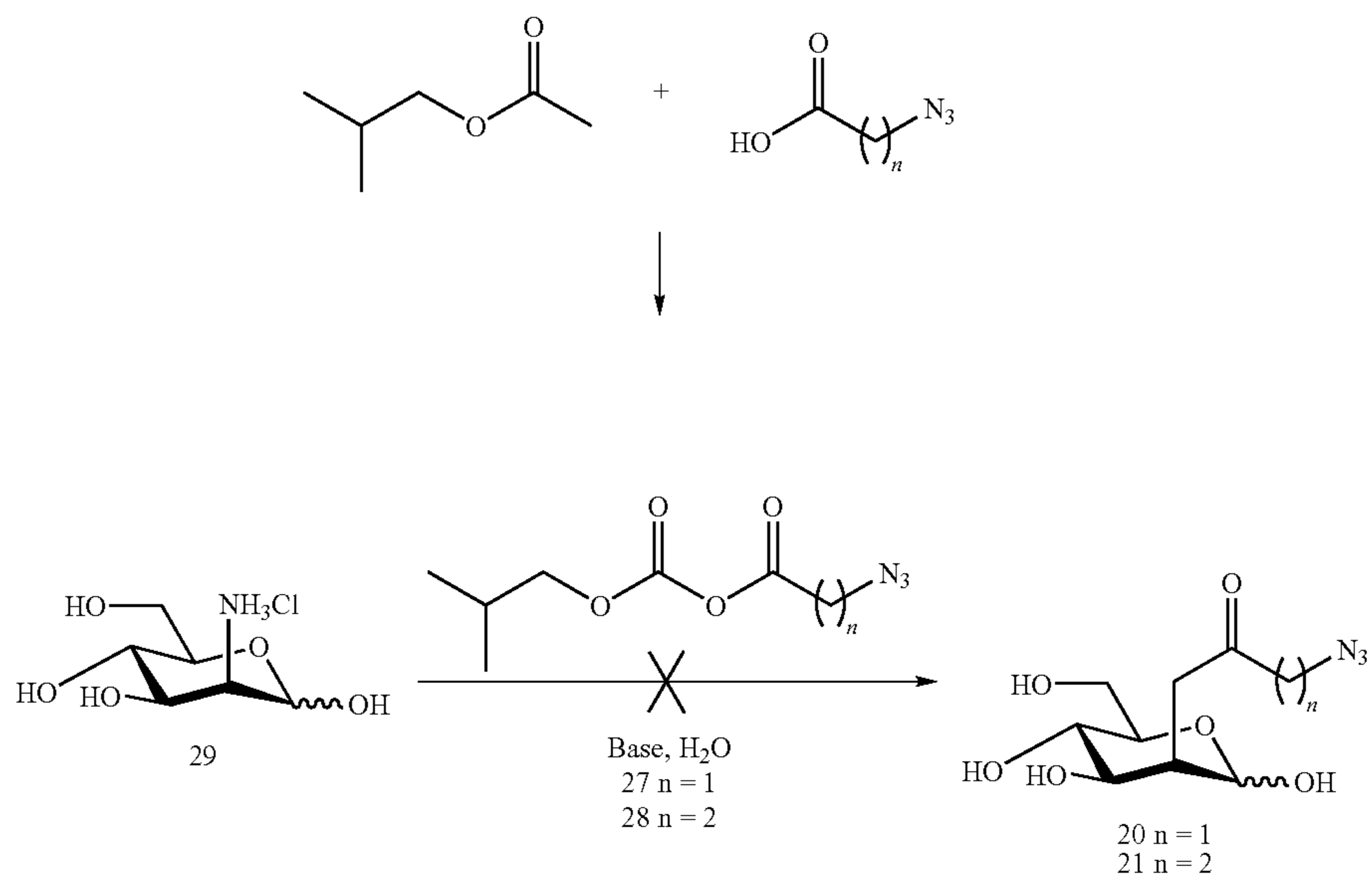
Scheme 7
