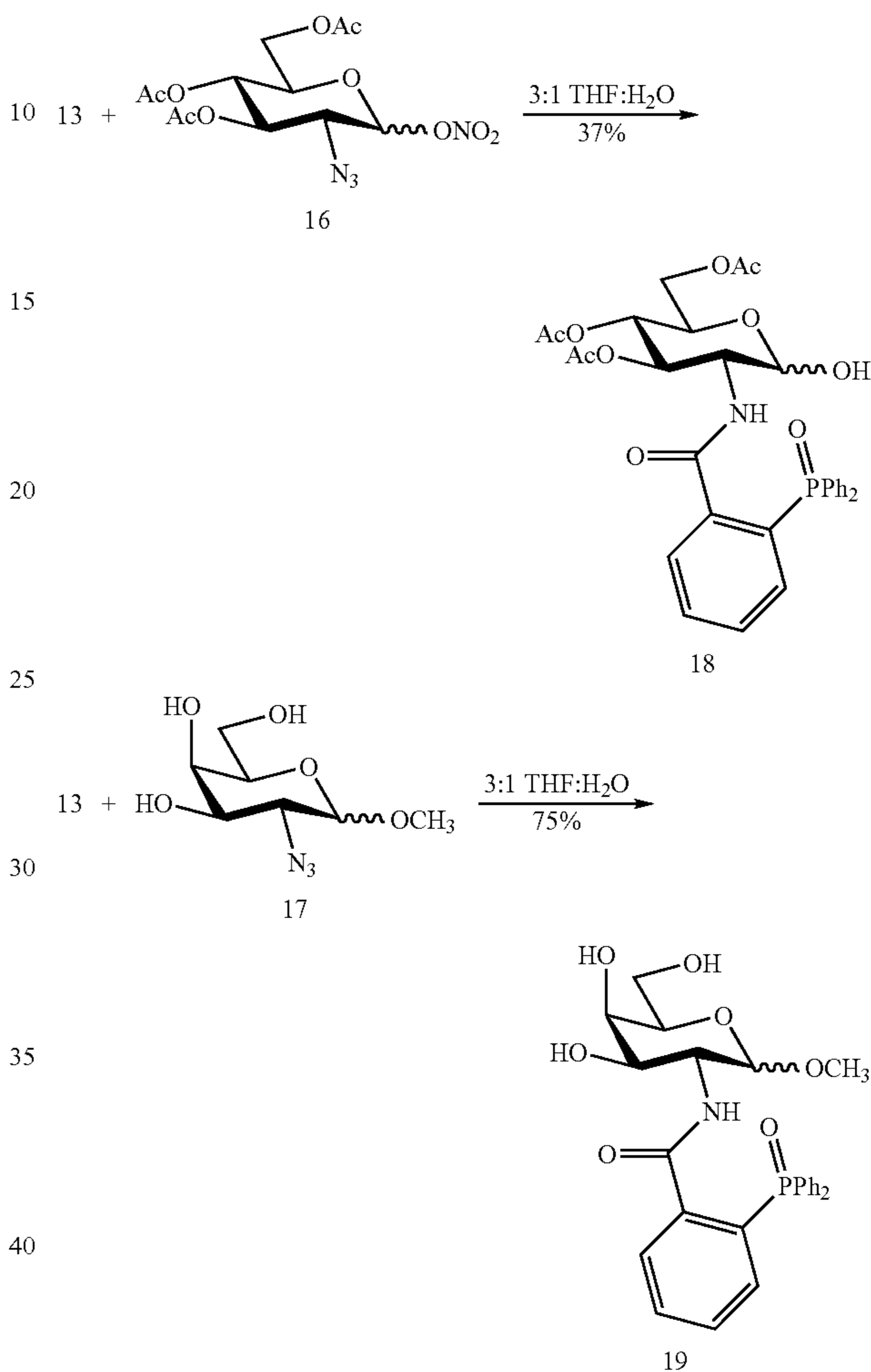
Scheme 5
