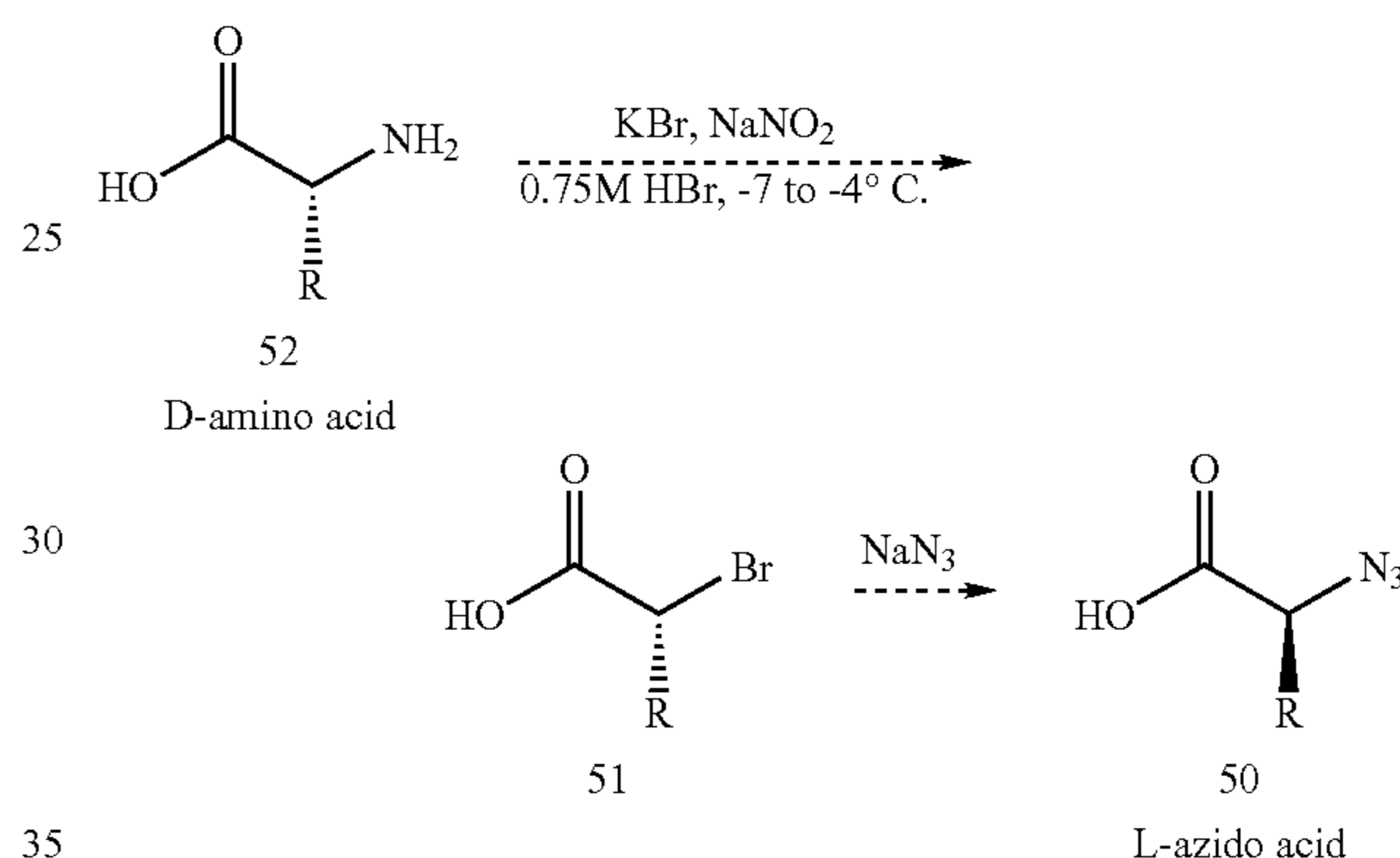
Scheme 15
