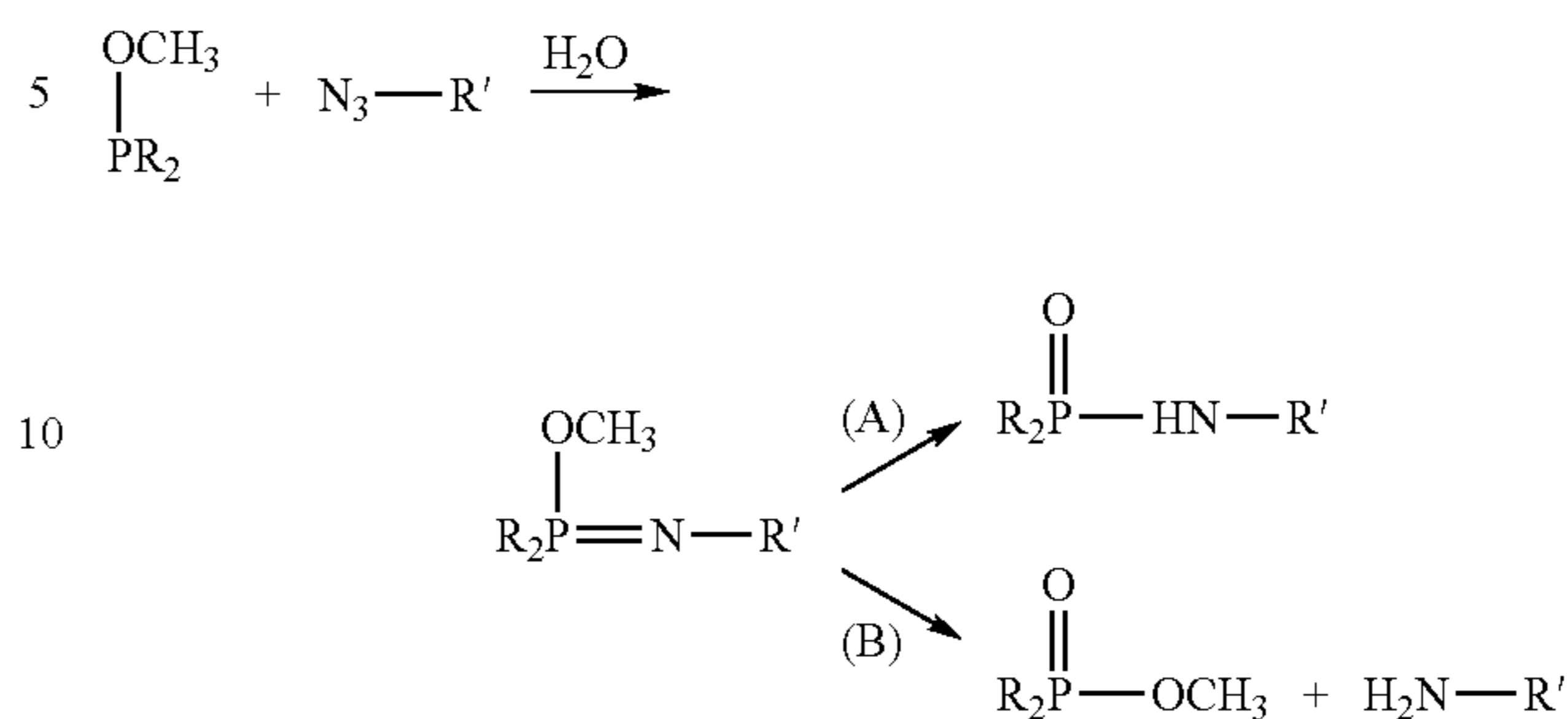
Scheme 1
