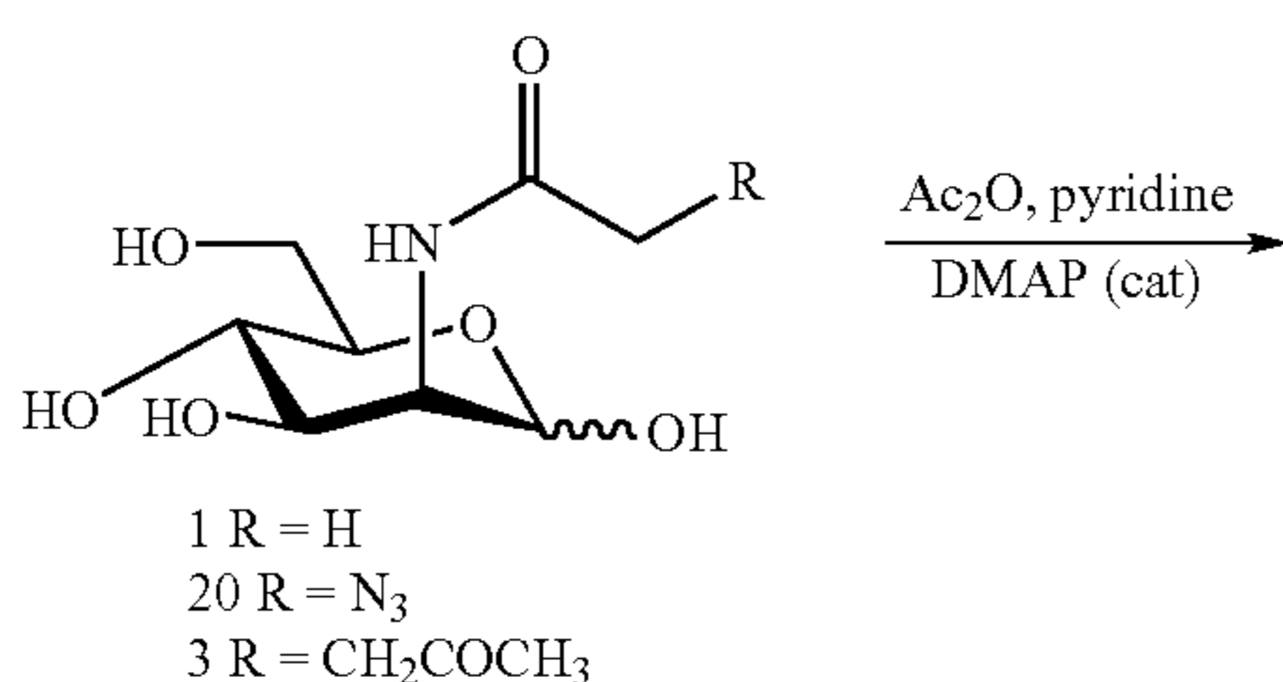
Scheme 11
