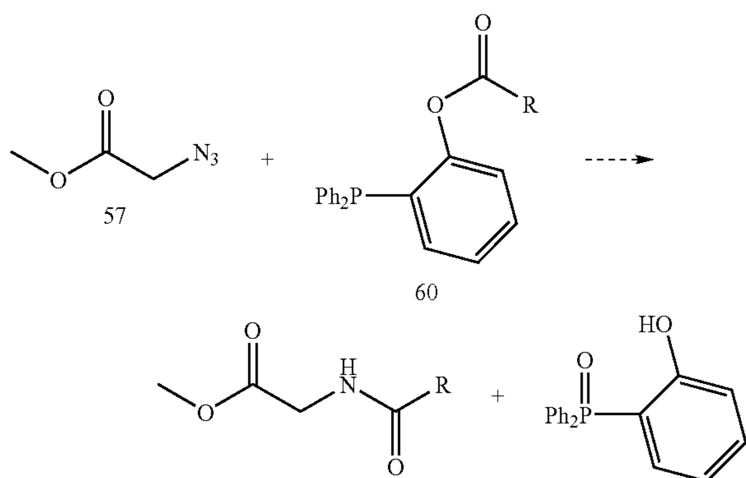
Scheme 18
