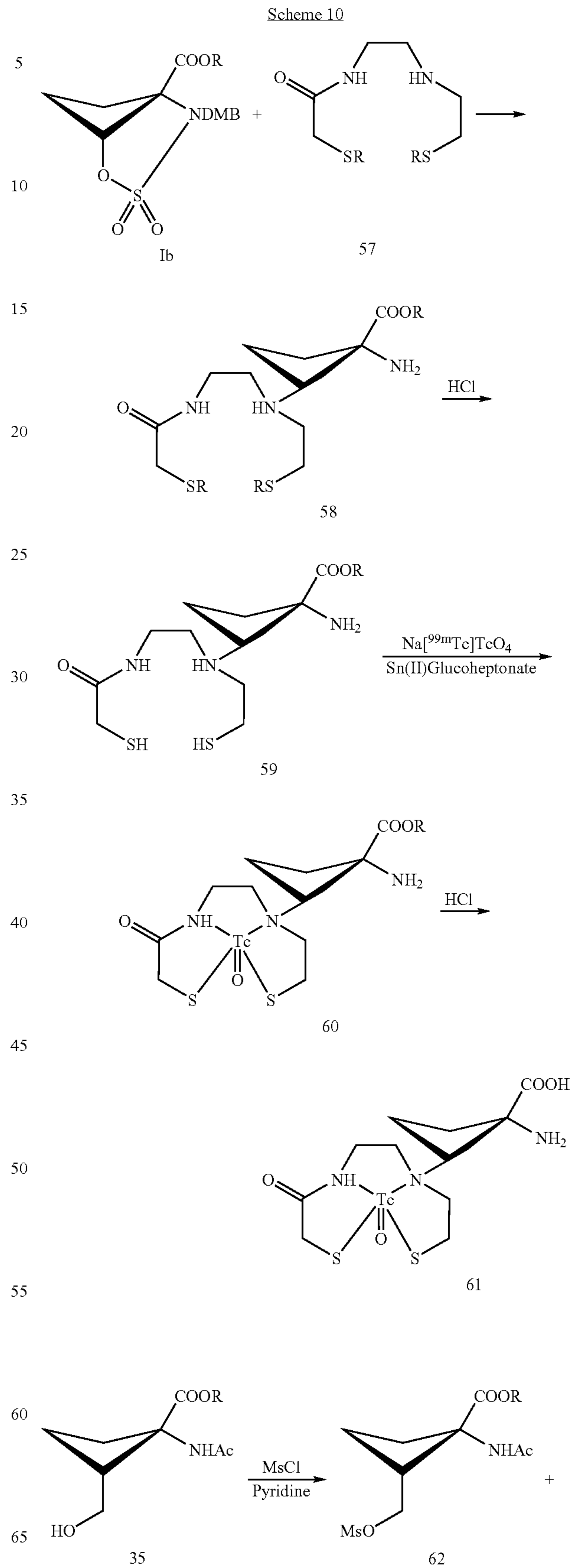
Schemes 10 and 11 depict synthetic routes for 2-substituted Tc-99m derivatives of the present invention.
