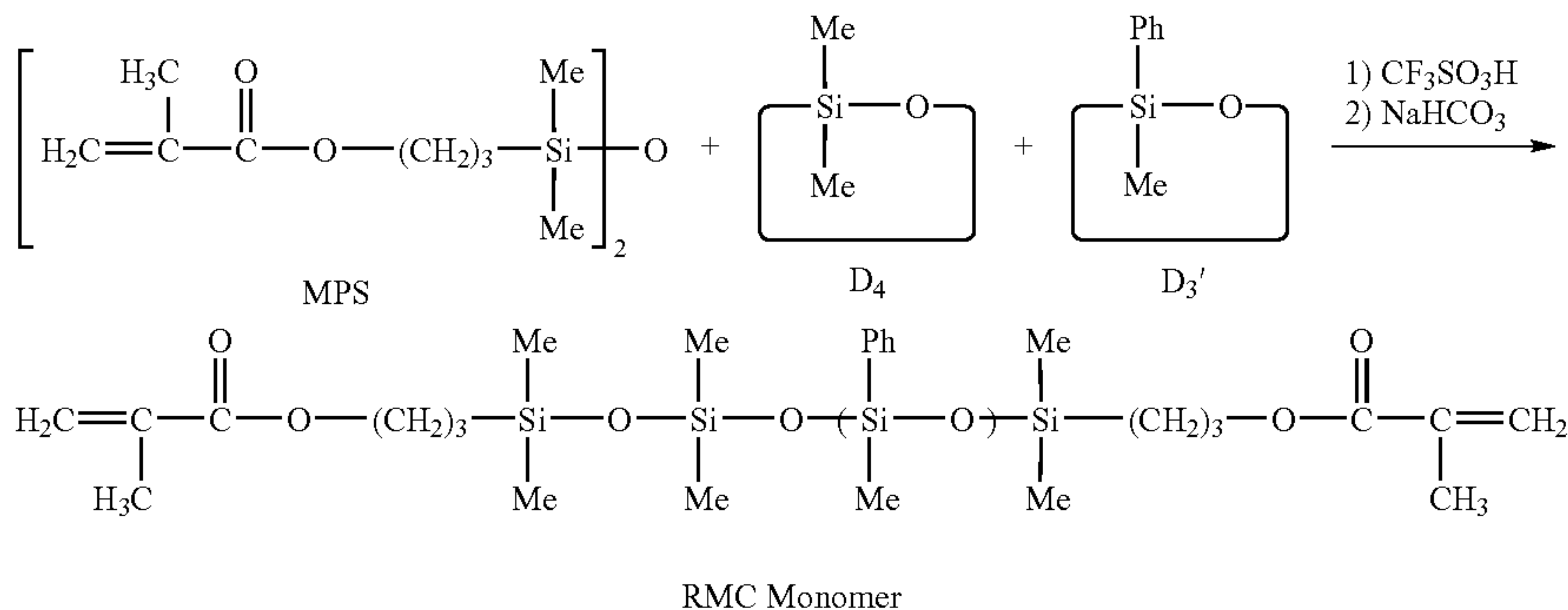
SCHEME 1
