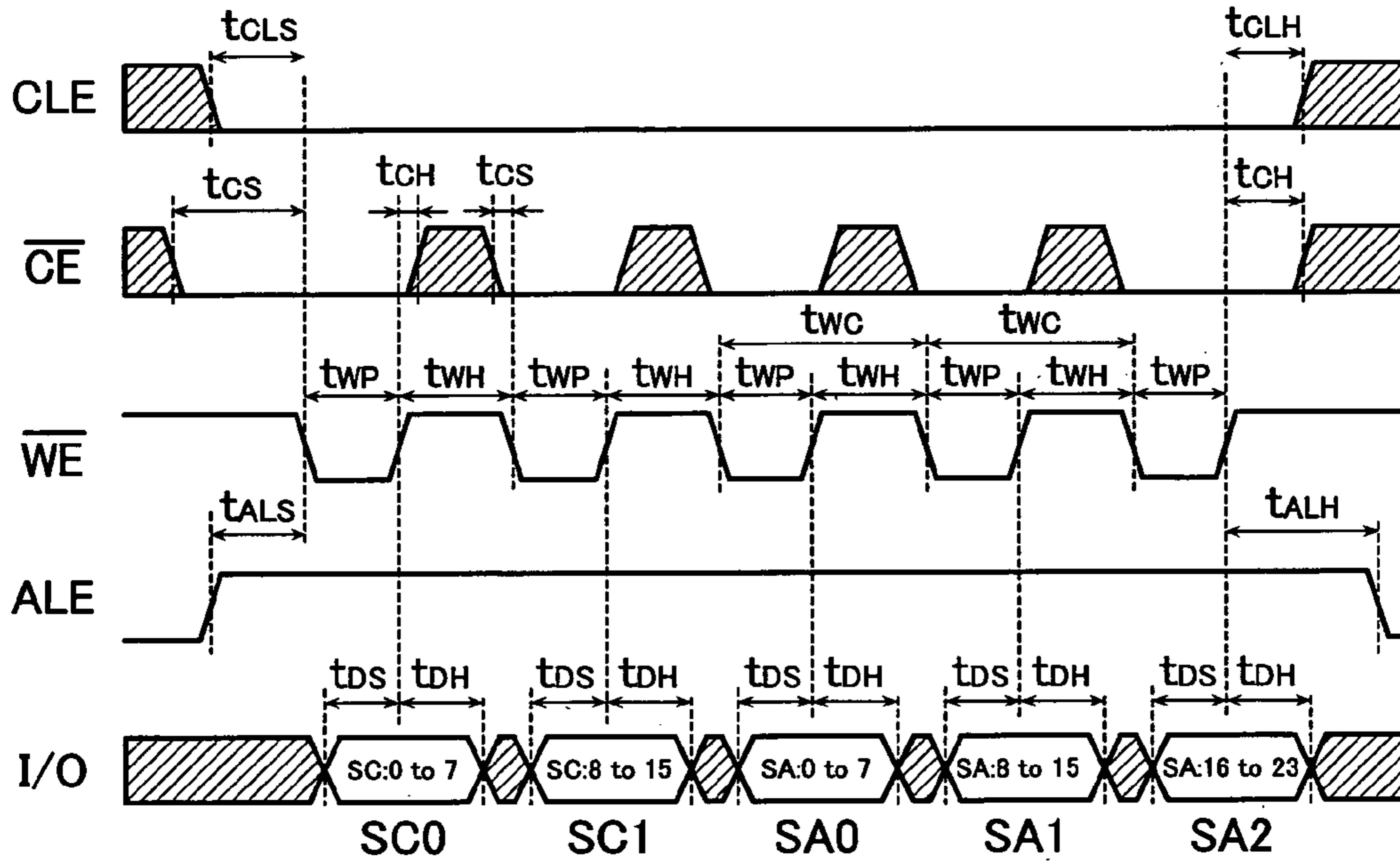
Address Input Cycle Timing Diagram
