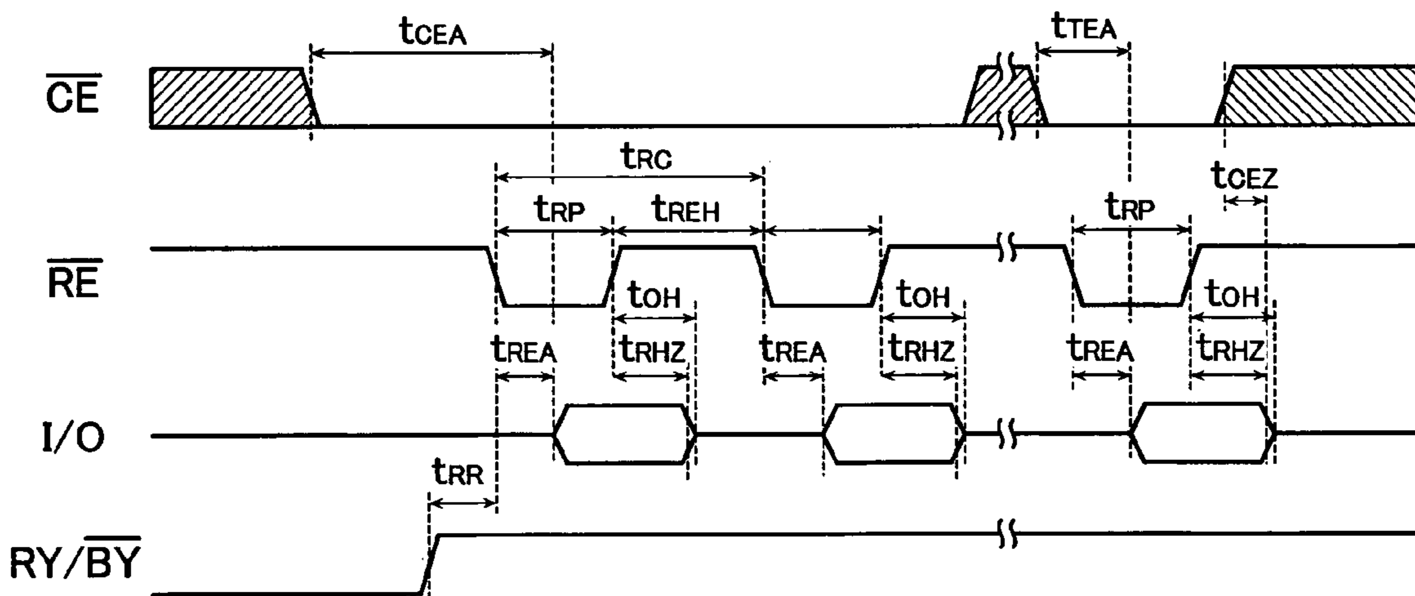
Serial Read Cycle Timing Diagram
