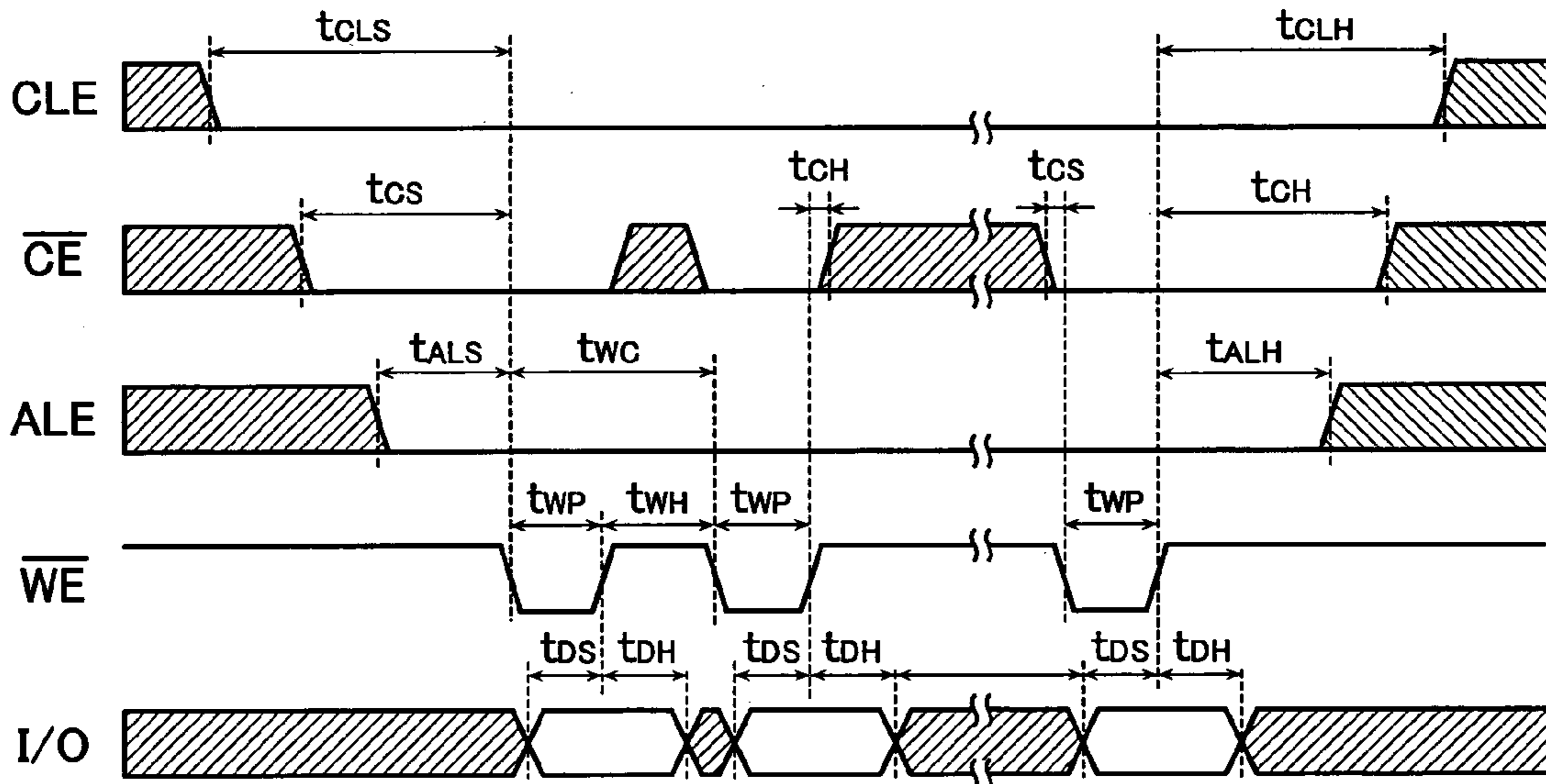
Data Input Cycle Timing Diagram
