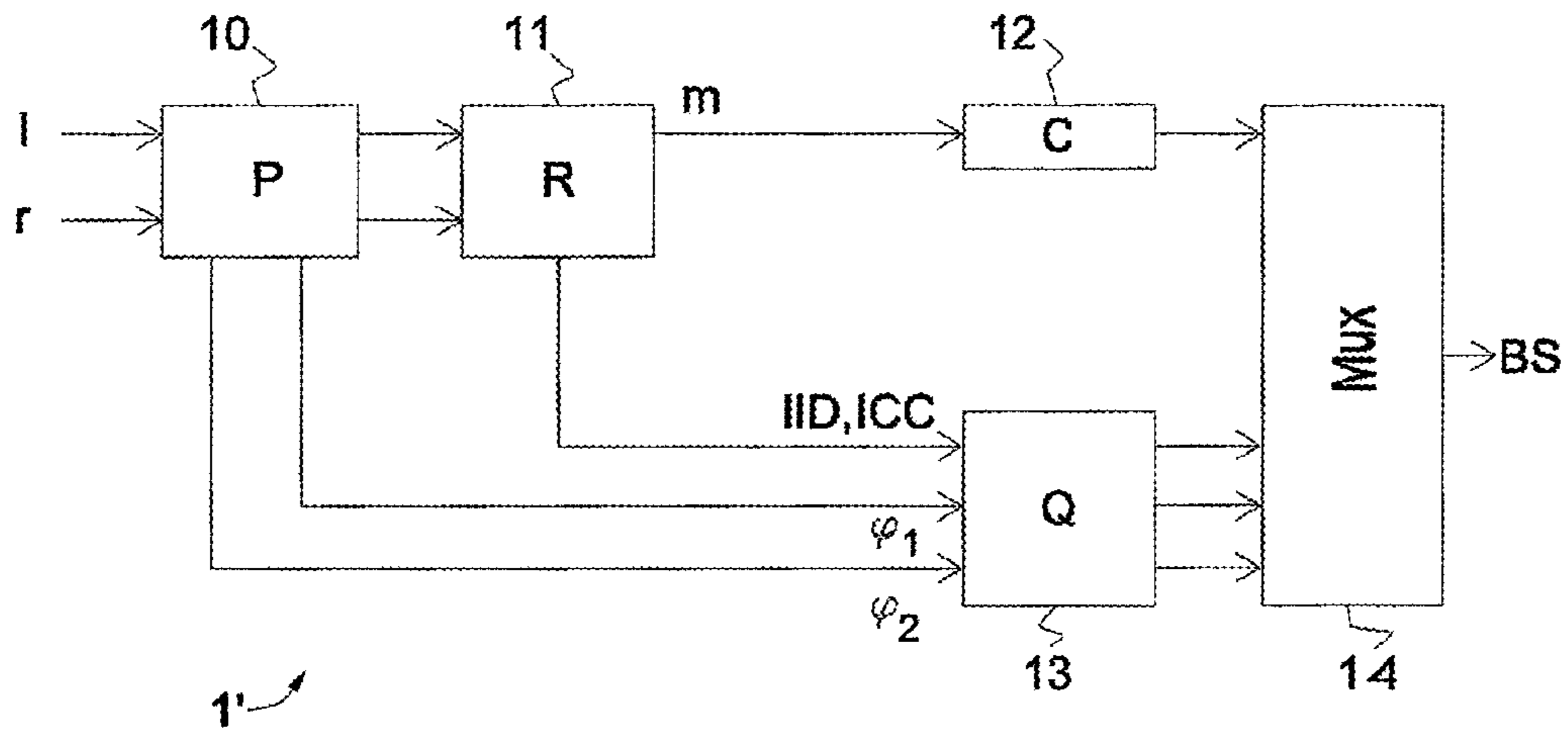
FIG. 1 PRIOR ART
