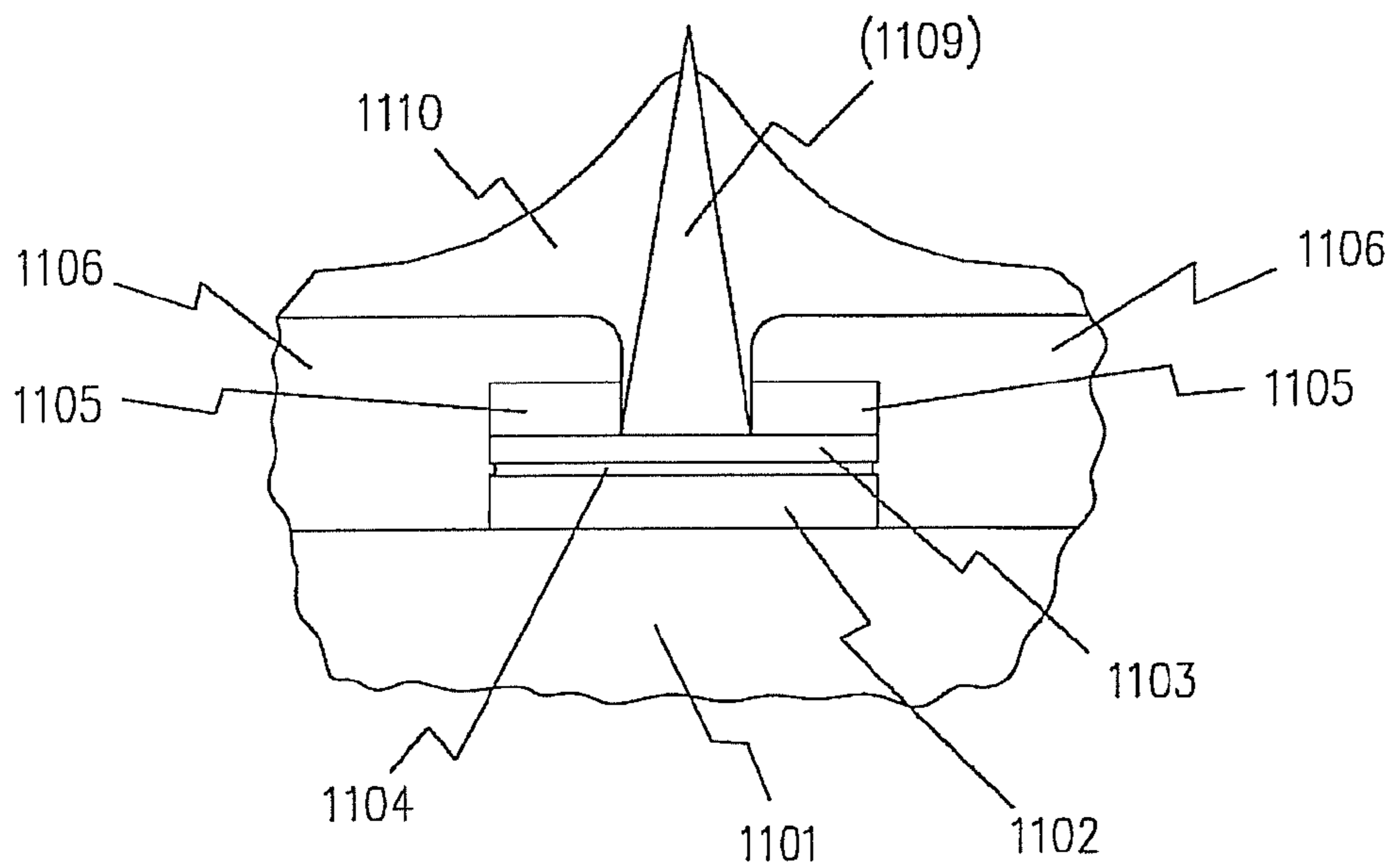
FIGURE 11b ELECTRODES
