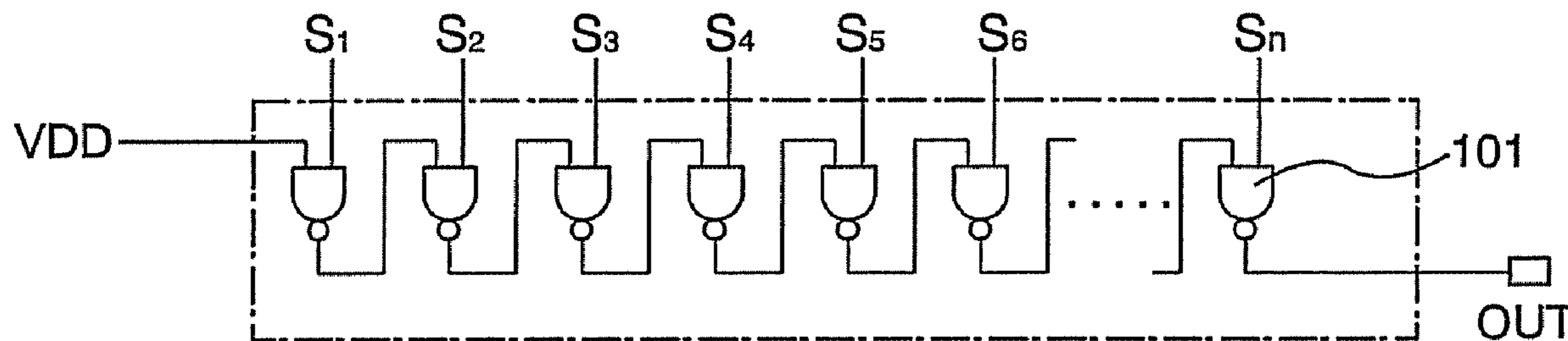
TESTING CIRCUIT
