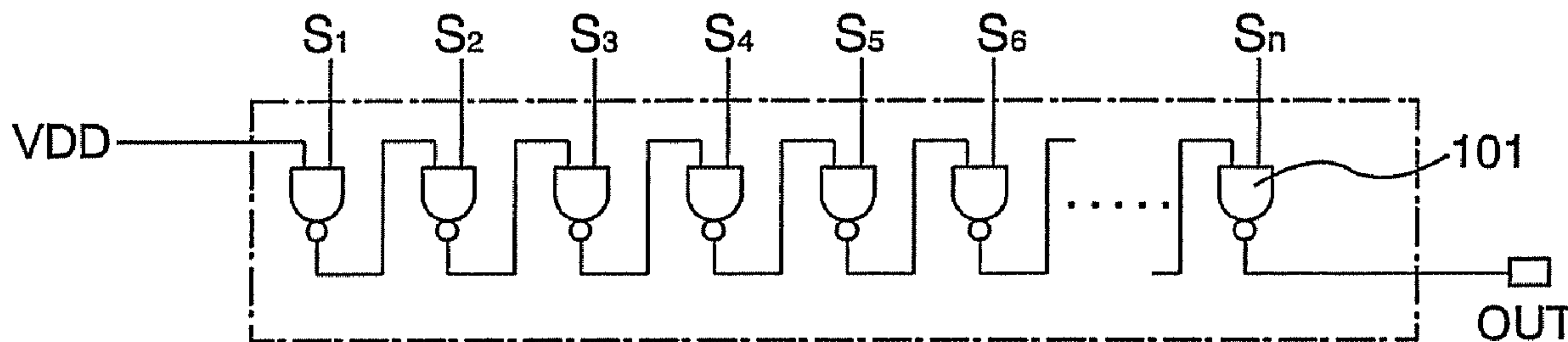
TESTING CIRCUIT
