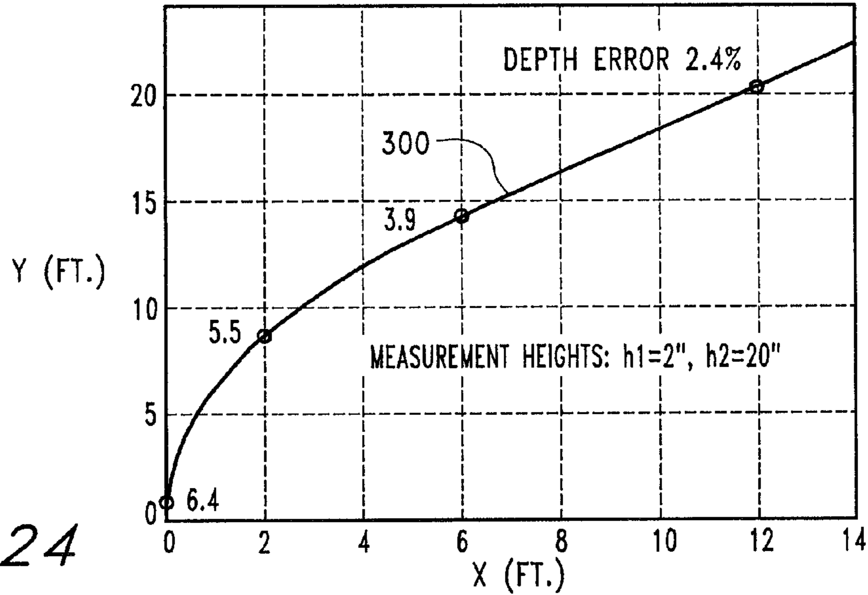
CABLE DEPTH FROM 2-POINT HEIGHT MEASUREMENTS, 5 FT. DEPTH
