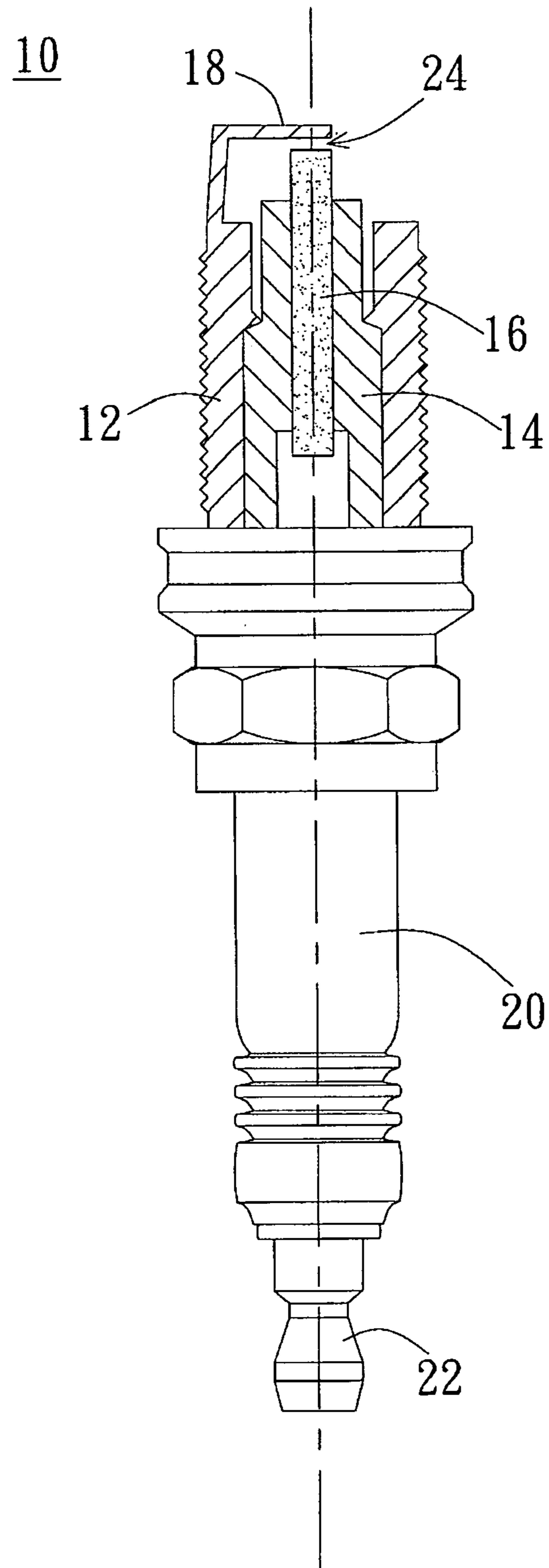
Fig. 1 (PRIOR ART)
