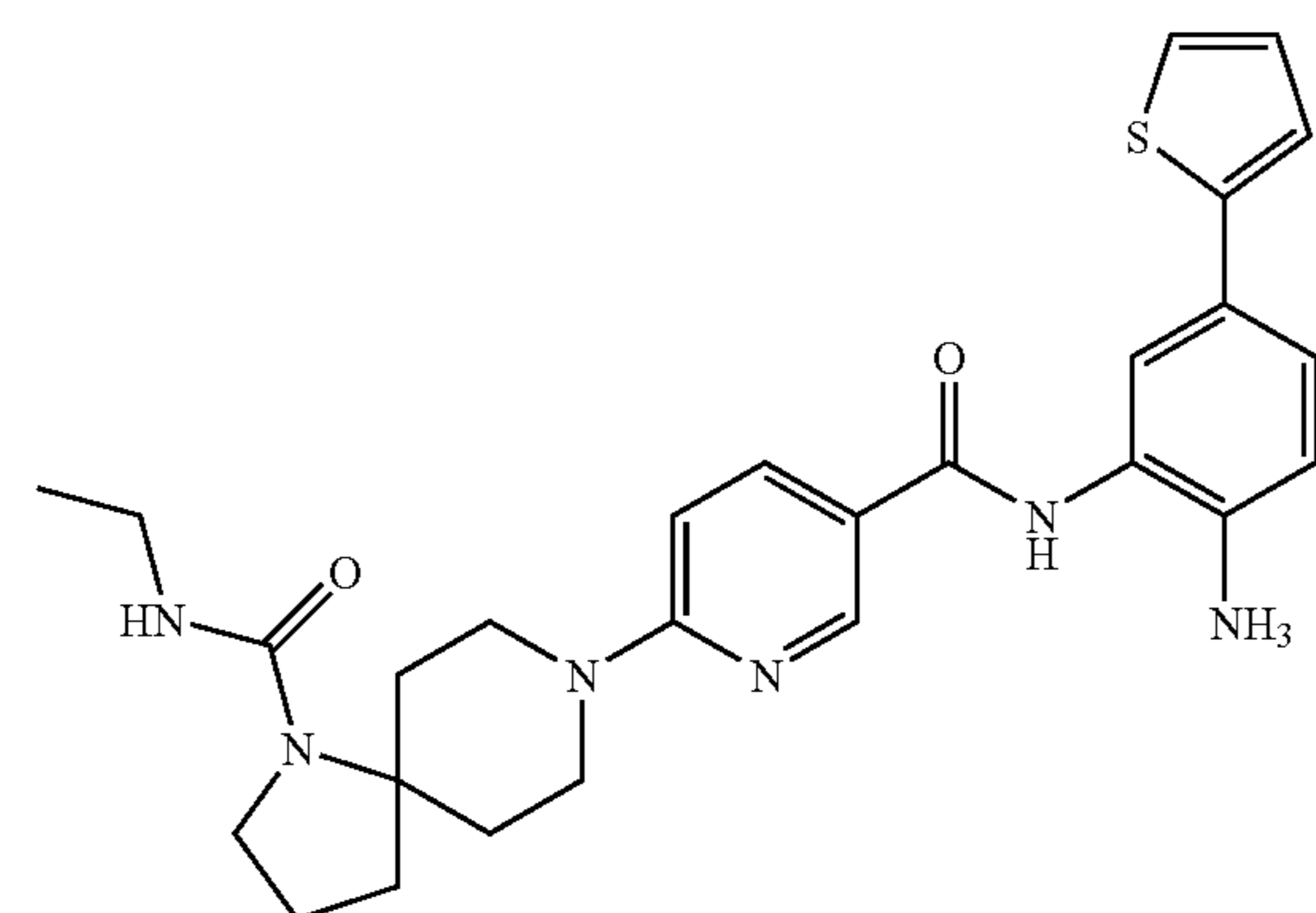
8-[5-({[2-Amino-5-(2-thienyl)phenyl]amino}carbonyl)pyridin-2-yl]-N-ethyl-1,8-diazaspiro[4.5]decane-1-carboxamide
