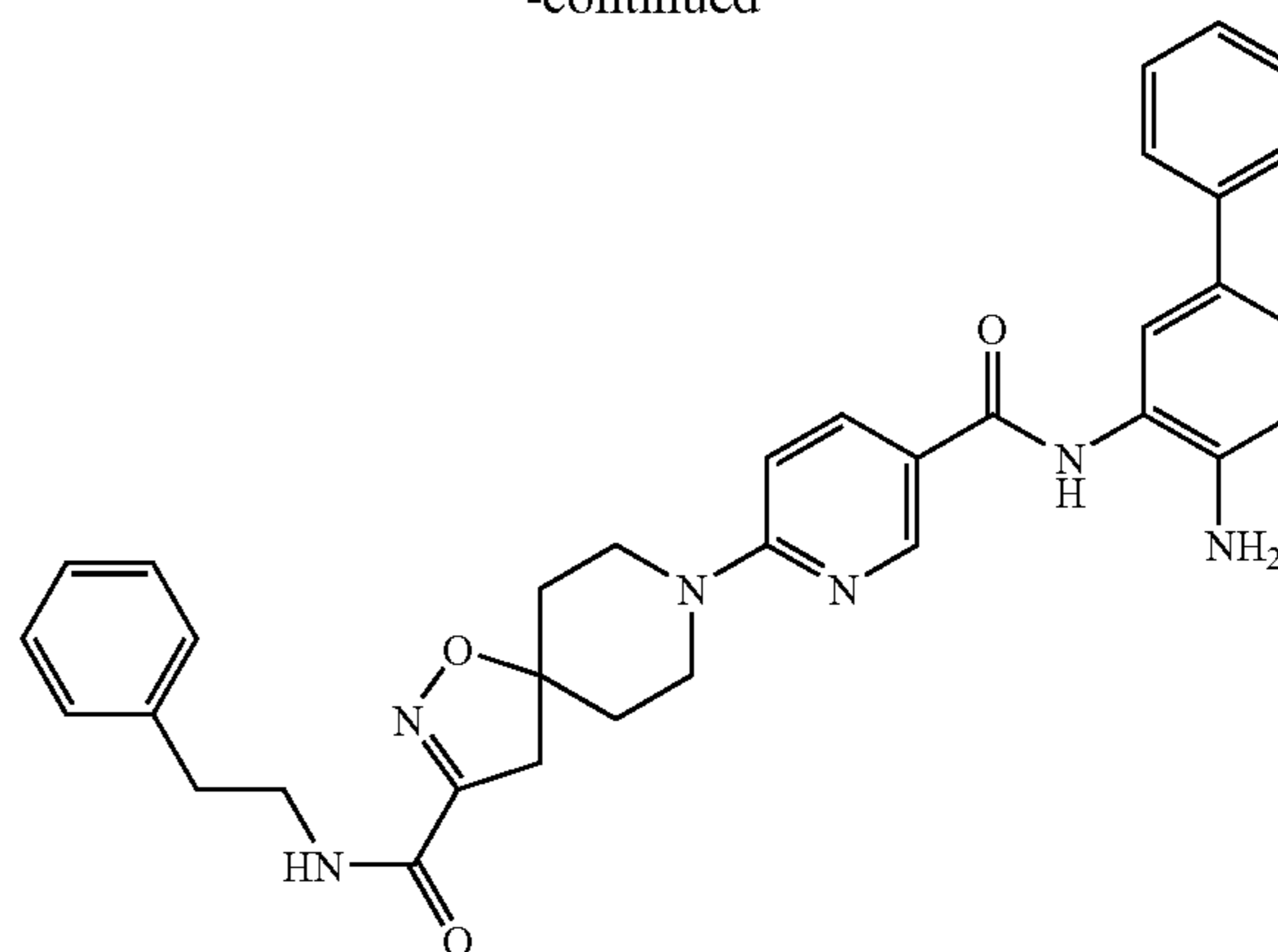
8-(5-[[[(4-Aminobiphenyl-3-yl)amino]carbonyl]pyridin-2-yl]-N-(2-phenylethyl)-1-oxa-2,8-diazaspiro[4.5]dec-2-ene-3-carboxamide
