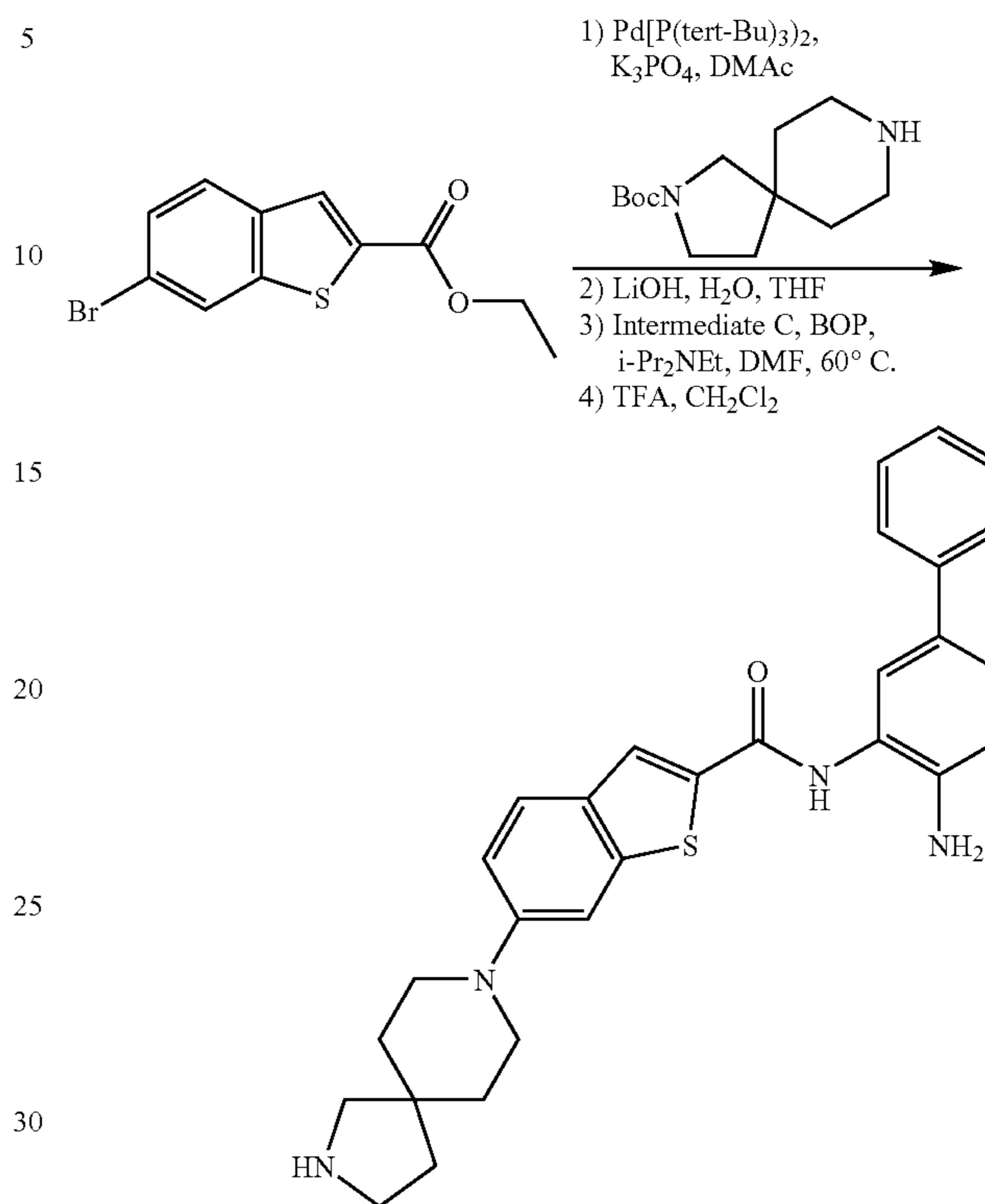
N-(4-Aminobiphenyl-3-yl)-6-(2,8-diazaspiro[4.5]dec-8-yl)-1-benzothiophene-2-carboxamide
