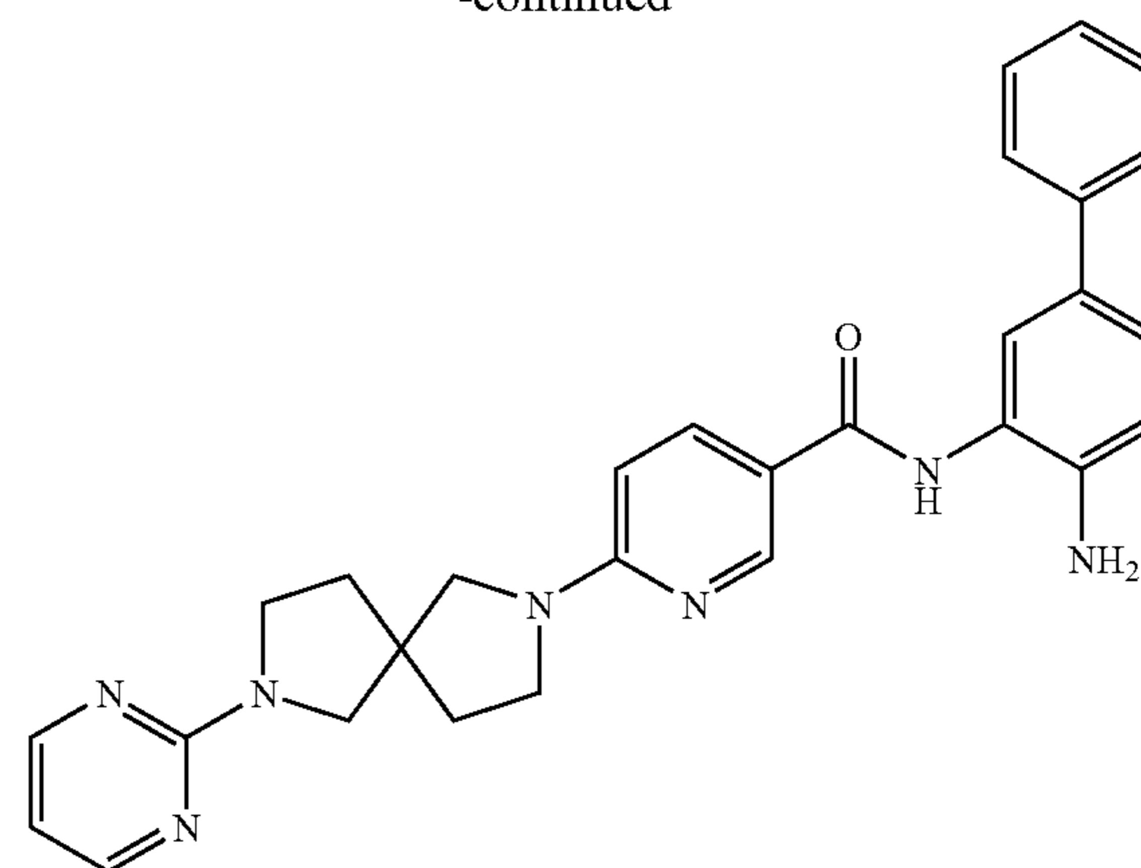
N-(4-Aminobiphenyl-3-yl)-6-(7-pyrimidin-2-yl-2,7-diazaspiro[4.4]non-2-yl)nicotinamide
