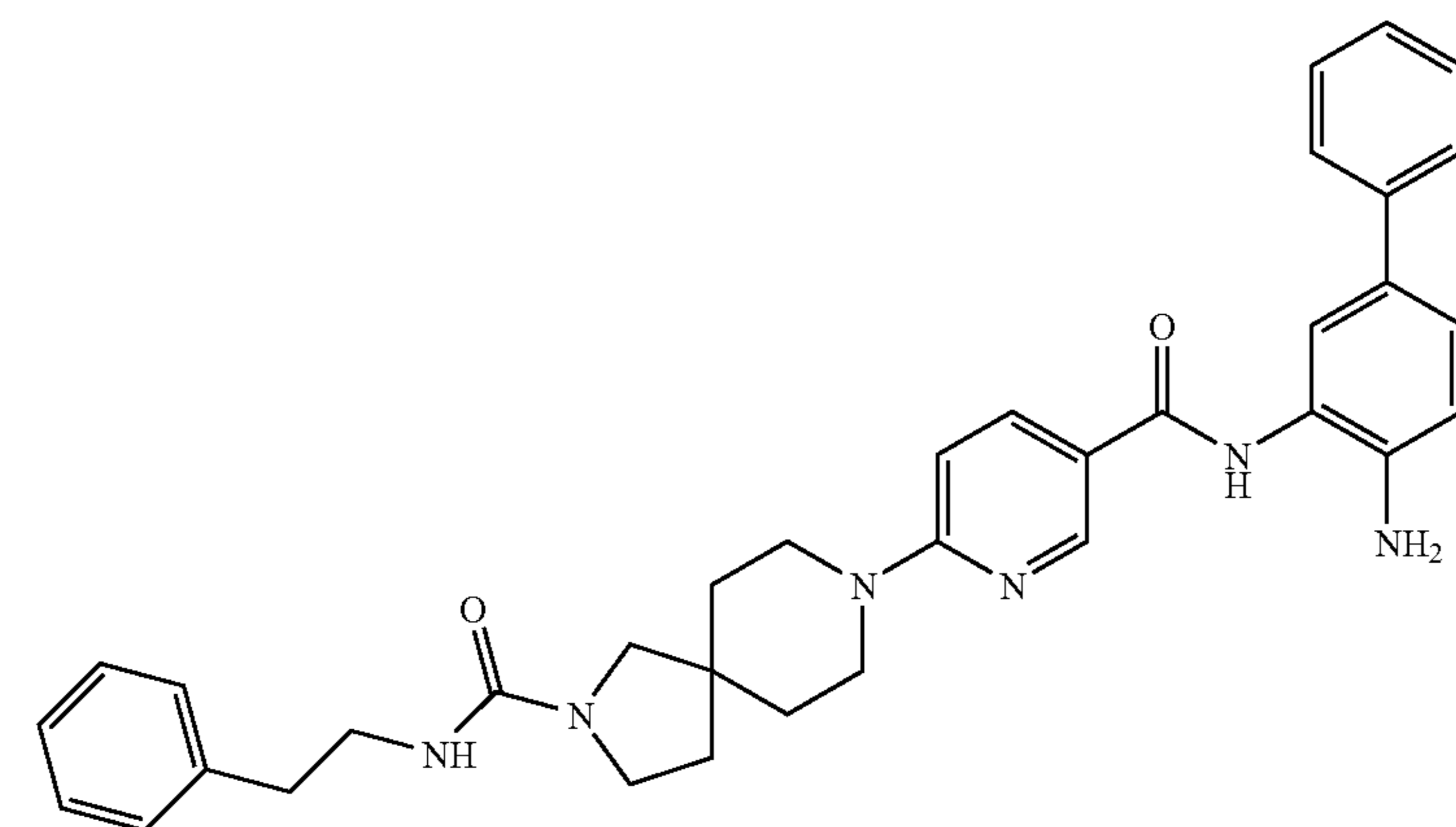
8-(5-[[[4-Aminobiphenyl-3-yl]amino]carbonyl]pyridin-2-yl)-N-(2-phenylethyl)-2,8-diazaspiro[4.5]decane-2-carboxamide
