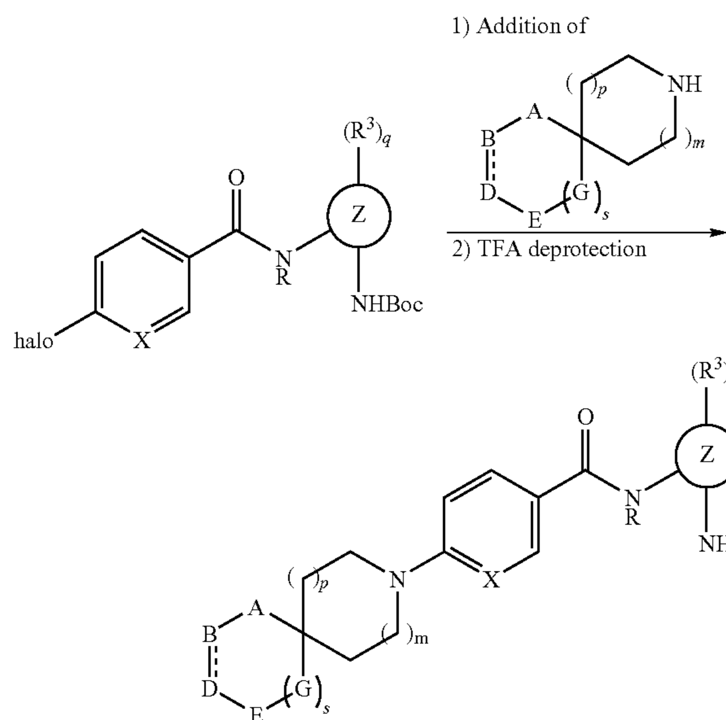
SCHEME 1
