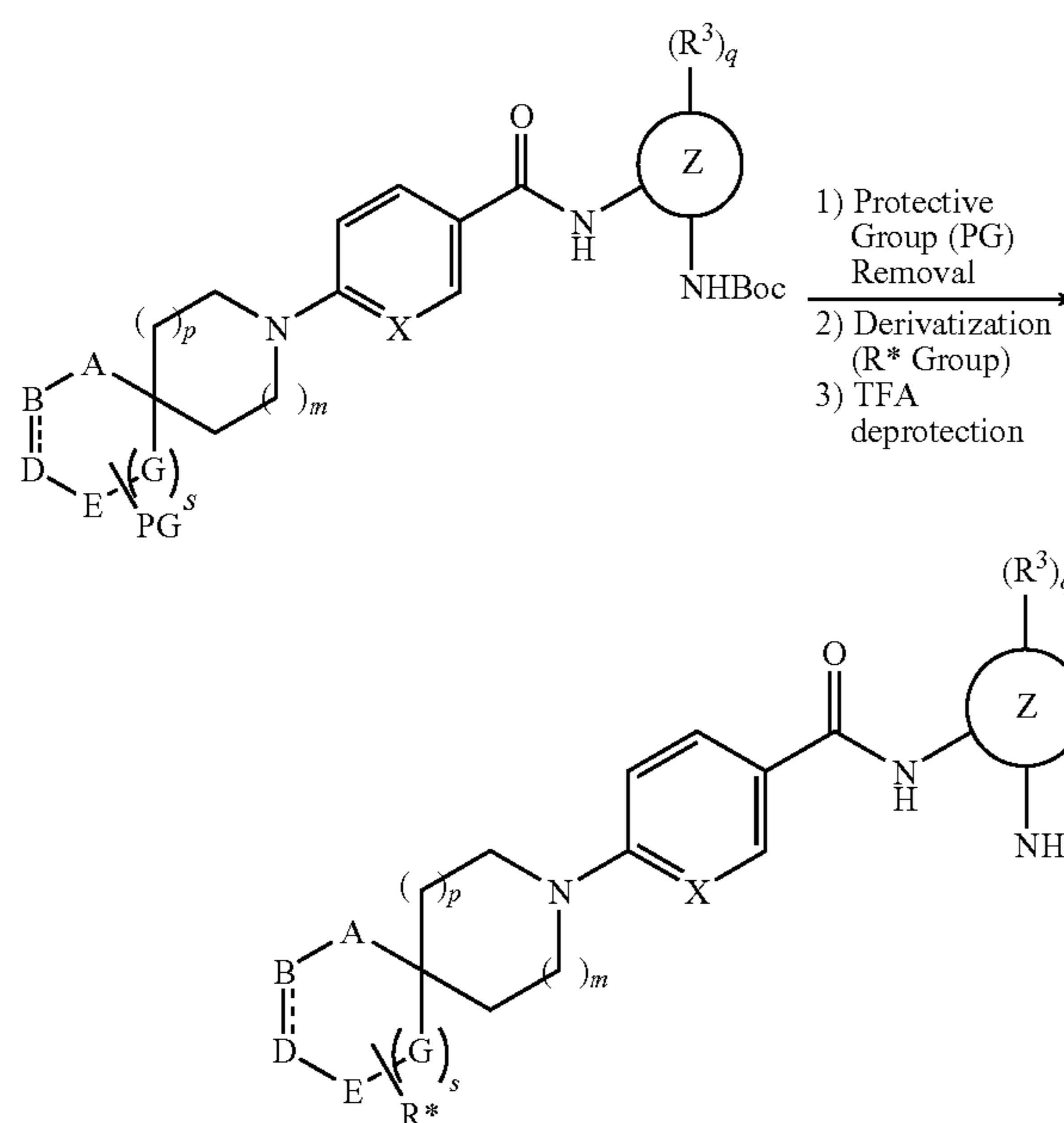
SCHEME 2
