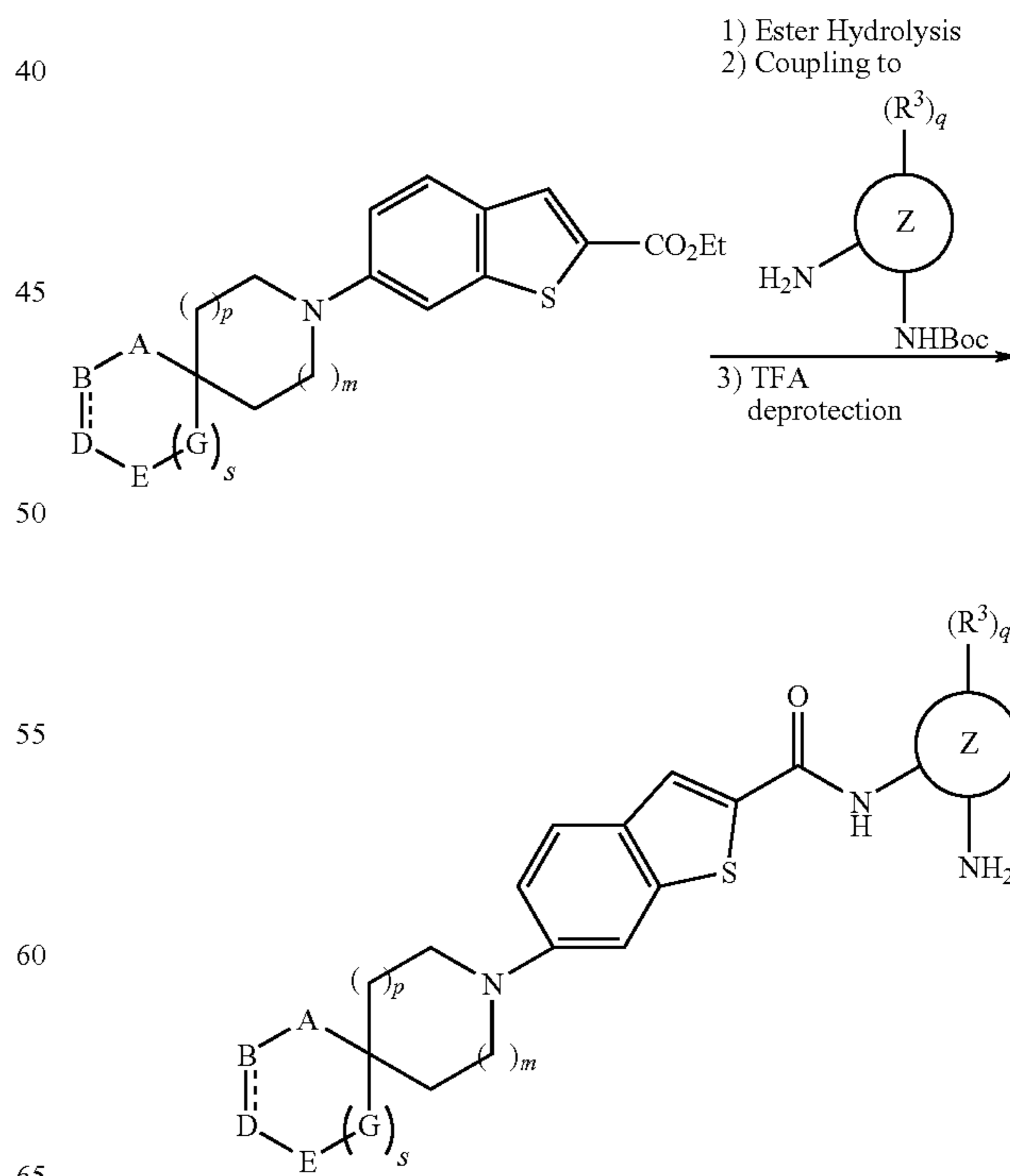
SCHEME 4
