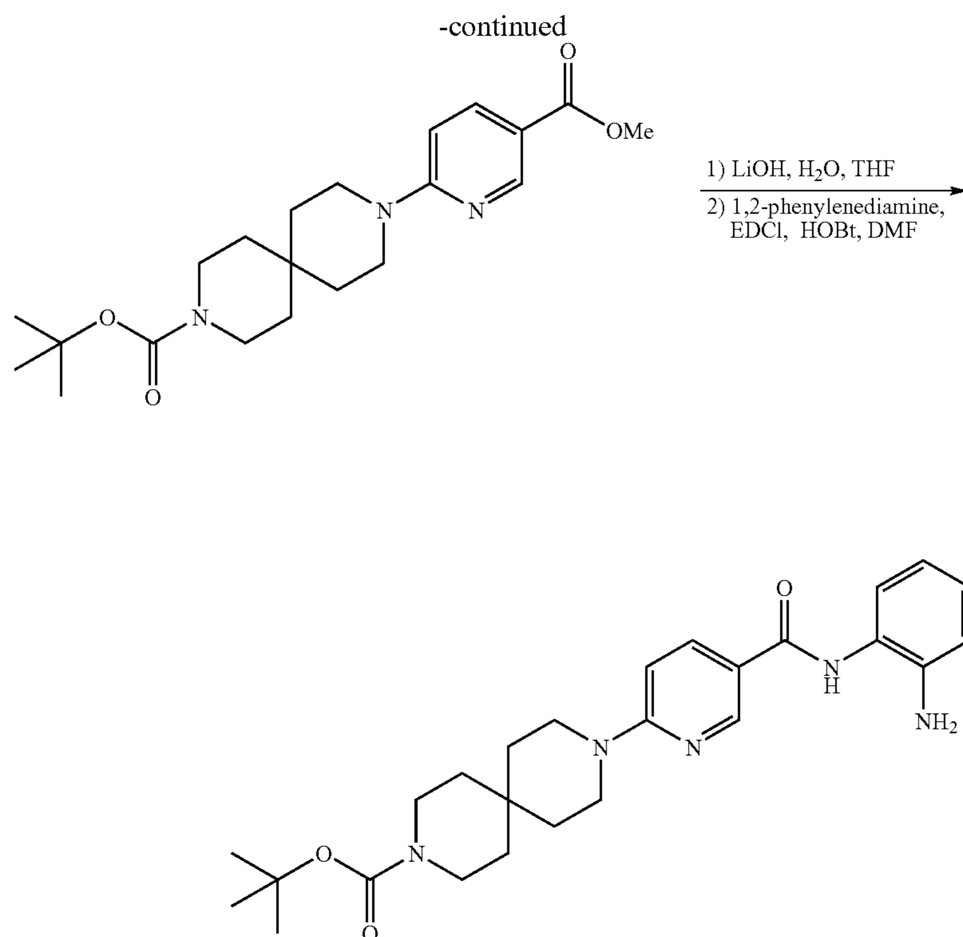
tert-butyl 9-(5-[[2-(aminophenyl)amino] carbonyl]pyridin-2-yl)-3,9-diazaspiro[5.5]undecane-3-carboxylate
