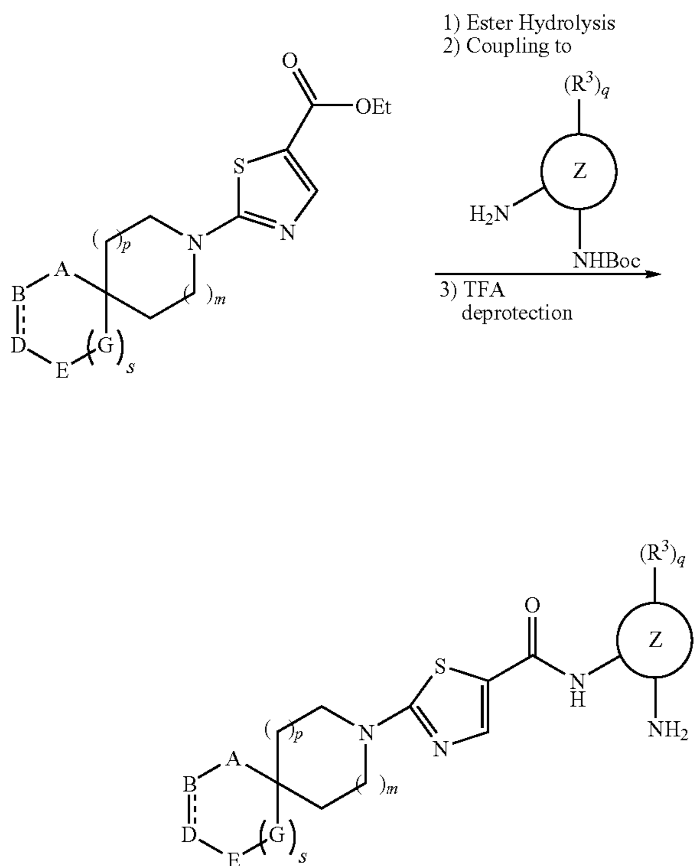
SCHEME 5
