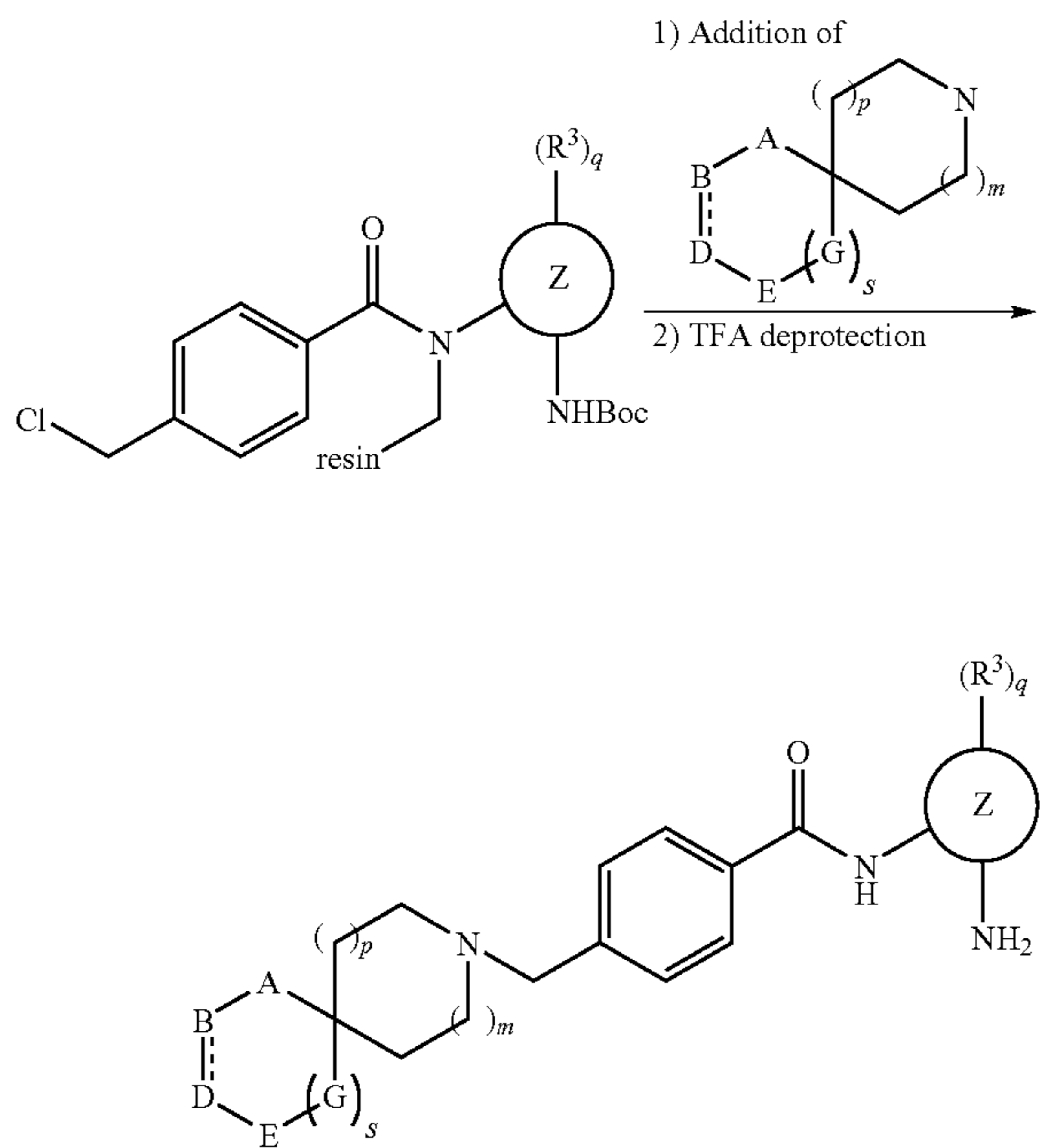
SCHEME 6
