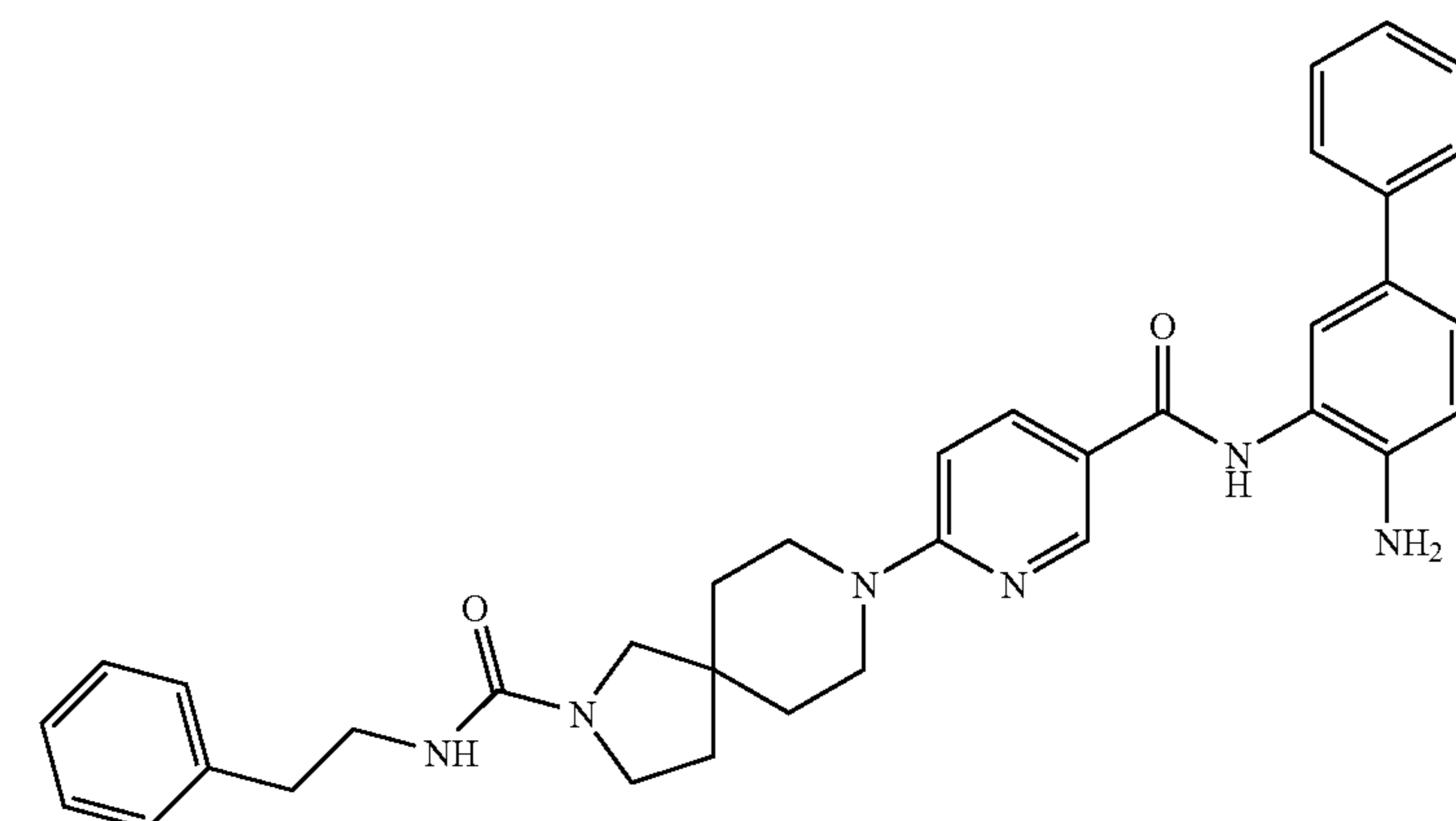
8-(5-[[[4-(2-phenylethylamino)phenyl]amino]carbonyl]pyridin-2-yl)-N-(2-phenylethyl)-2,8-diazaspiro[4.5]decane-2-carboxamide
