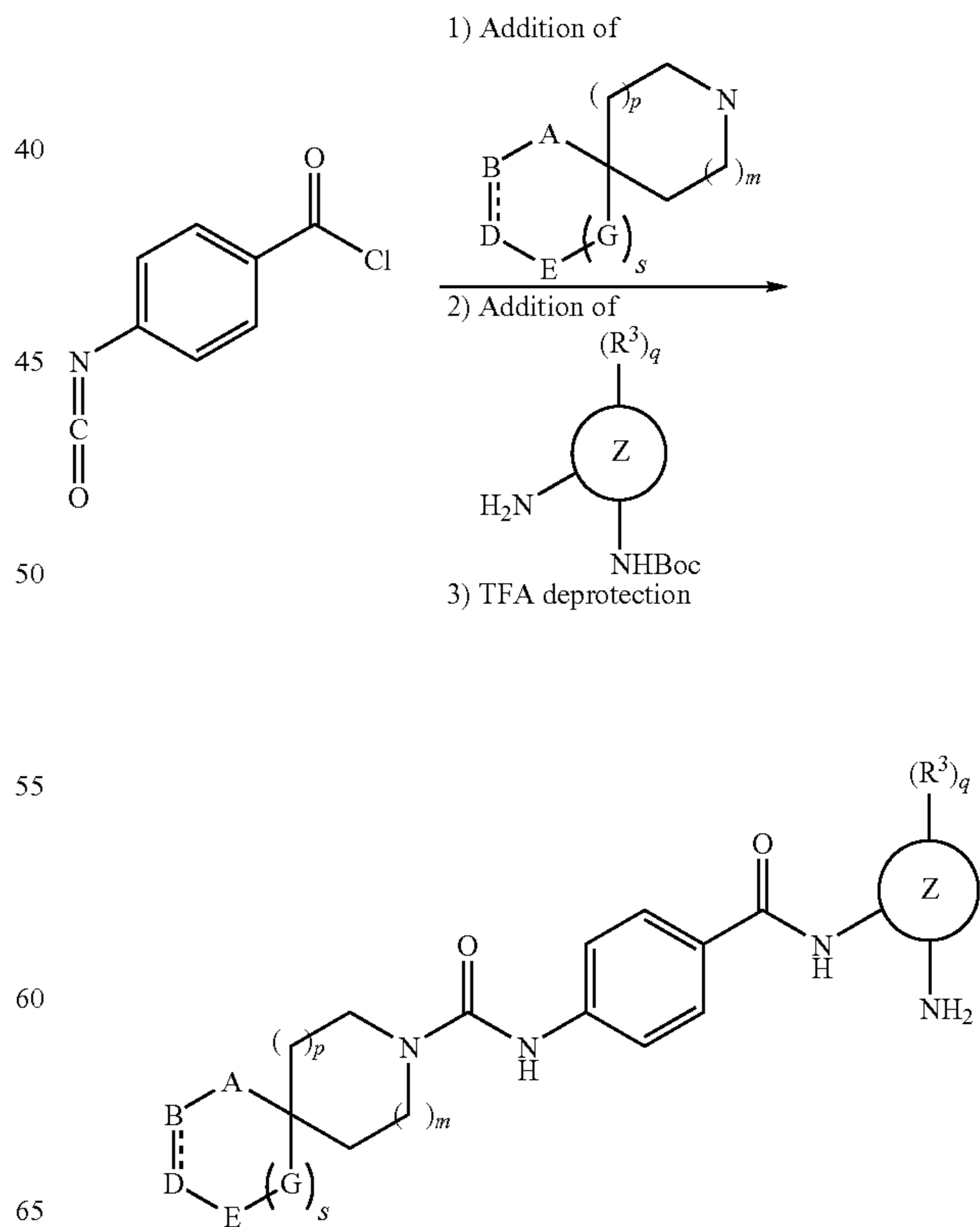
SCHEME 8
