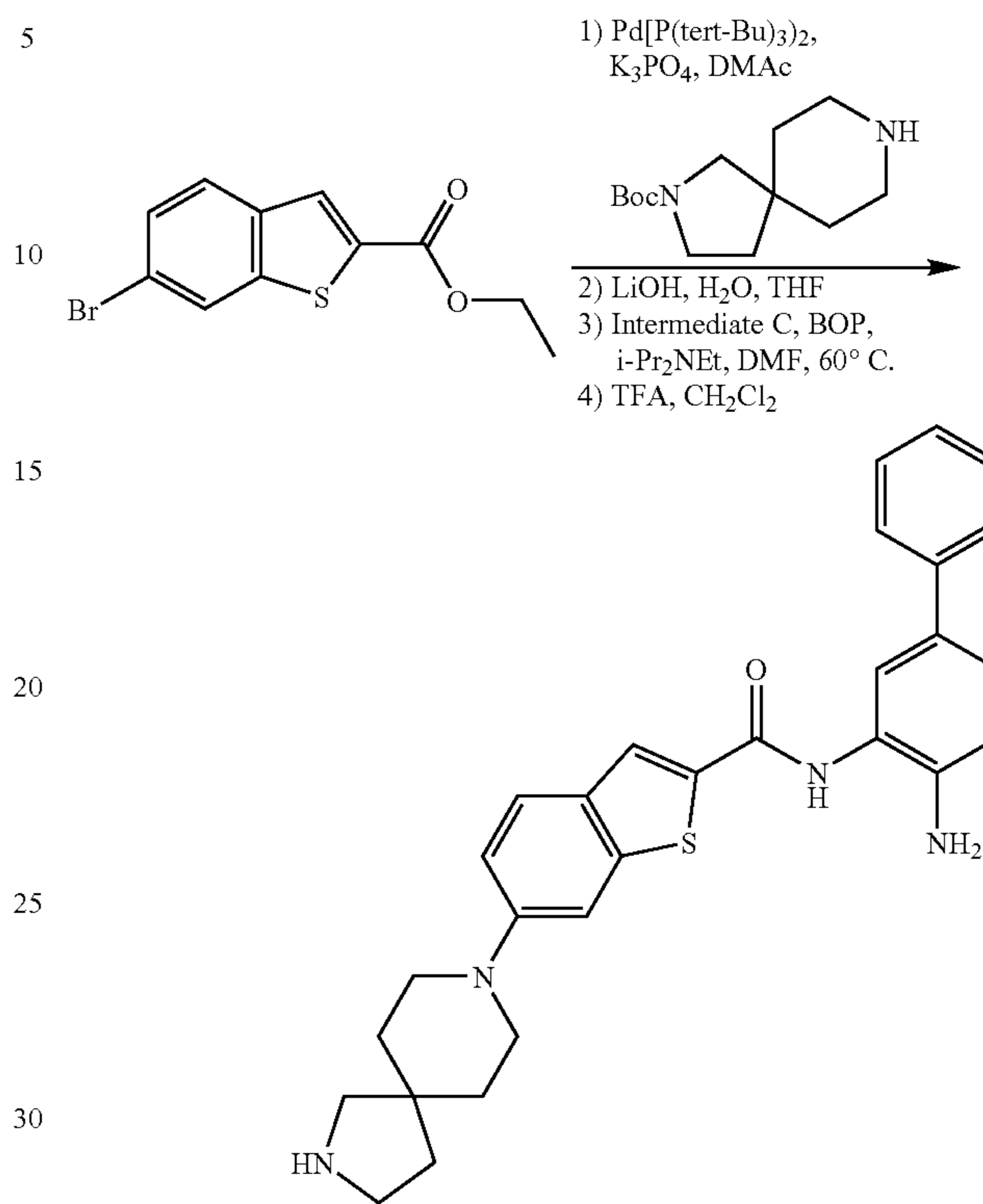
N-(4-Aminobiphenyl-3-yl)-6-(2,8-diazaspiro[4.5]dec-8-yl)-1-benzothiophene-2-carboxamide
