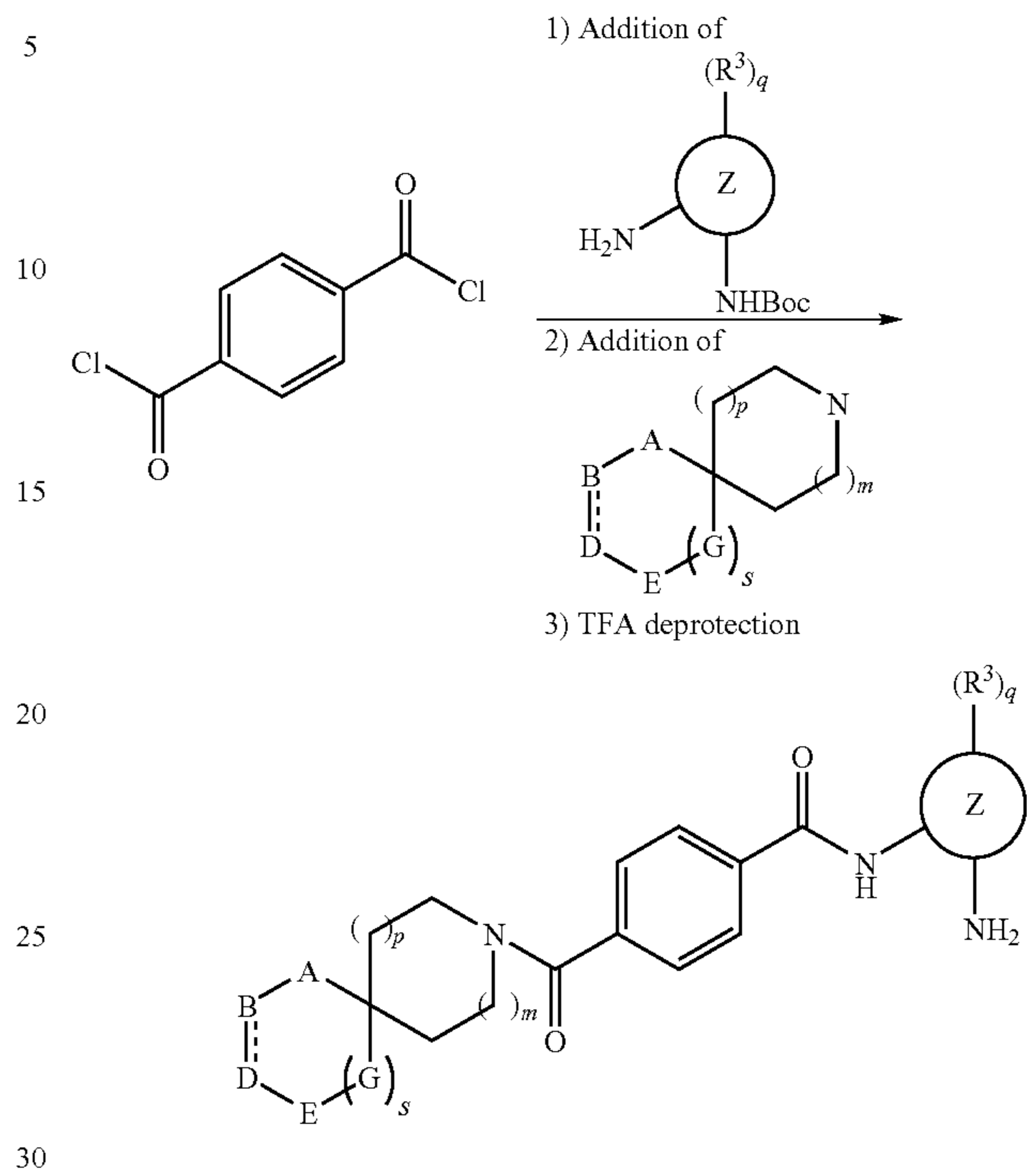
SCHEME 7
