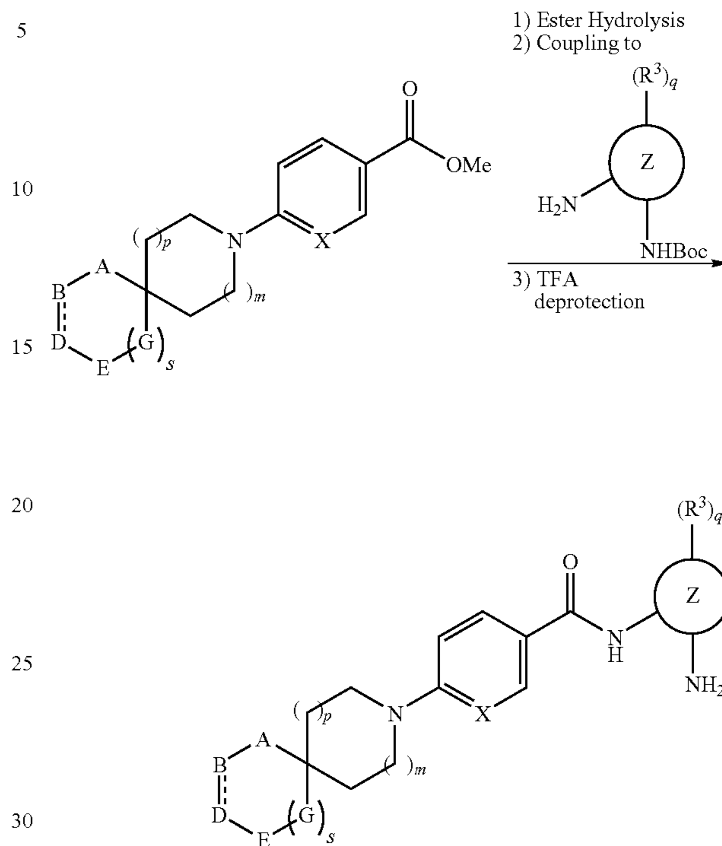
SCHEME 3
