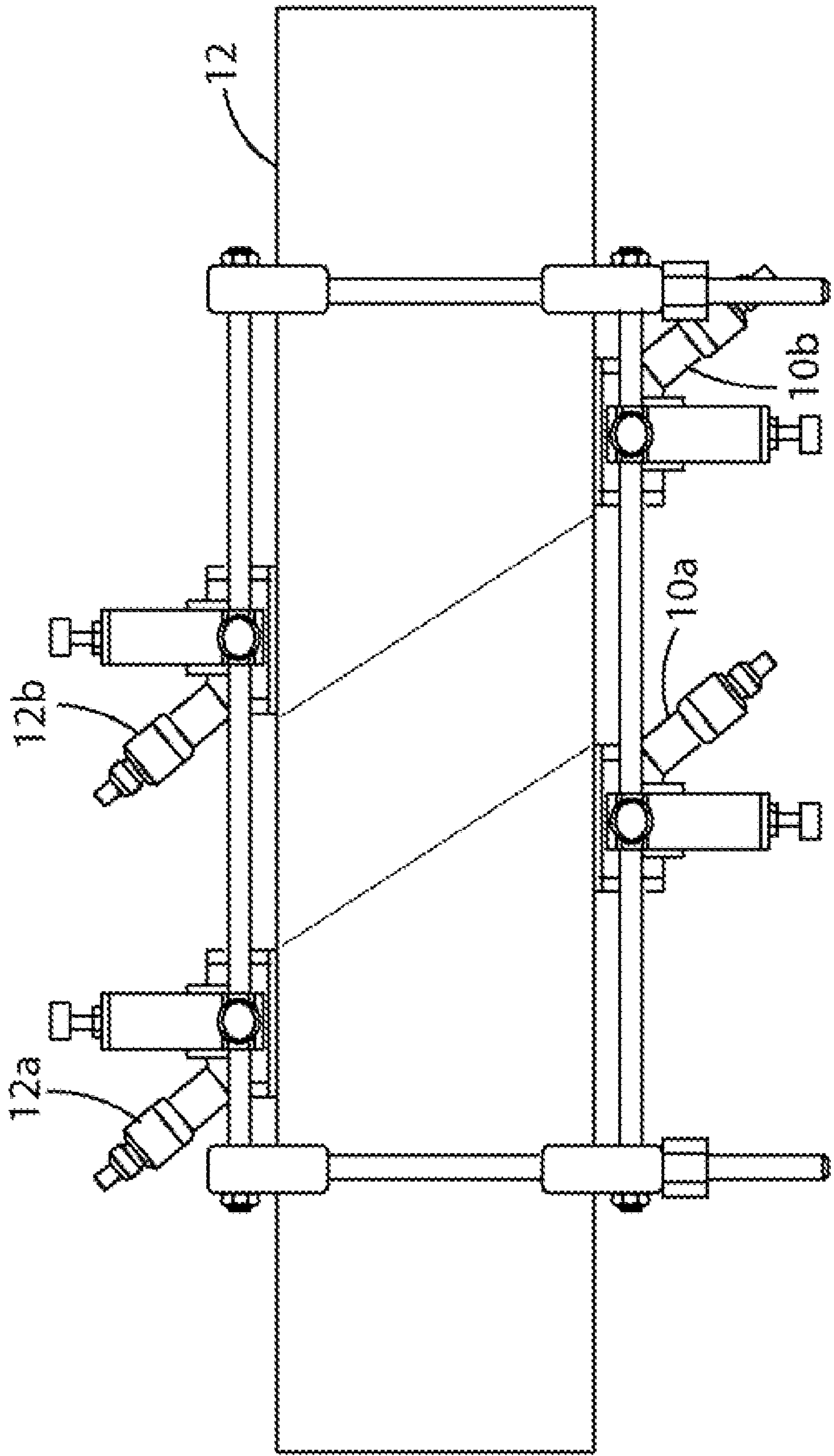
FIG. 1 (Prior Art)
