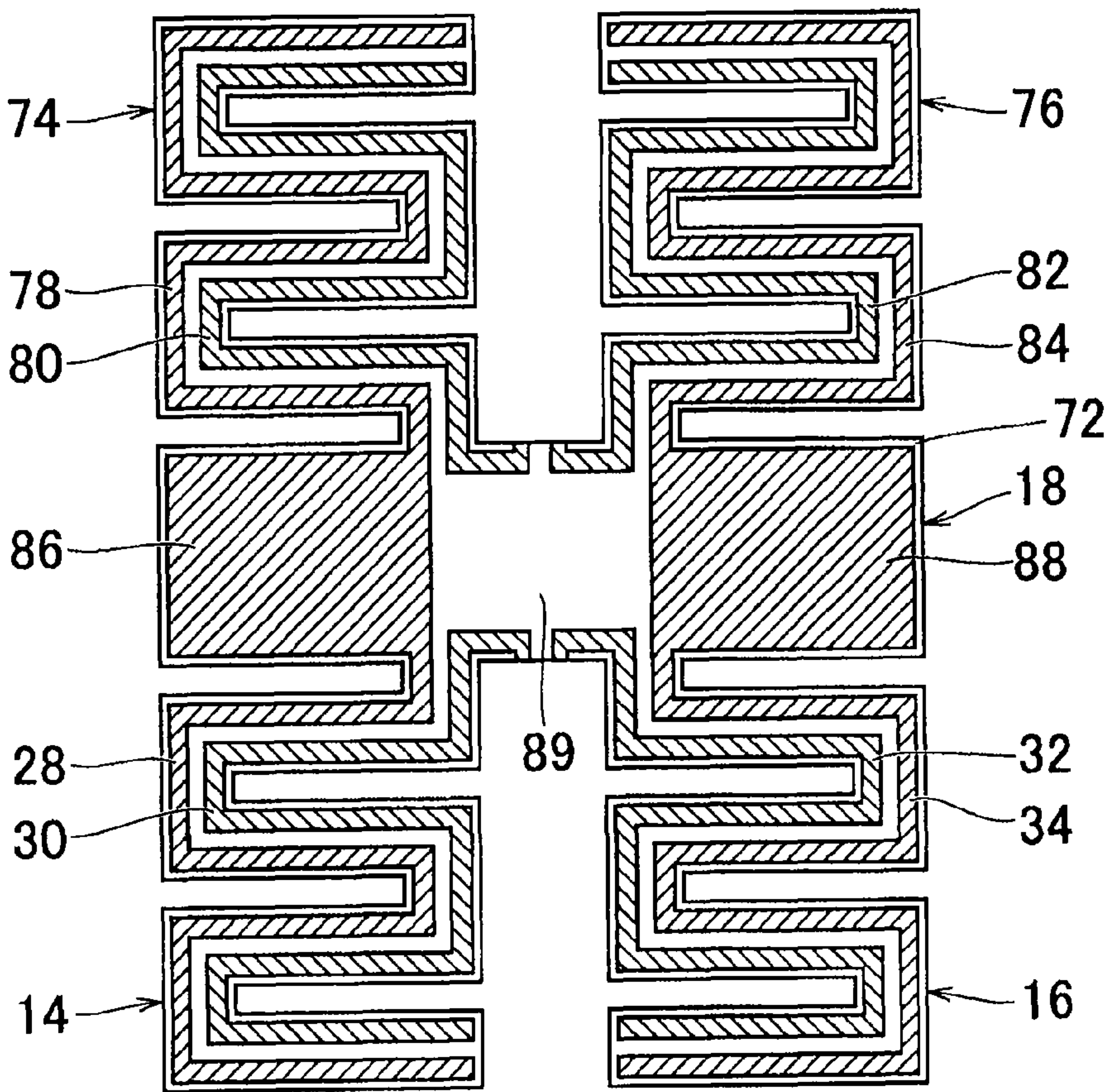
FIG. 8 PRIOR ART
