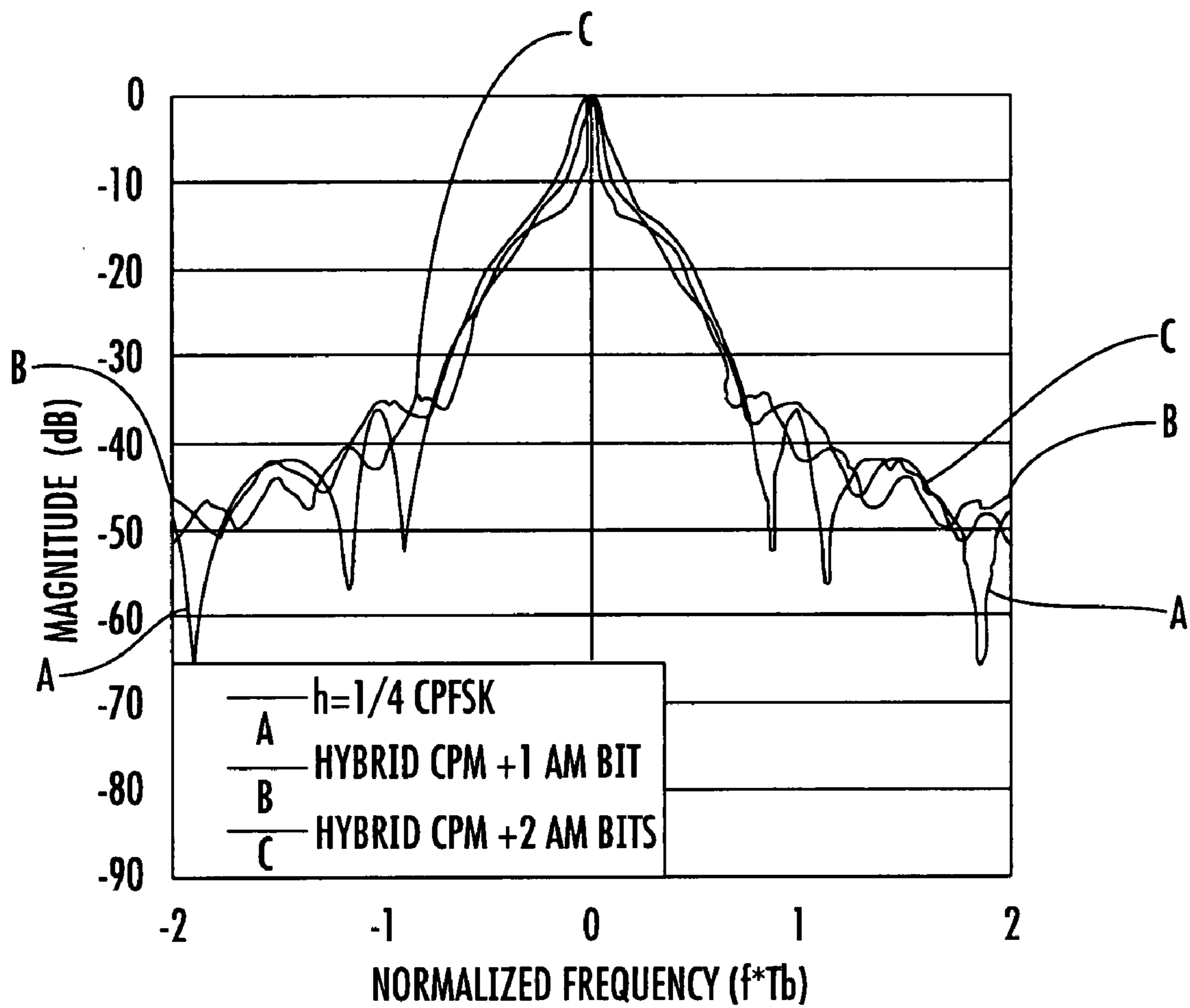
HYBRID AM PULSE SPECTRA
