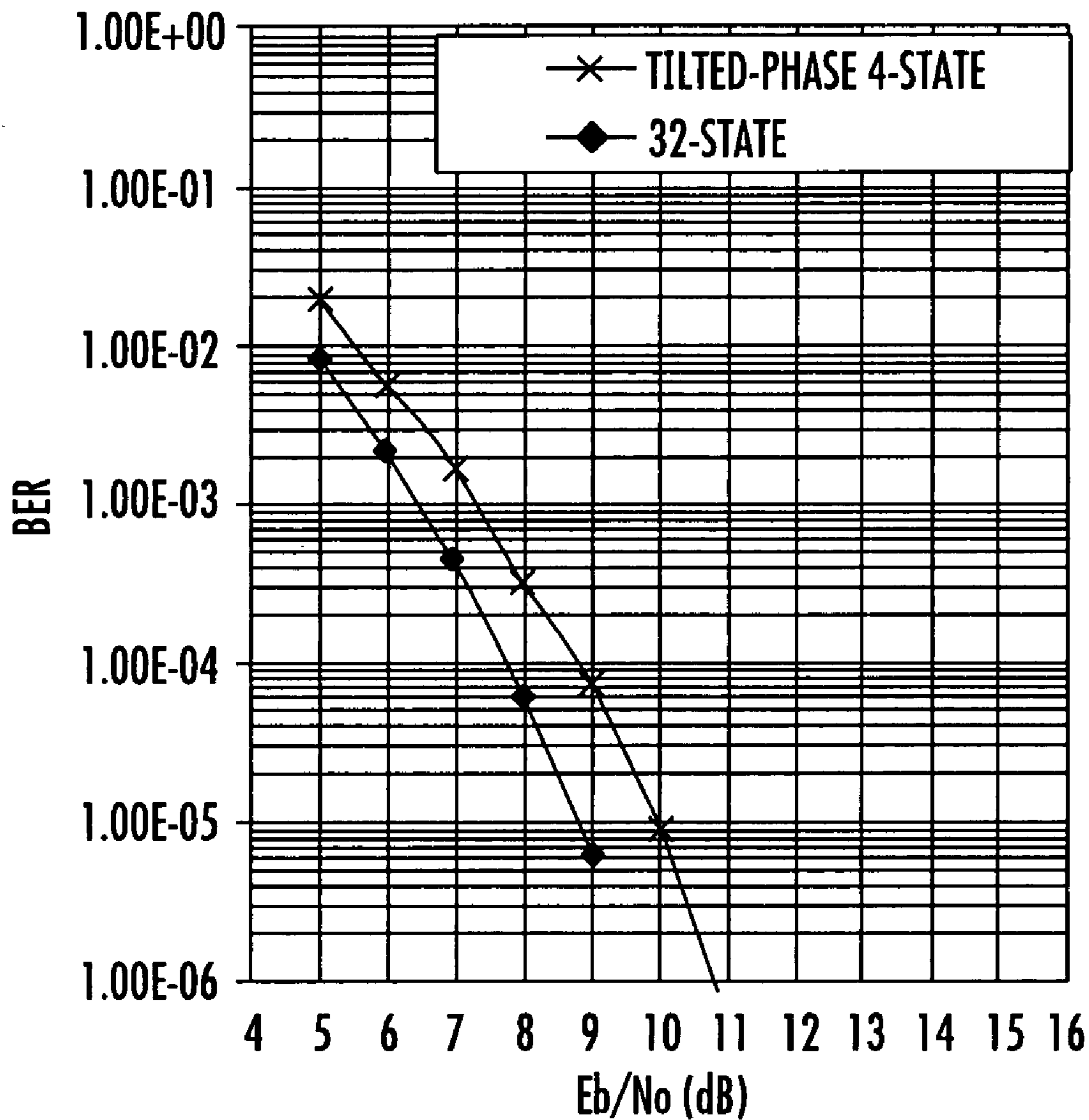
BER COMPARISON OF MIL-STD-188-181C h=\{ 4/16, 5/16 \} 4-ary CPFSK WITH TILTED-PHASE REDUCED-STATE MODEL
