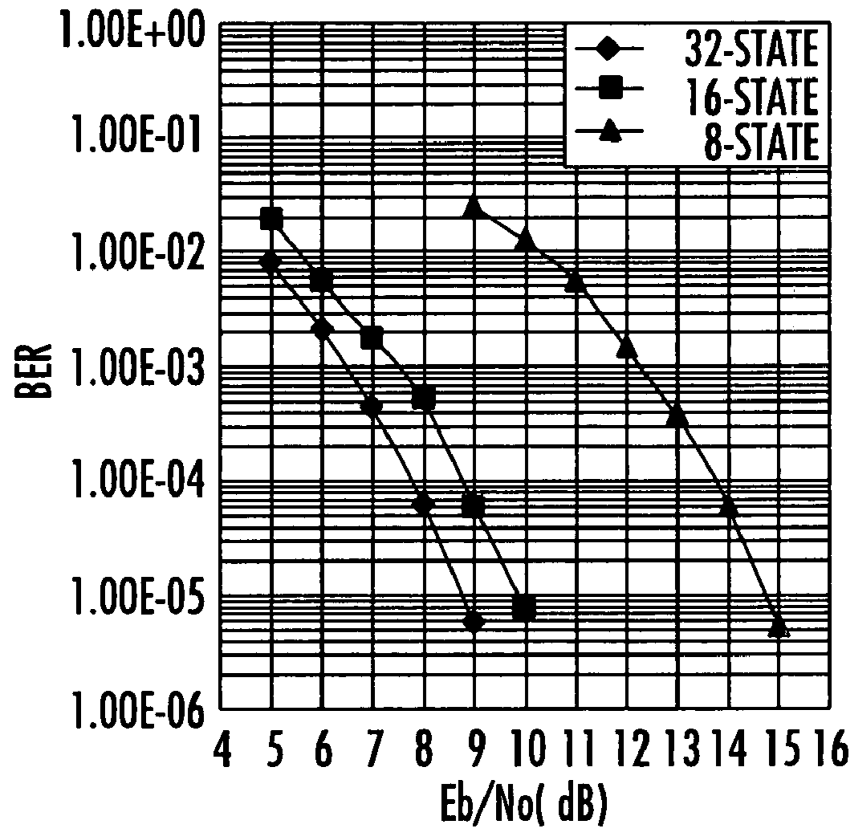
BER COMPARISON OF MIL-STD-188-181C h=\{4/16, 5/16\} 4-ARY CPFSK TO SET-PARTITIONING REDUCED-STATE MODEL.
