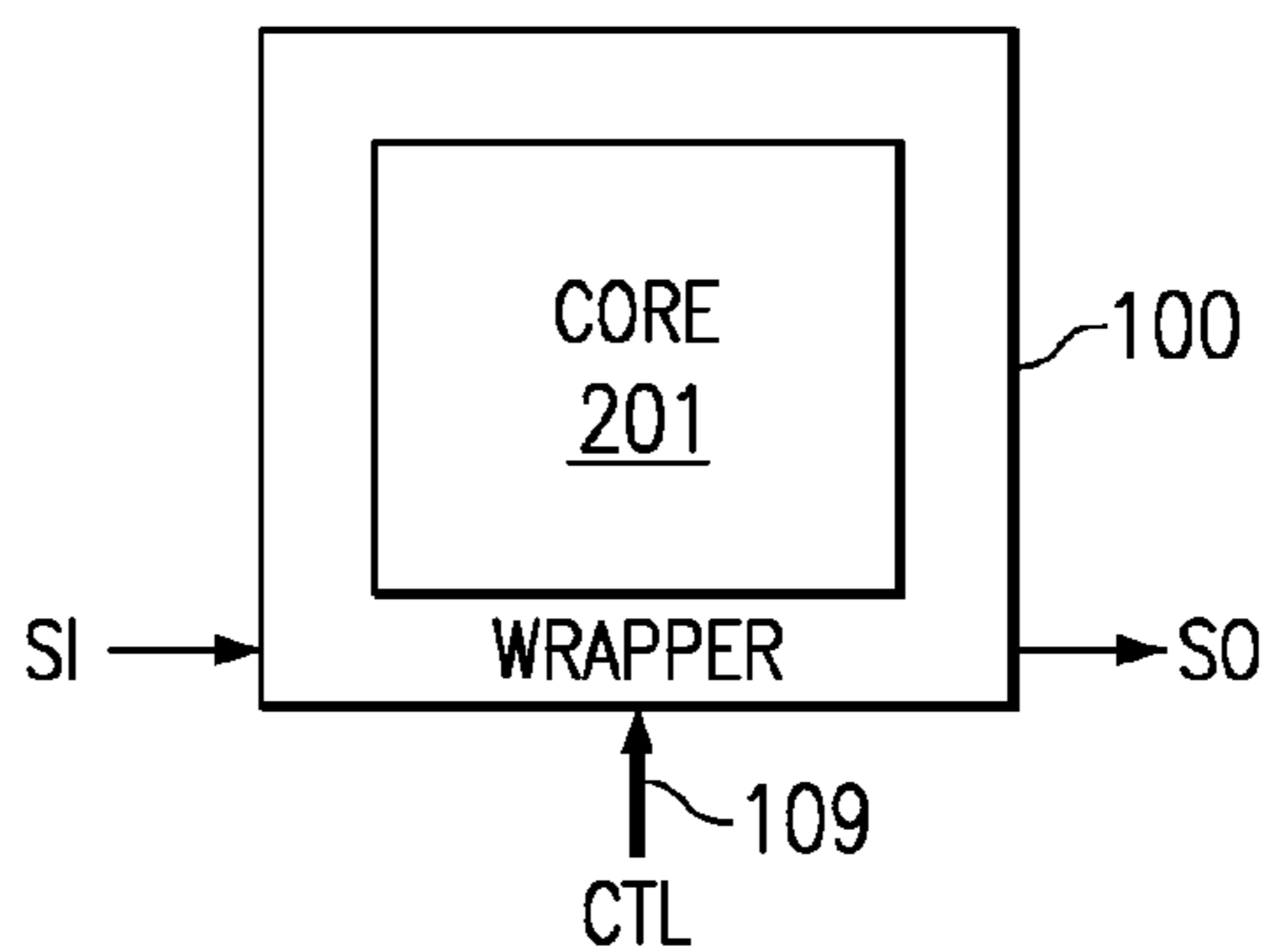
FIG. 2 (PRIOR ART)
