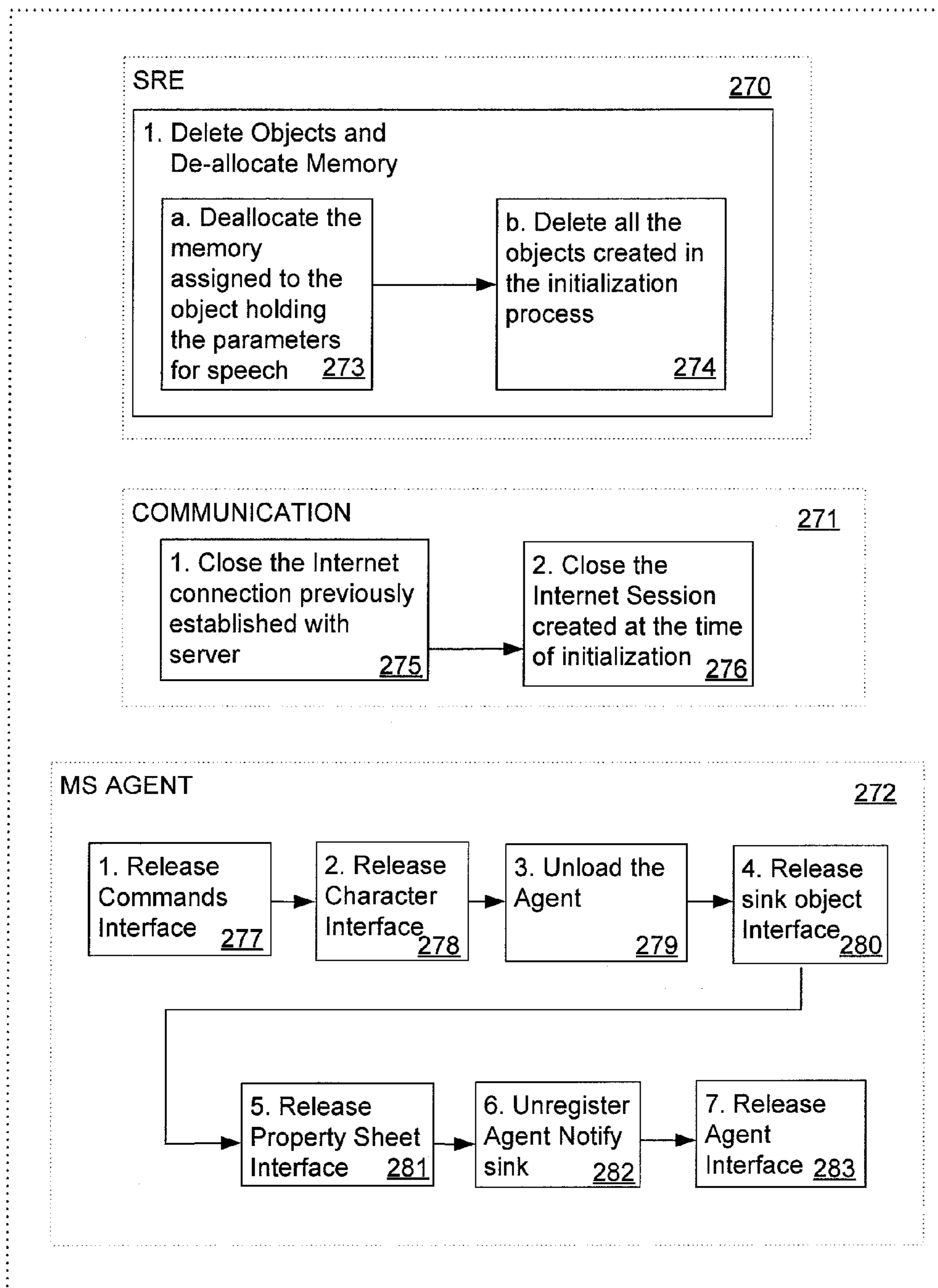
Fig. 4 Client-side Un-Initialization
