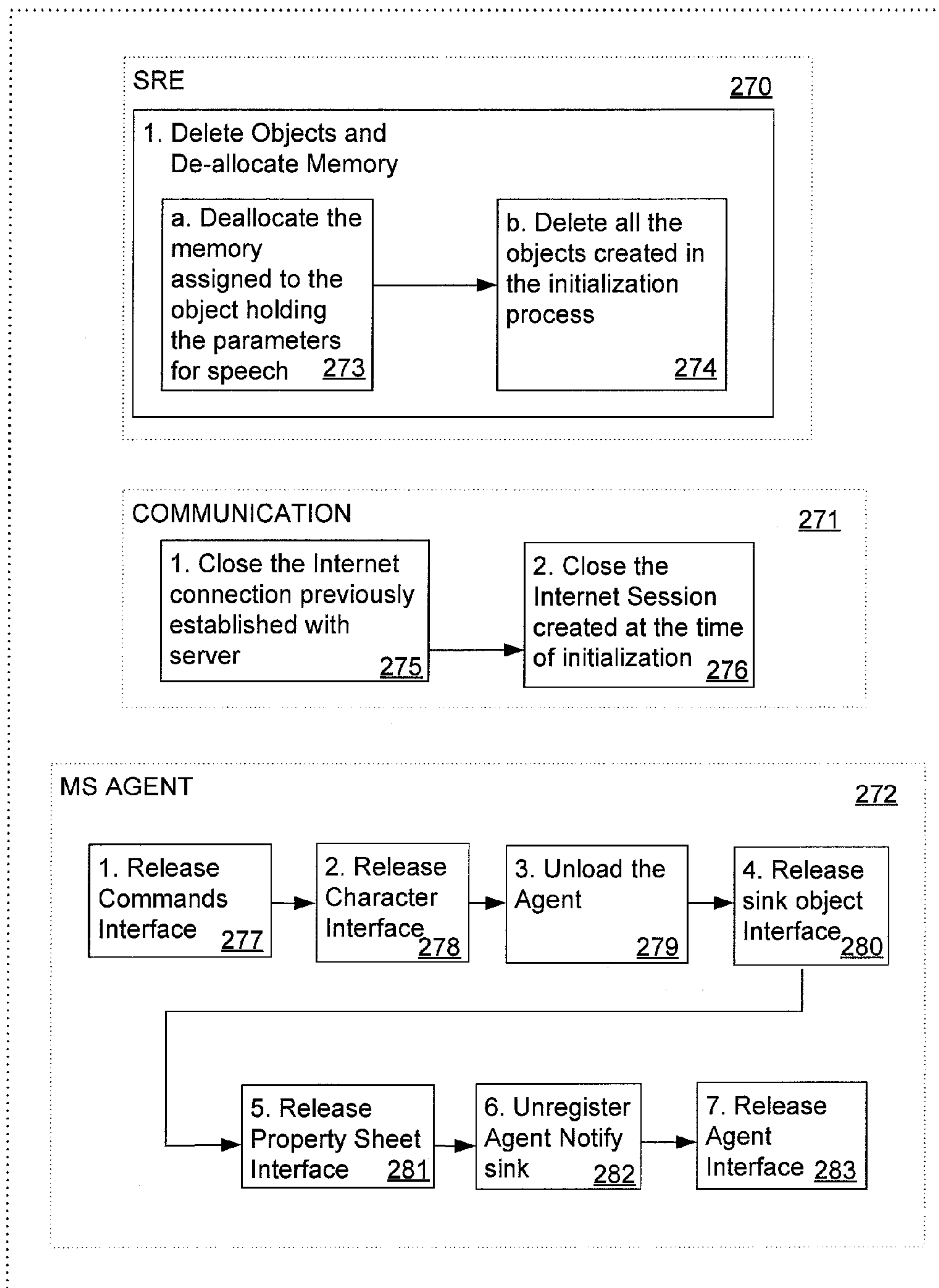
Fig. 4 Client-side Un-Initialization
