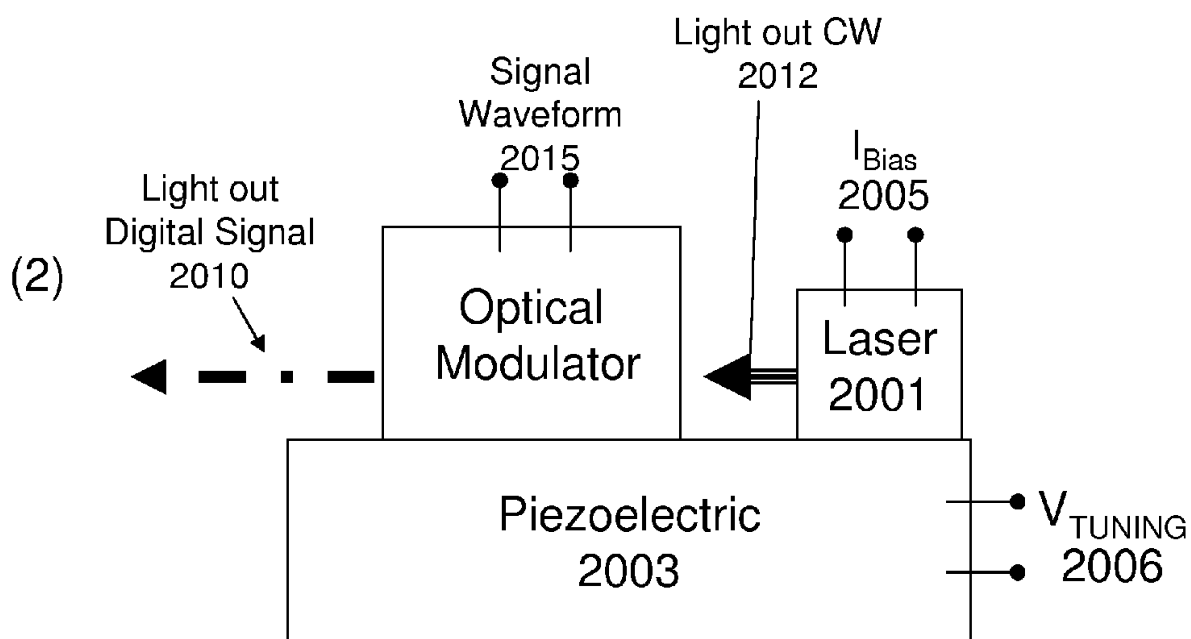
Optical modulator with tunable laser assembly 2030
