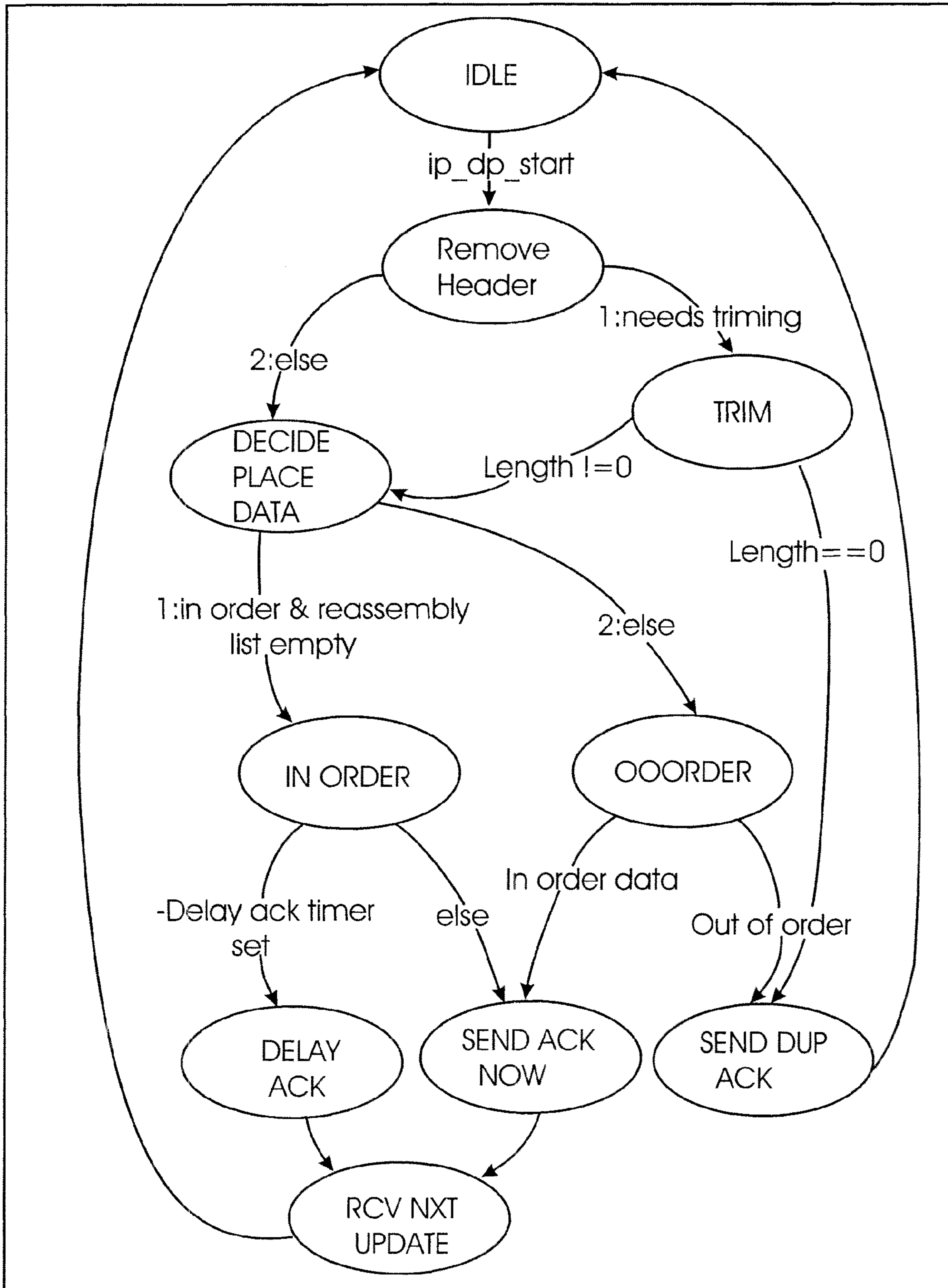
Data Processing State Machine
