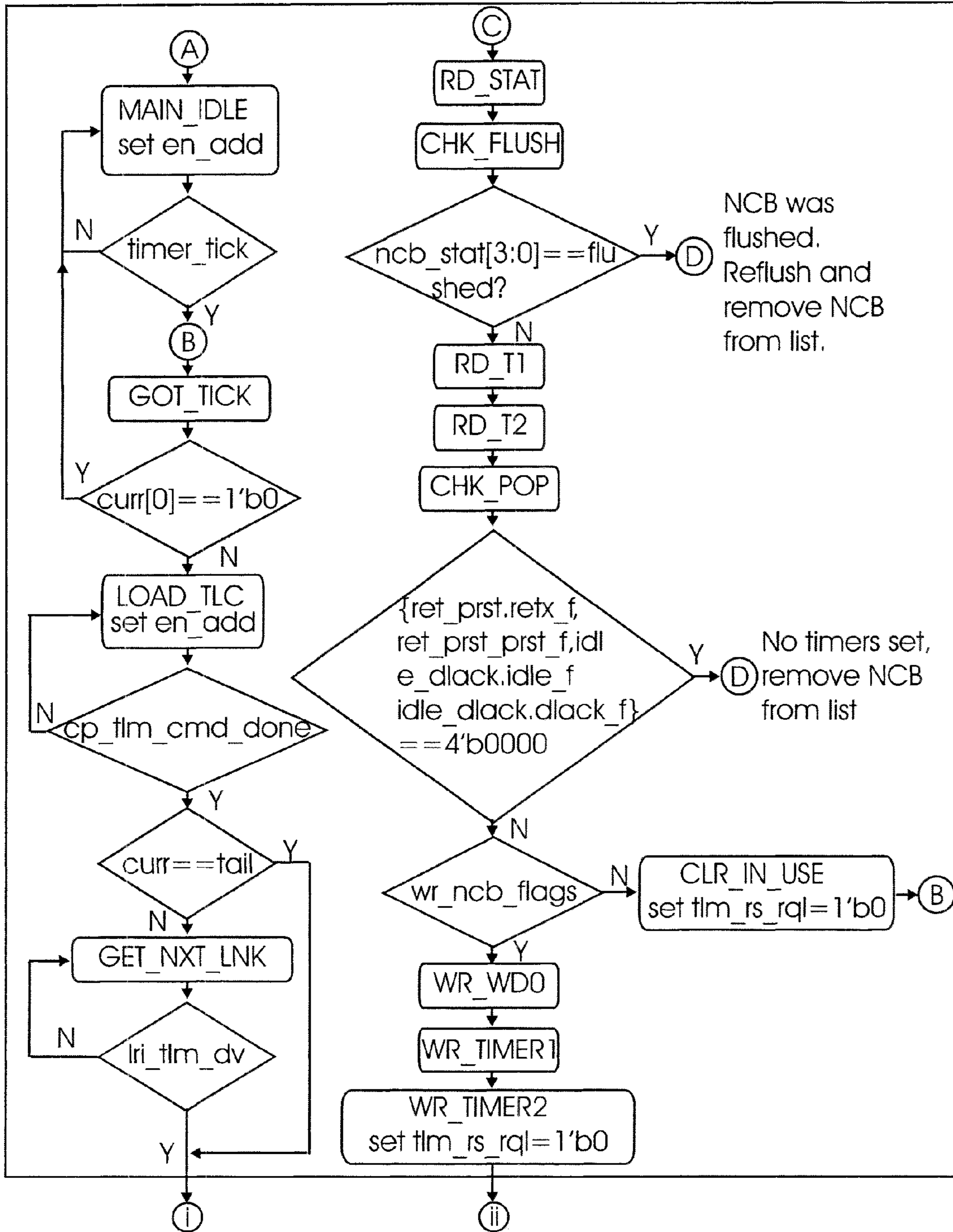
Figure 3D1-A Timer List Manager State Machine
