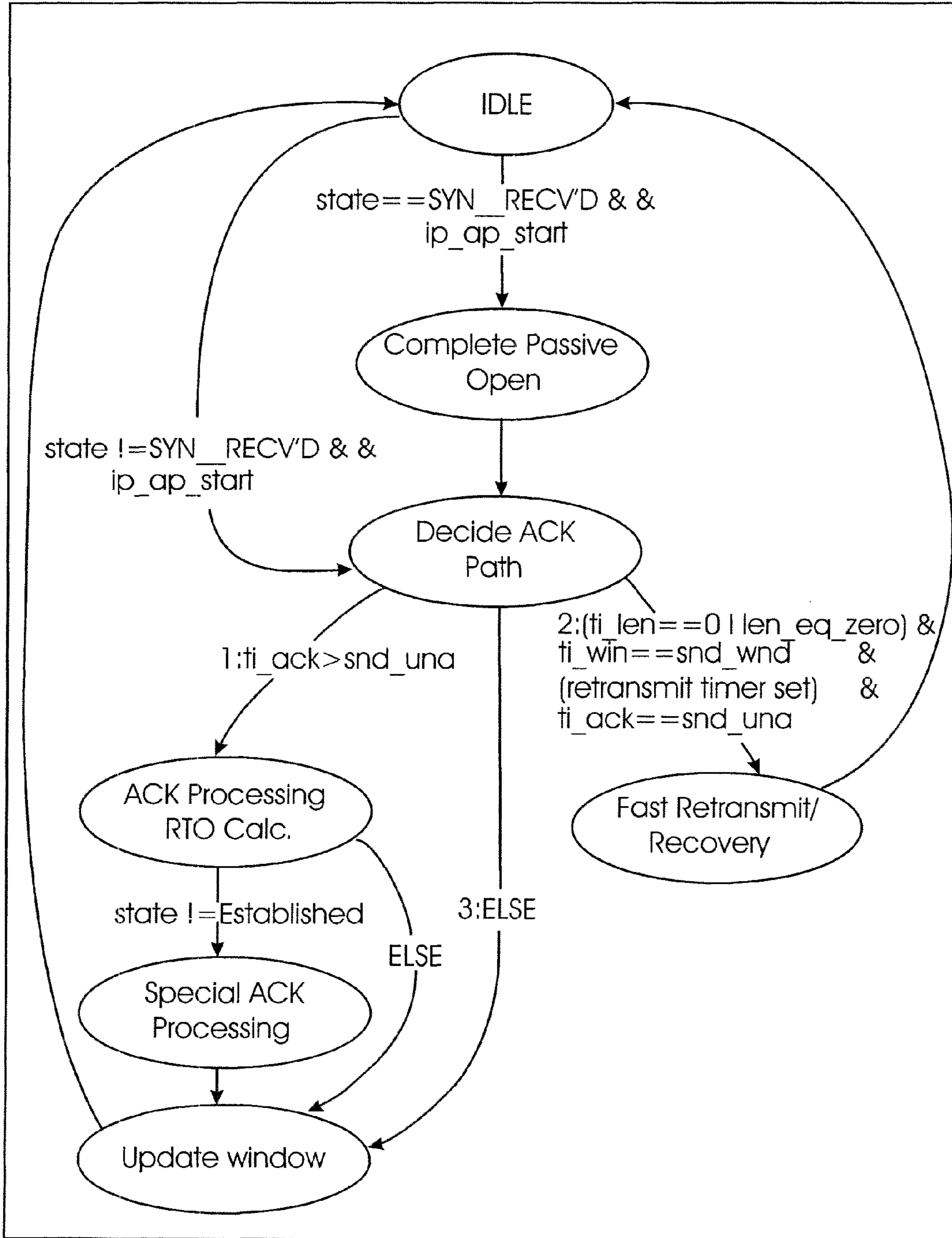
Figure3C6 - ACK Processor
