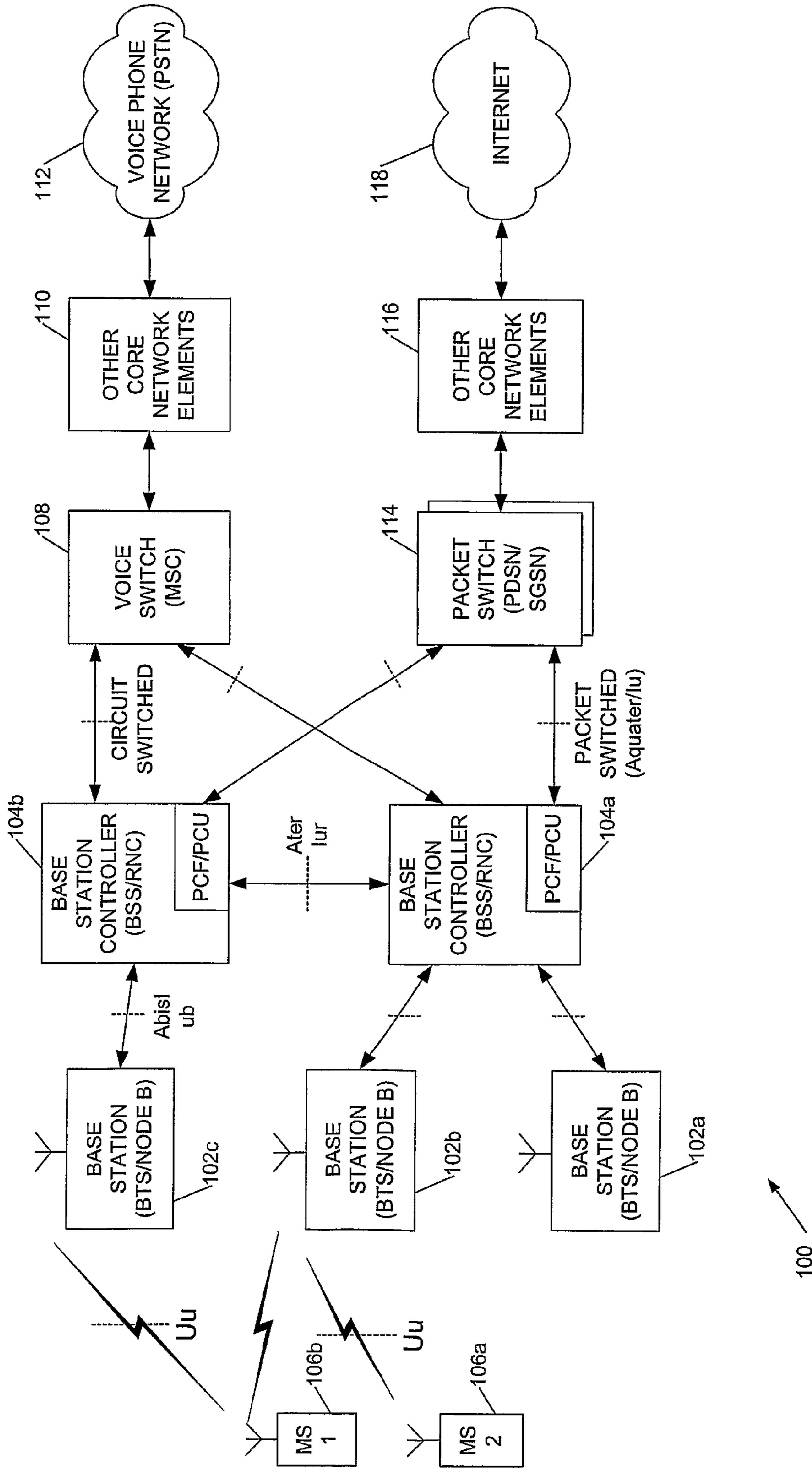
Figure 1 PRIOR ART
