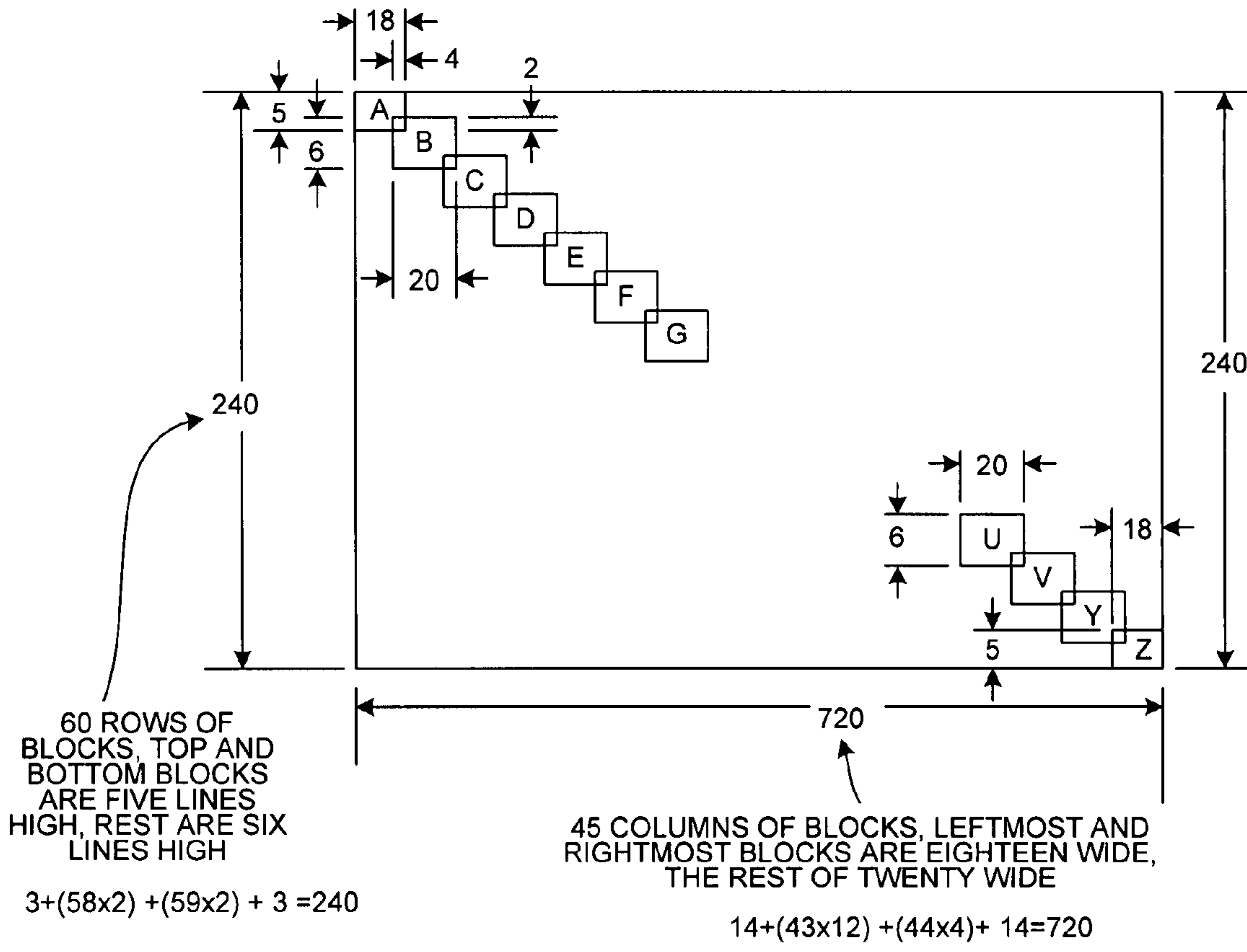
LAYOUT OF BLOCKS IN A FIELD FIG. 6
