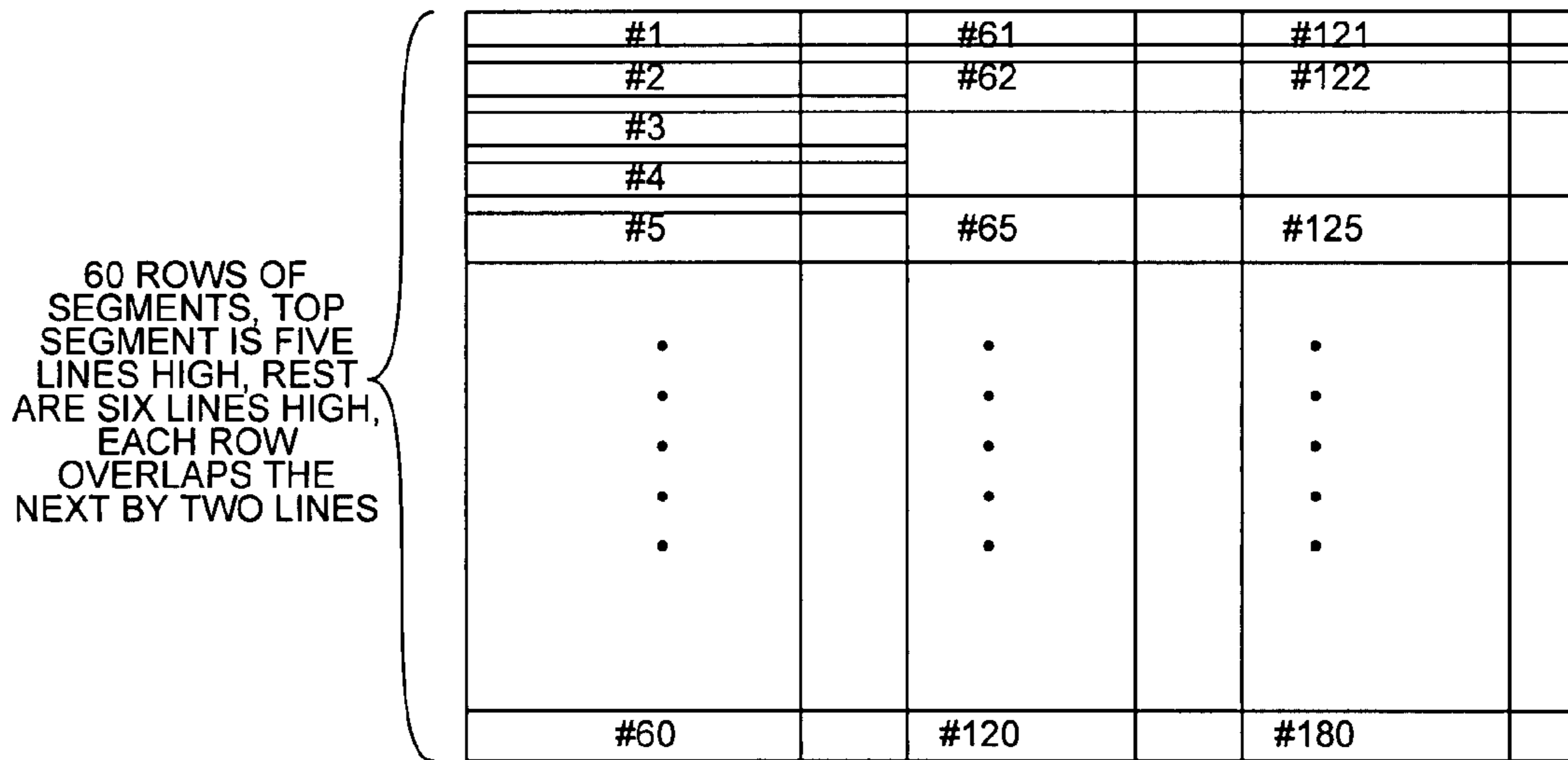
SEGMENT LOADING SEQUENCE FIG. 5
