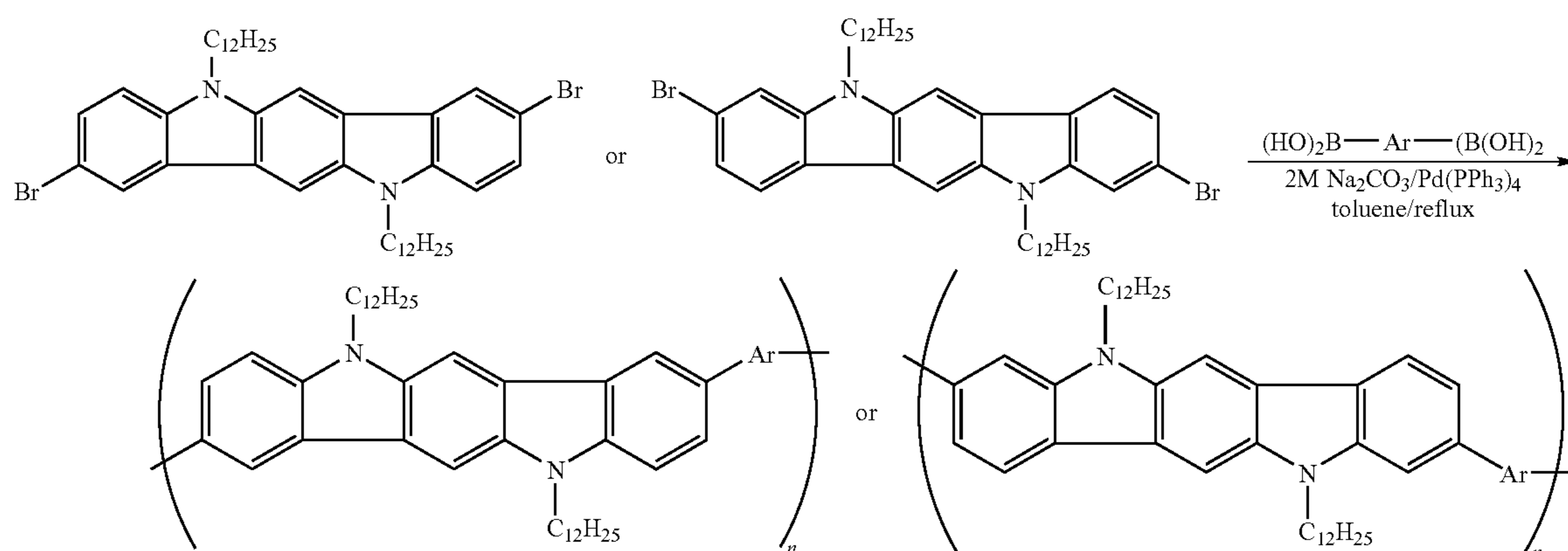
Scheme 2. Synthesis of polymer (13) through (18).
