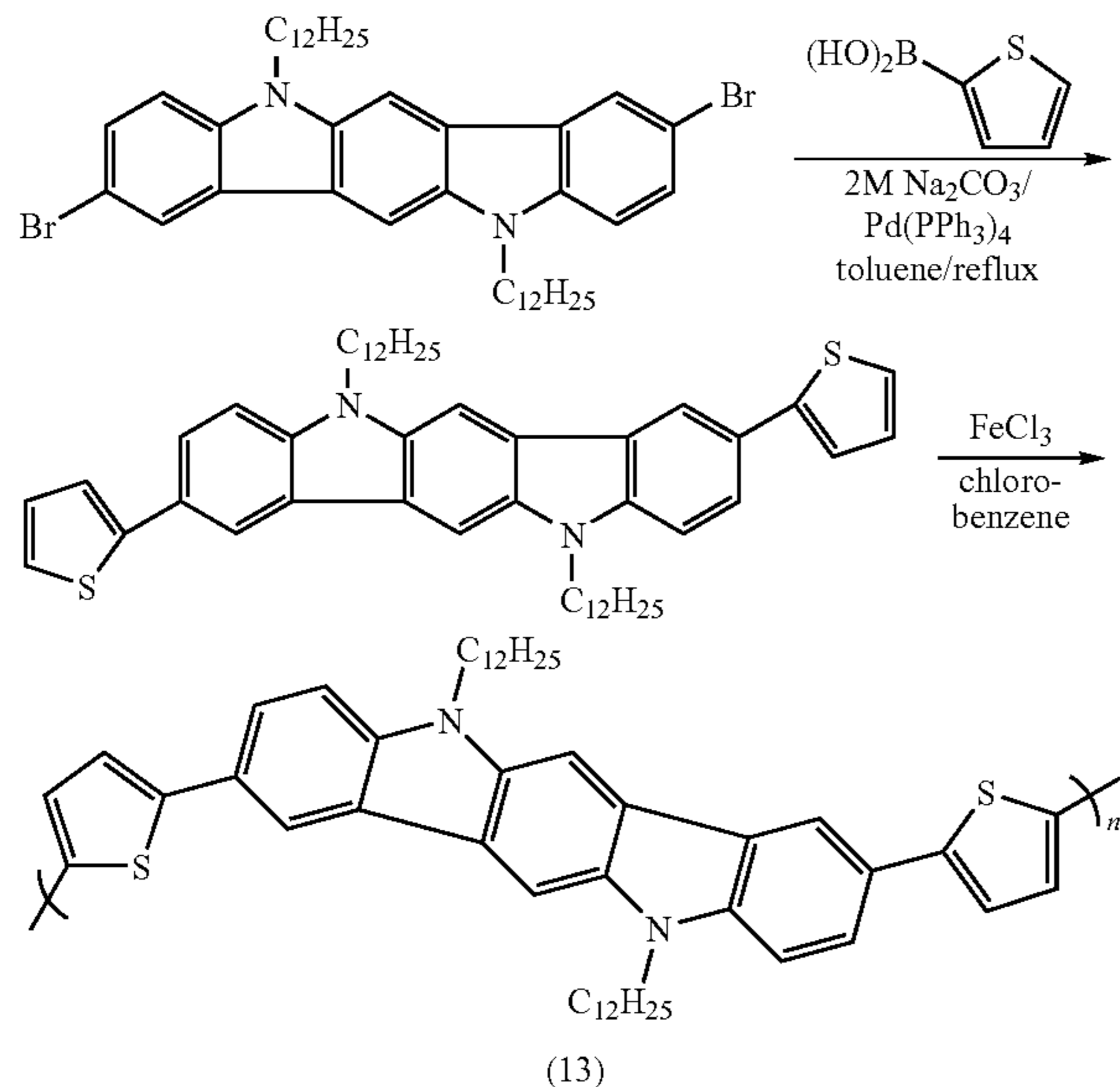
Scheme 3. Synthesis of polymer (13).
