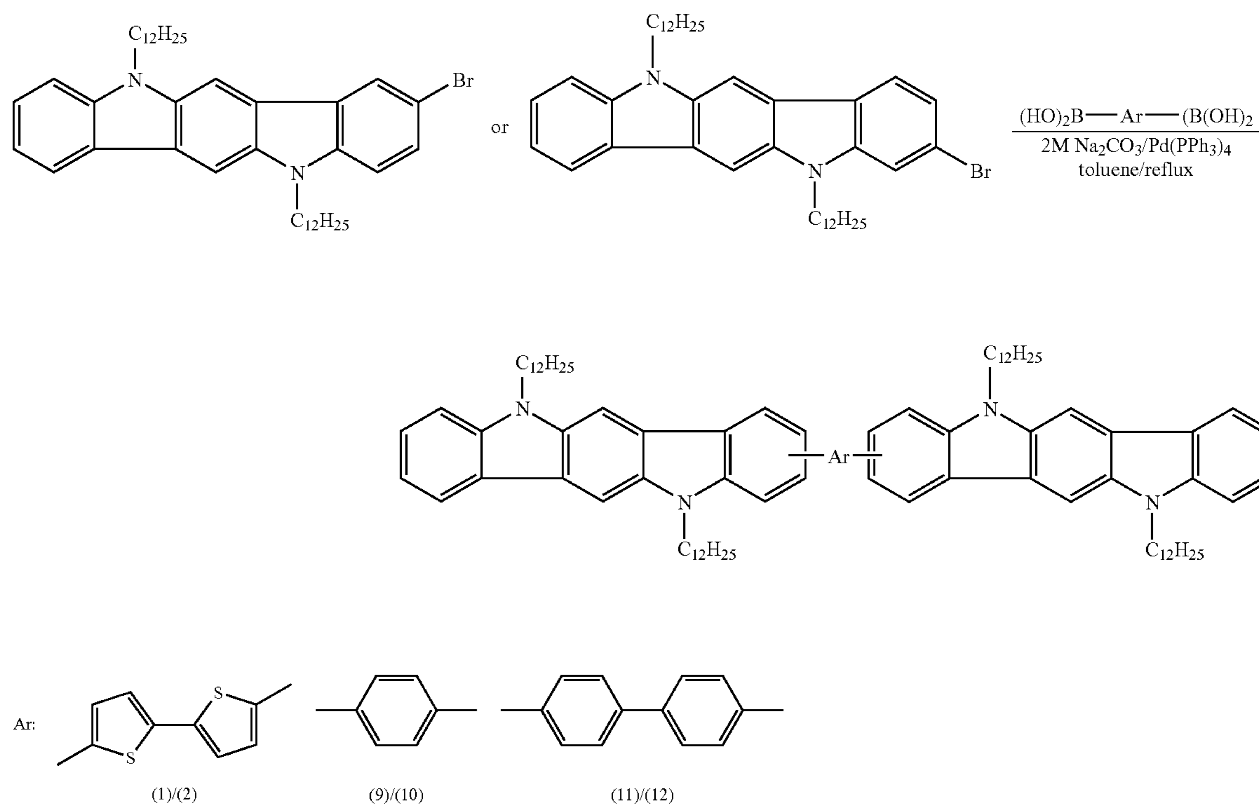
Scheme 1. Synthesis of Compound (1), (2), and (9) through (12).
