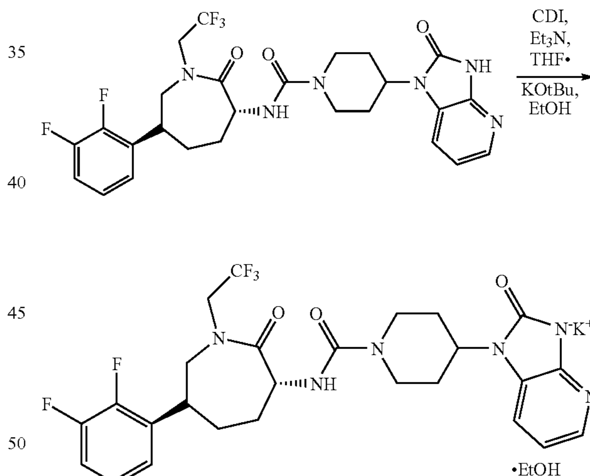
Scheme 1C
