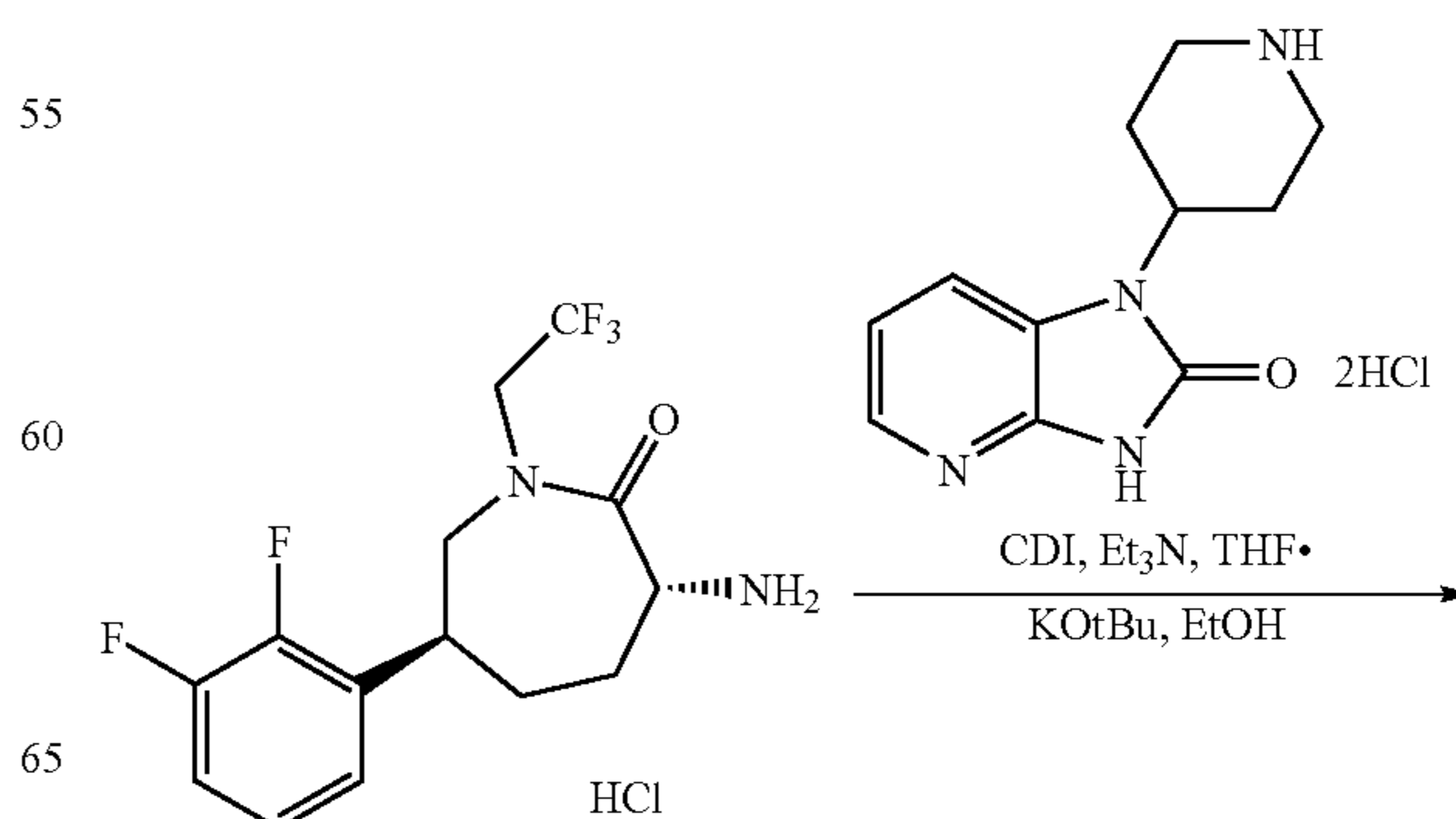
Scheme 1C
