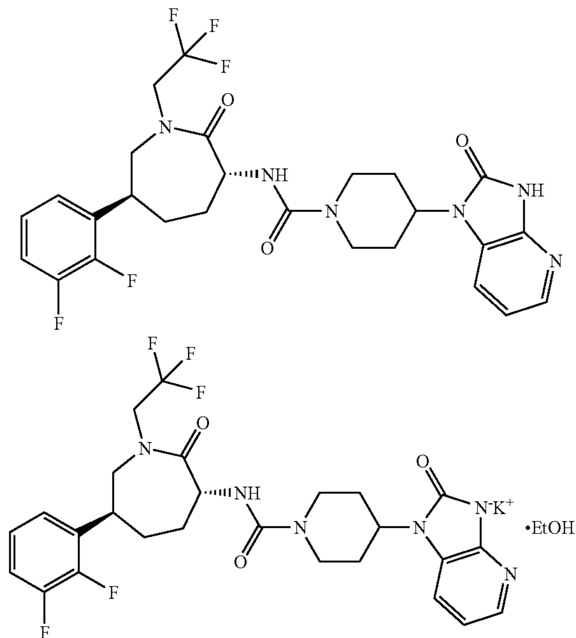
Scheme 1C
