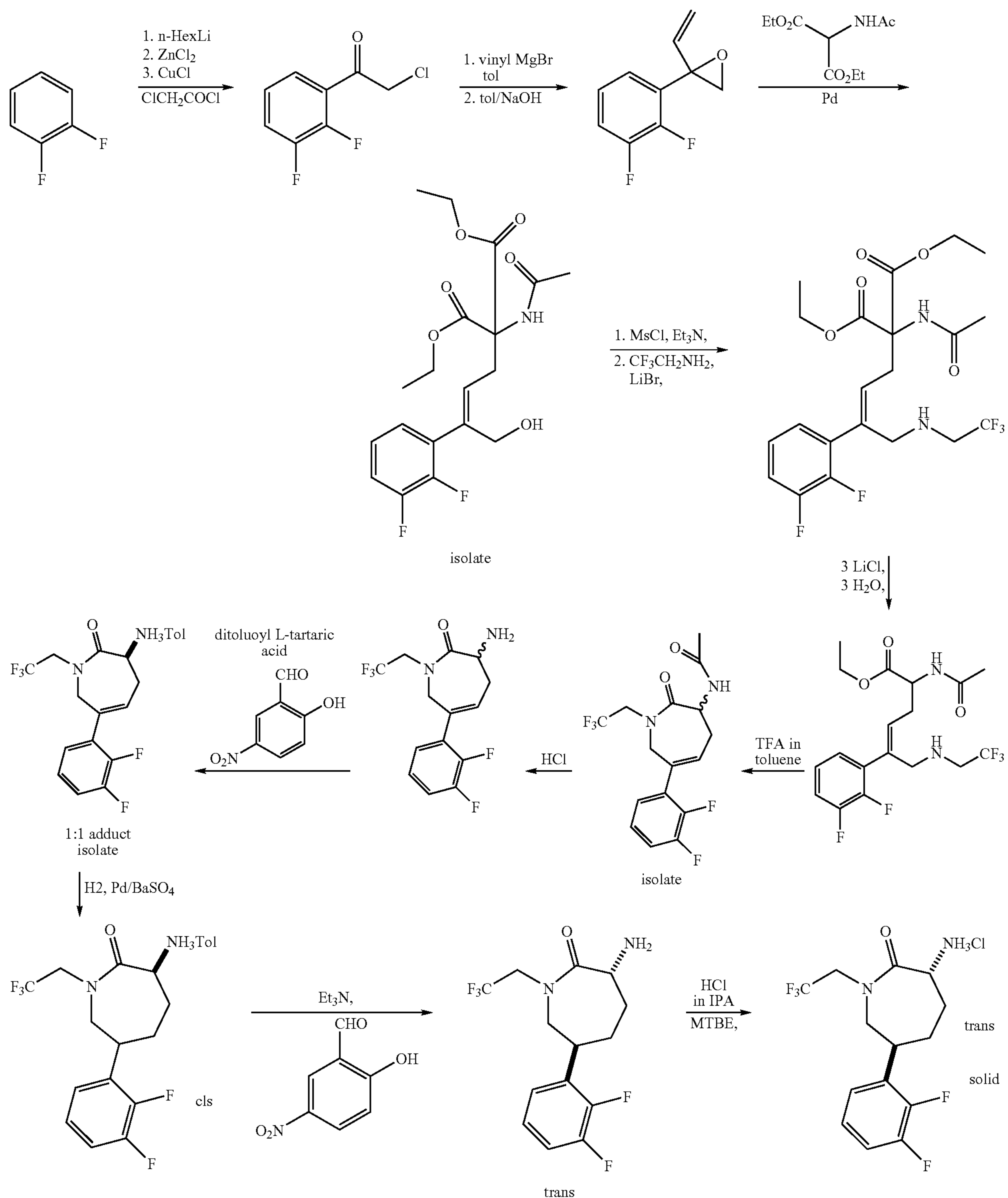
Scheme 2
