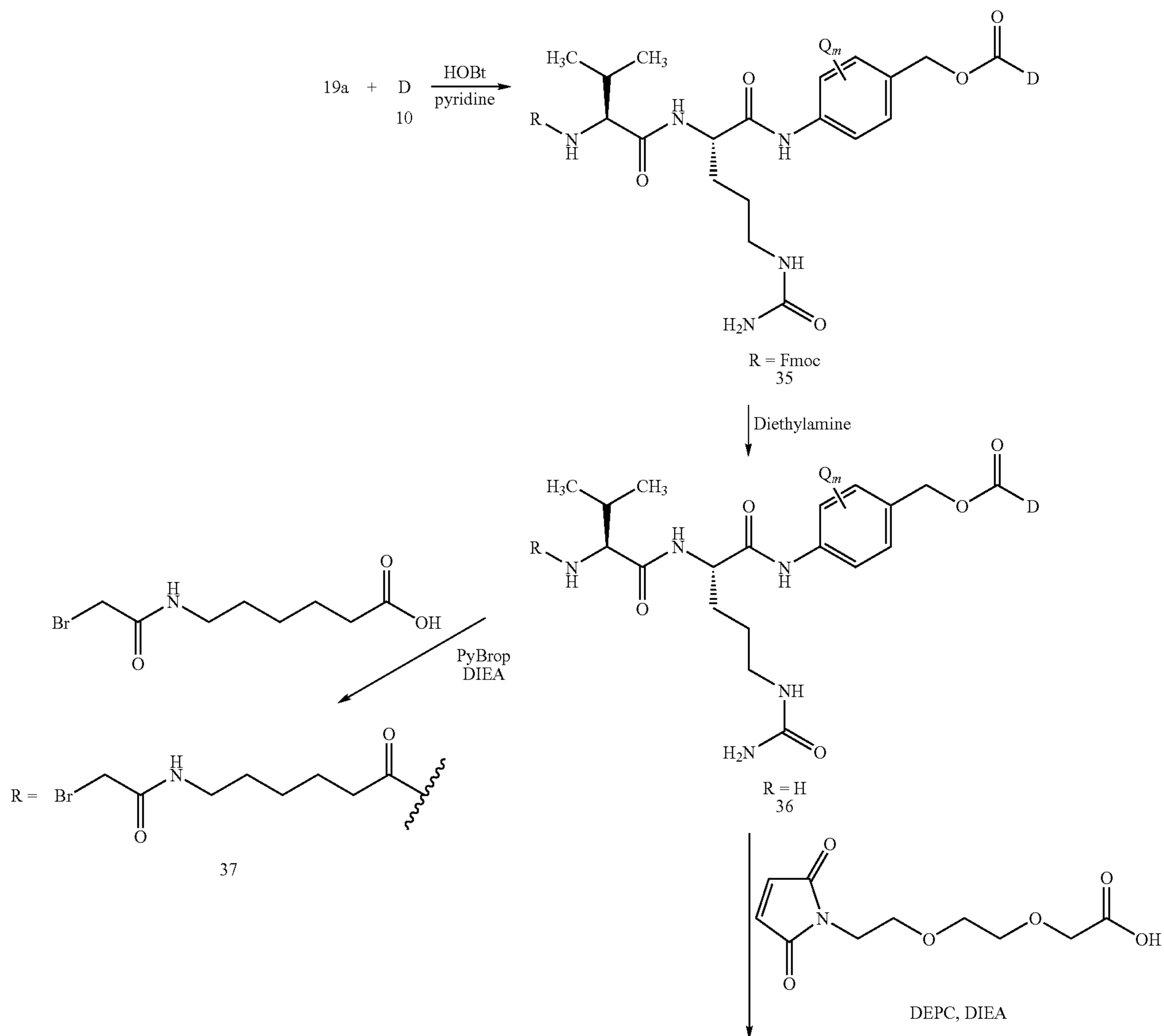
Scheme 14
