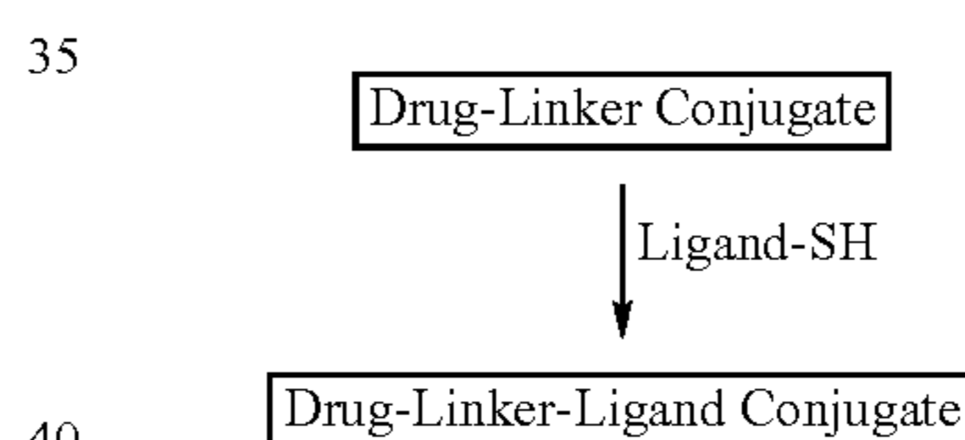
Scheme 17
