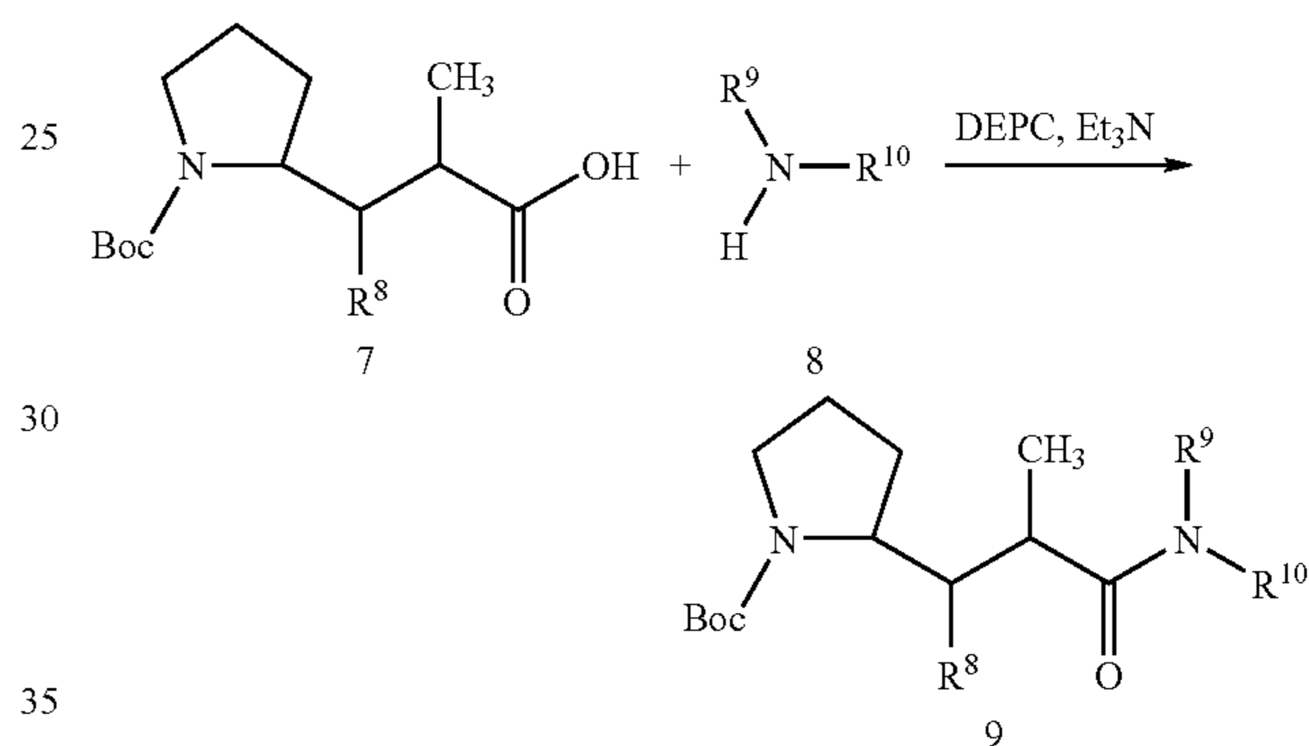
Scheme 6
