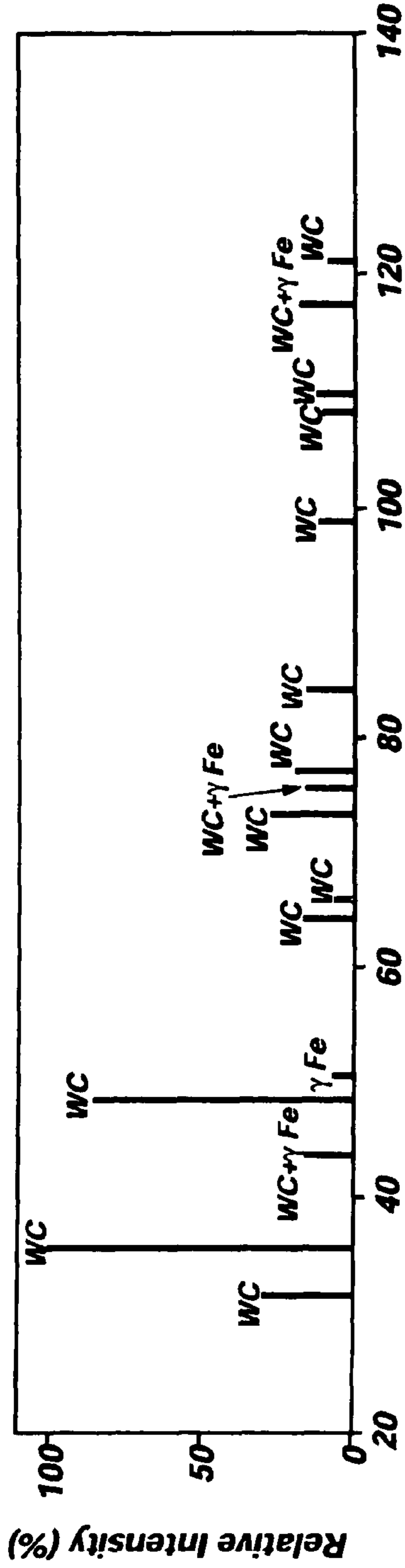
X-ray Diffraction Pattern Alloy "C" Carbide as ROCed
