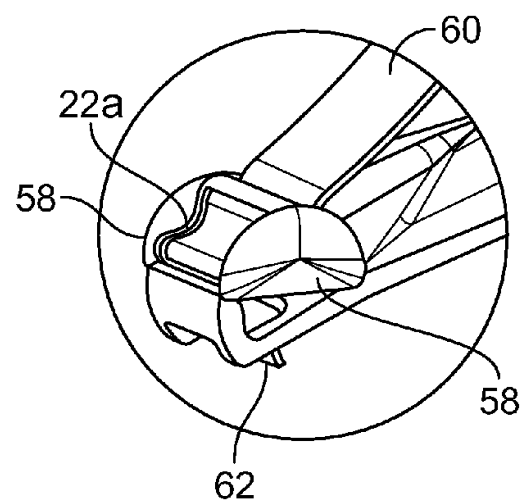
FIG. 3D
