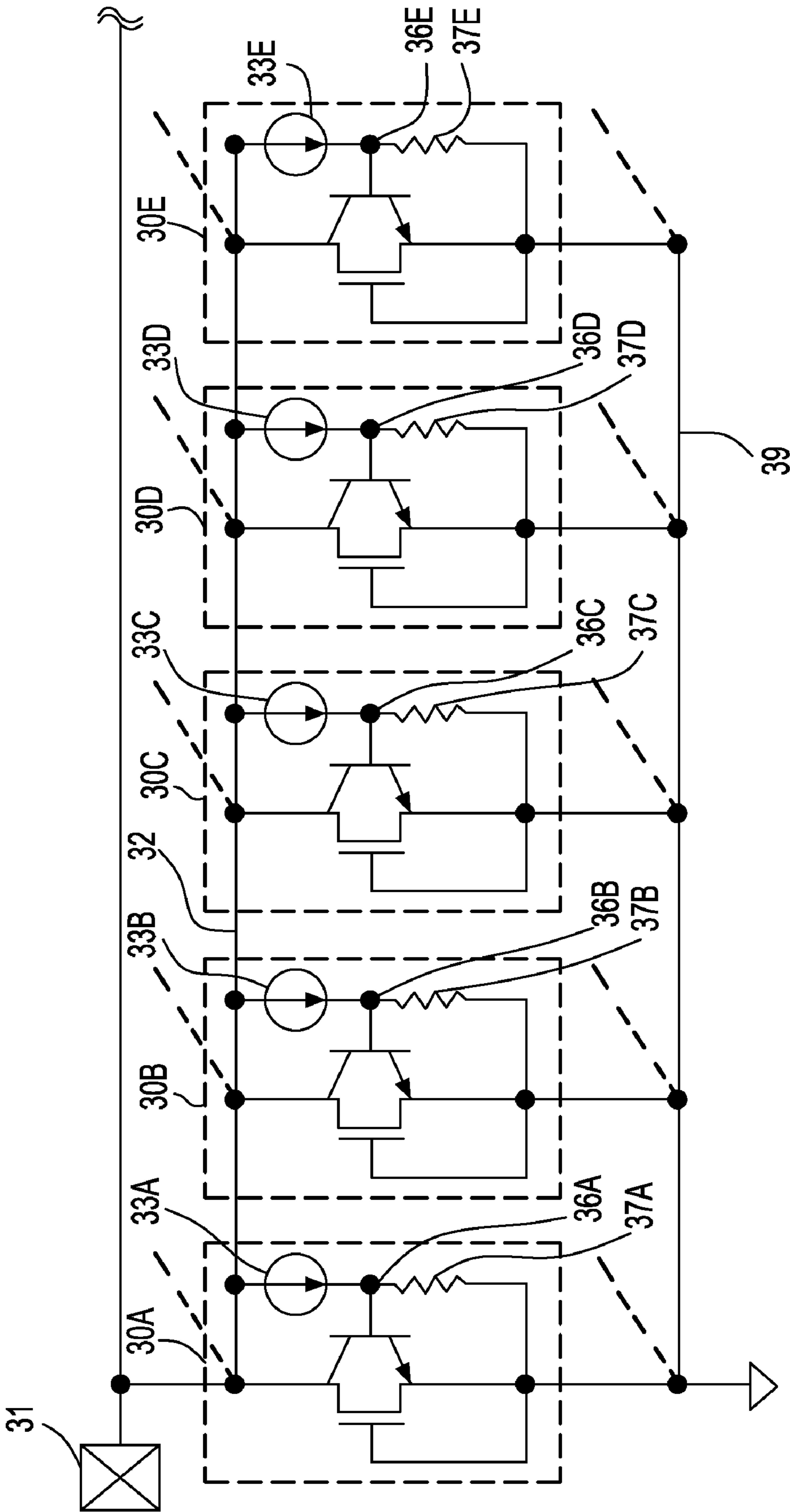
FIG. 3 (PRIOR ART)
