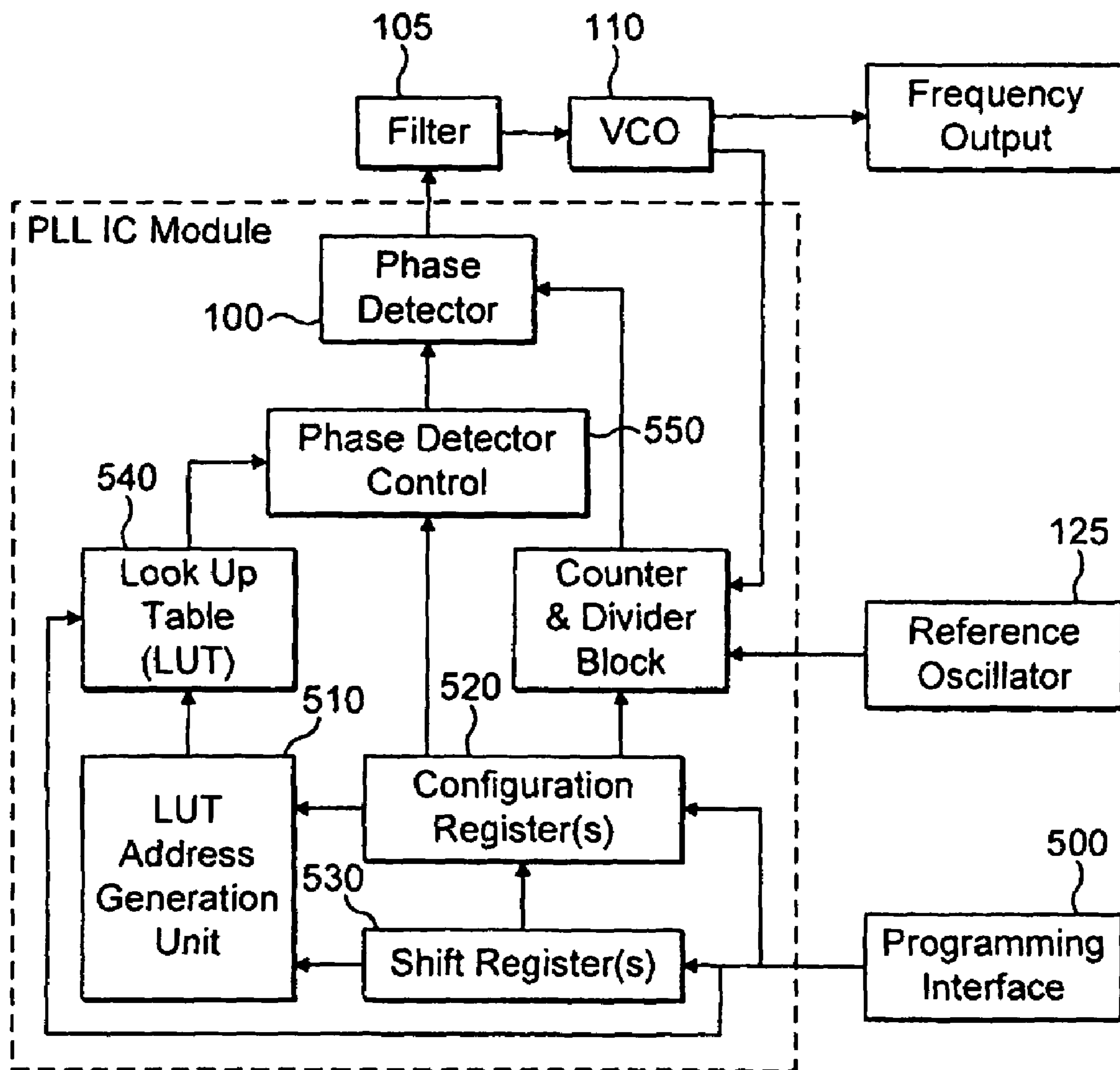
Look Up Table Implementation
